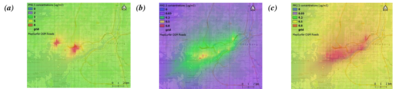
Figure 10: -Modelled annual mean PM 2.5 concentrations ( \mu\text{g m}^{-3} ) and contributions of shipping to the annual mean concentrations in year 2012: (a) Modelled annual mean concentrations in Base model simulation; (b) Modelled annual mean contribution of local shipping; (c) Modelled annual mean contributions of local and regional shipping. Base map credits: © OpenStreetMap contributors (openstreetmap.org). Distributed under a Creative Commons BY-SA License.
