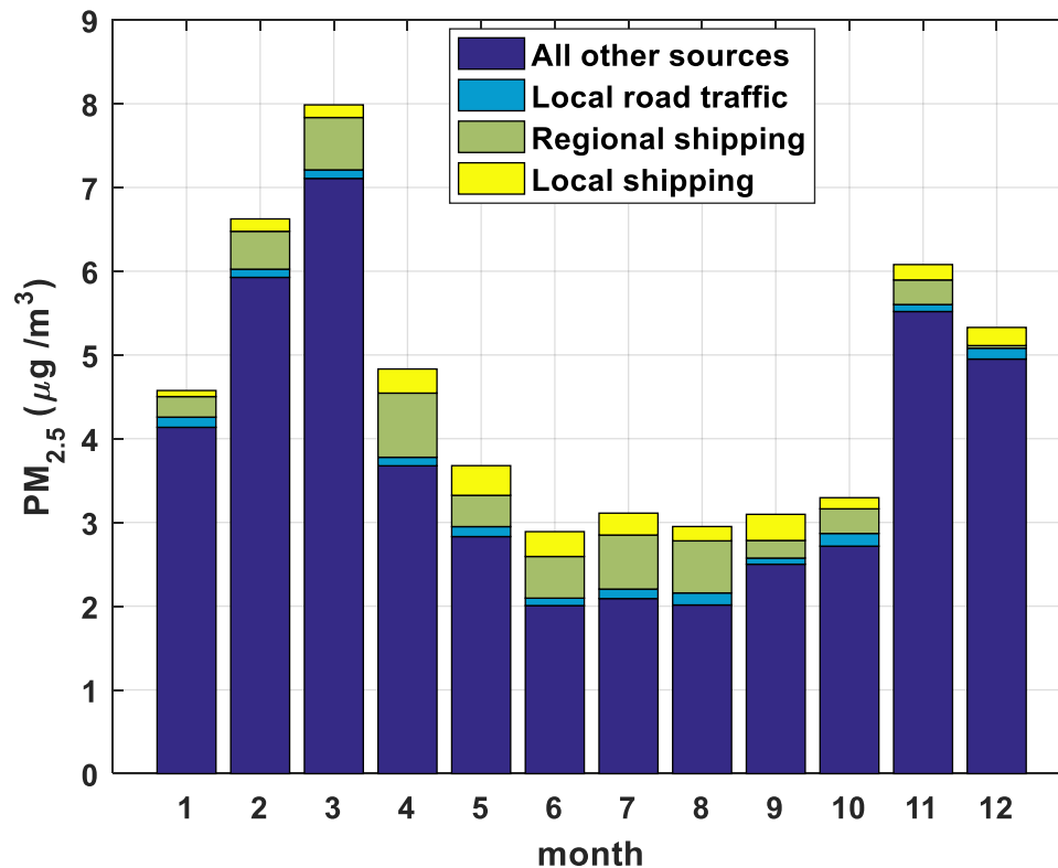
Figure 11: Modelled monthly mean contributions from local shipping, regional shipping and other sources (including contribution from the boundary condition) to PM_{2.5} concentrations ( \mu g m^{-3} ) at Eriksberg for year 2012.
