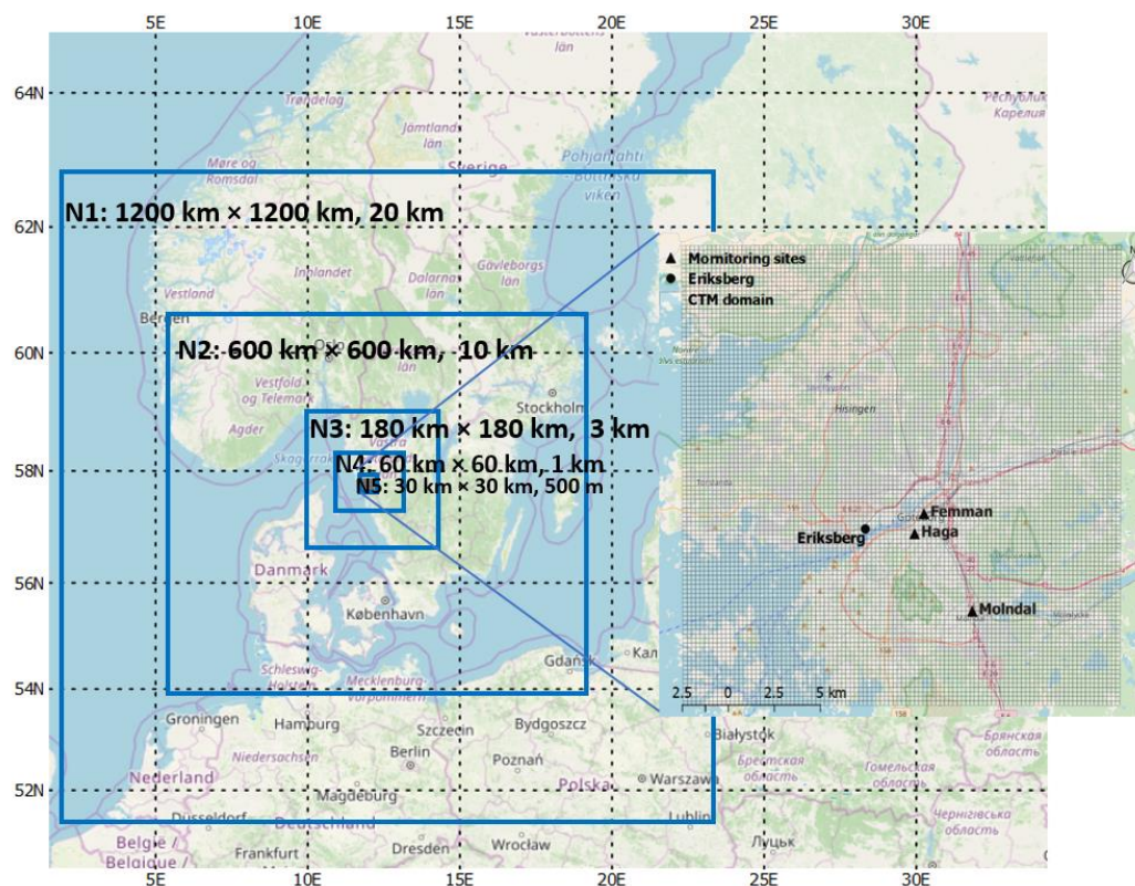
Figure 3: (a) Five nested meteorological model domains with their sizes and spatial resolutions. The fifth domain with air pollution grid (250 x 250 m 2 ) is pointed out in the figure, showing location of the three air quality monitoring sites Femman, Haga and Mölndal, as well as Eriksberg, a residential area close to the harbour;
