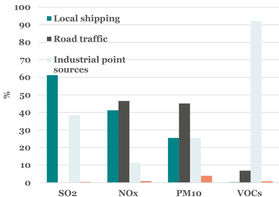
Figure 2: Proportion 3: Proportions of different source categories to in the local emission inventory for the city-scale model domain in year 2012. The total emissions were are 502 ton/tons year -1 for SO 2 , 5072 ton/tons year -1 for NO x , 357 ton/tons year -1 for PM 10 and 7457 ton/tons year -1 for VOCs.
