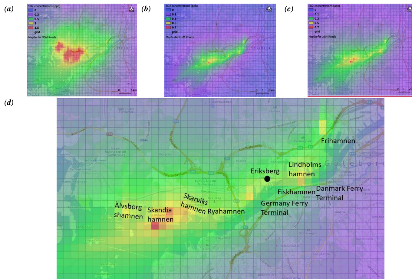
Figure 6: Simulated atmospheric concentrations of \text{SO}_2 (in ppb) for year 2012: (a) Annual mean concentrations in Base case simulation; (b) Annual mean contribution of the local shipping; (c) Annual mean contribution of the local and the regional shipping; and (d) Same as (c) with main ports along the Göta älv as well as Eriksberg. Base map credits: © OpenStreetMap contributors (openstreetmap.org). Distributed under a Creative Commons BY-SA License.
