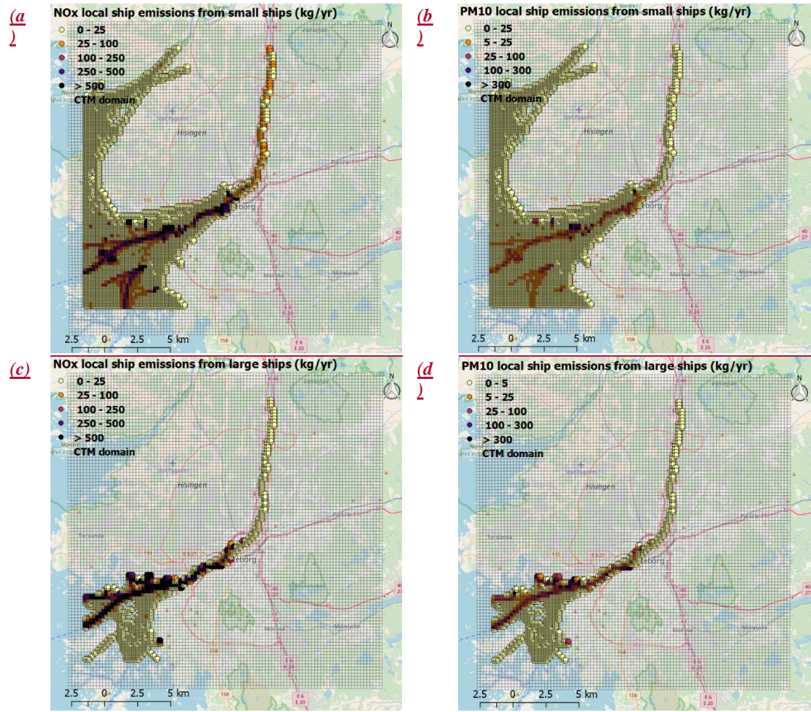
Figure 2: Annual local shipshipping emissions of (a) \text{NO}_x and (b) \text{PM}_{10} (equal to \text{PM}_{2.5} ) for from small vessels with stack height below 36 m (assumed 15 m) and (c) \text{NO}_x and (d) \text{PM}_{10} from large vessels with high stacks height above 36 m (assumed 36 m) in the Gothenburg area. Base map credits: © OpenStreetMap contributors (openstreetmap.org). Distributed under a Creative Commons BY-SA License.
