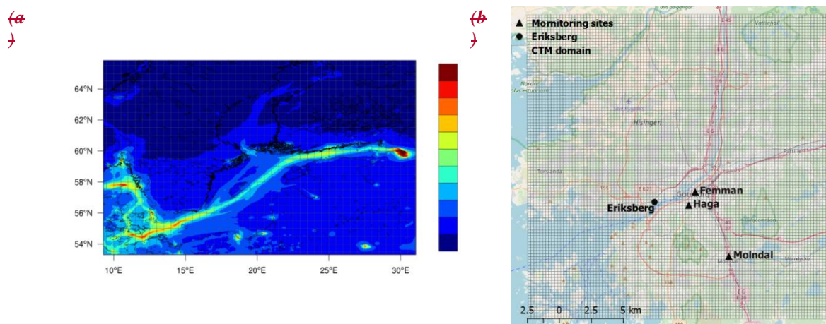
Figure 3: Summer mean (JJA) NO 2 atmospheric concentrations [ppbV] from the regional scale CMAQ simulation (4 × 4 km 2 ) for year 2012 (a) used for the boundary conditions in TAPM, and (b) the TAPM domain (250 × 250 m 2 ) with the three monitoring sites Femman, Haga and Mölndal used for validation of the urban-scale model simulations for Gothenburg. Eriksberg is the selected site which is close to the harbour and has high population density. Base map credits: © OpenStreetMap contributors (openstreetmap.org). Distributed under a Creative Commons BY-SA License
