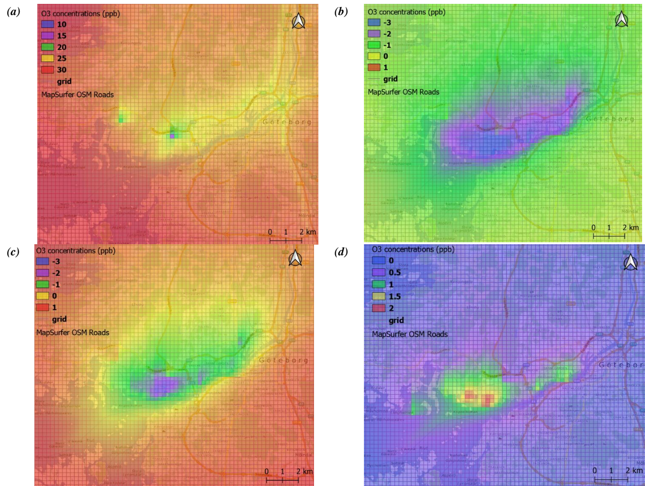
Figure 9: -Modelled summer mean (JJA) ozone concentrations (ppb) in year 2012 and contributions of local and regional shipping to the summer mean concentration in year 2012 : (a) Modelled O_3 concentrations in the Base model simulation; (b) Modelled contribution of emissions from local shipping; (c) Modelled contribution of emissions from local and regional shipping; (d) Modelled contributions of NMVOC emissions from local shipping. Base map credits: © OpenStreetMap contributors (openstreetmap.org). Distributed under a Creative Commons BY-SA License.
