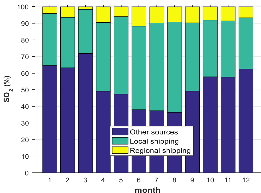
Figure S3: Modelled monthly mean relative contributions from local shipping, regional shipping and all other emission sources (road traffic, industry etc.) to \text{SO}_2 concentrations at Eriksberg in year 2012.
