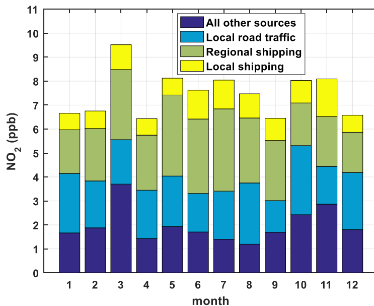
Figure 8: Time series of simulated Modelled monthly mean contributions of the local shipping and regional shipping, local road traffic and other anthropogenic emissions (including contribution from the boundary conditions) to the \text{NO}_2 daily mean concentrations at Eriksberg, located at the north of the Göta älv for the in year 2012. Modelled local shipping contributions (black line) deduced from the scenarios “Base” and “No local shipping”, regional shipping contributions (red line) deduced from the scenario “No local shipping” and “No local and no regional shipping”, and road traffic contributions (blue line) deduced from the scenario “Base” and “No road traffic” are presented.
