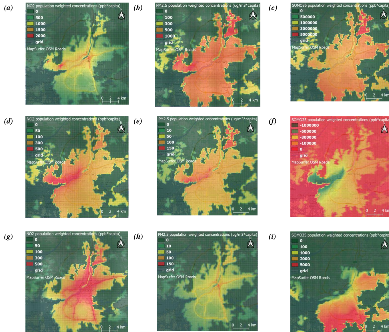
Figure 12: The population weighted annual mean concentrations for \text{NO}_2 ( \text{ppb} \times \text{capita} ), \text{PM}_{2.5} ( \mu\text{g m}^{-3} \times \text{capita} ) and \text{SOMO}_{35} ( \text{ppb} \times \text{h} \times \text{capita} ): (a) \text{NO}_2 in the Base simulation; (b) \text{PM}_{2.5} in the Base simulation; (c) \text{SOMO}_{35} in the Base simulation; (d) \text{NO}_2 from local and regional shipping; (e) \text{PM}_{2.5} from local and regional shipping; (f) \text{SOMO}_{35} from local and regional shipping; (g) \text{NO}_2 from road traffic; (h) \text{PM}_{2.5} from road traffic and (i) \text{SOMO}_{35} from road traffic. Base map credits: © OpenStreetMap contributors (openstreetmap.org). Distributed under a Creative Commons BY-SA License.
