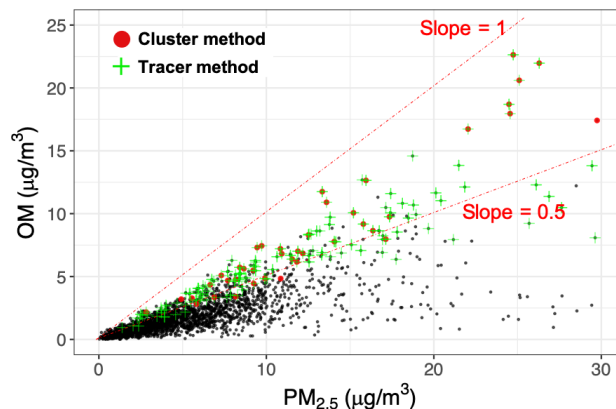
Figure 7. Scatter plot comparing total PM_{2.5} and OM mass in atmospheric samples. Red circles indicate residential wood burning and wildfire samples identified by cluster analysis (Bürki et al., 2020). Green crosses shows burning samples identified based on lignin and levoglucosan signatures. Black circles indicate the existing atmospheric samples in the IMPROVE network (2011 and 2013; approximately 3050 samples). The dotted dashed lines delineate the range of OM mass fraction for samples designated as burning-influenced (the slope of 0.5 is arbitrarily chosen to guide the eye). OM was estimated by multiplying OC by 1.8 (assuming an average OM:OC ratio of 1.8). Refer to Fig. S14 for more detailed classification.
