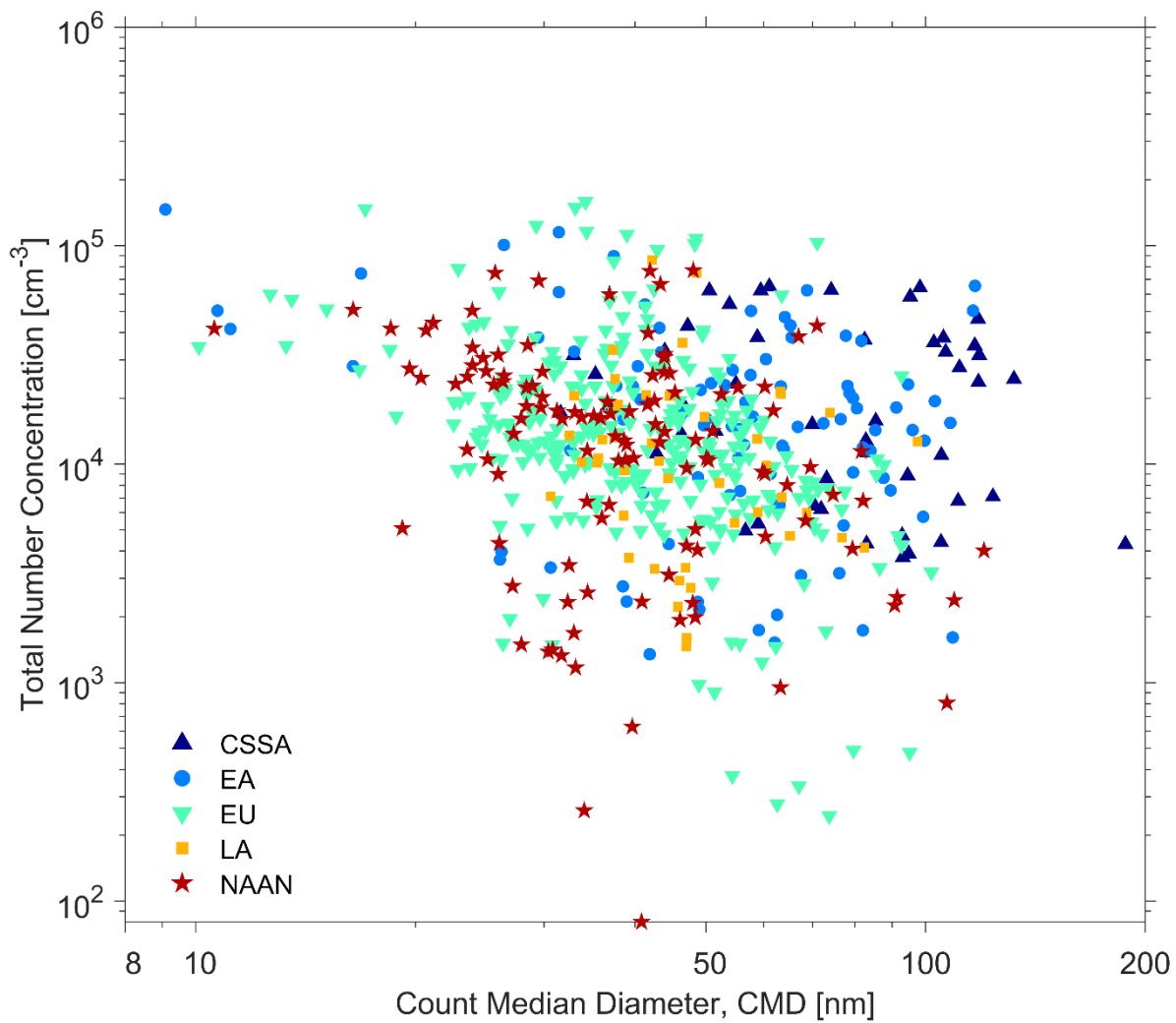
00 Figure 8. Relationship between the total particle number concentration, integrated over the measured size range, and the count median diameter (CMD), determined for each sub-micron number PSD measured by electrical mobility-based techniques (624 PSDs) and grouped by geographical region.
