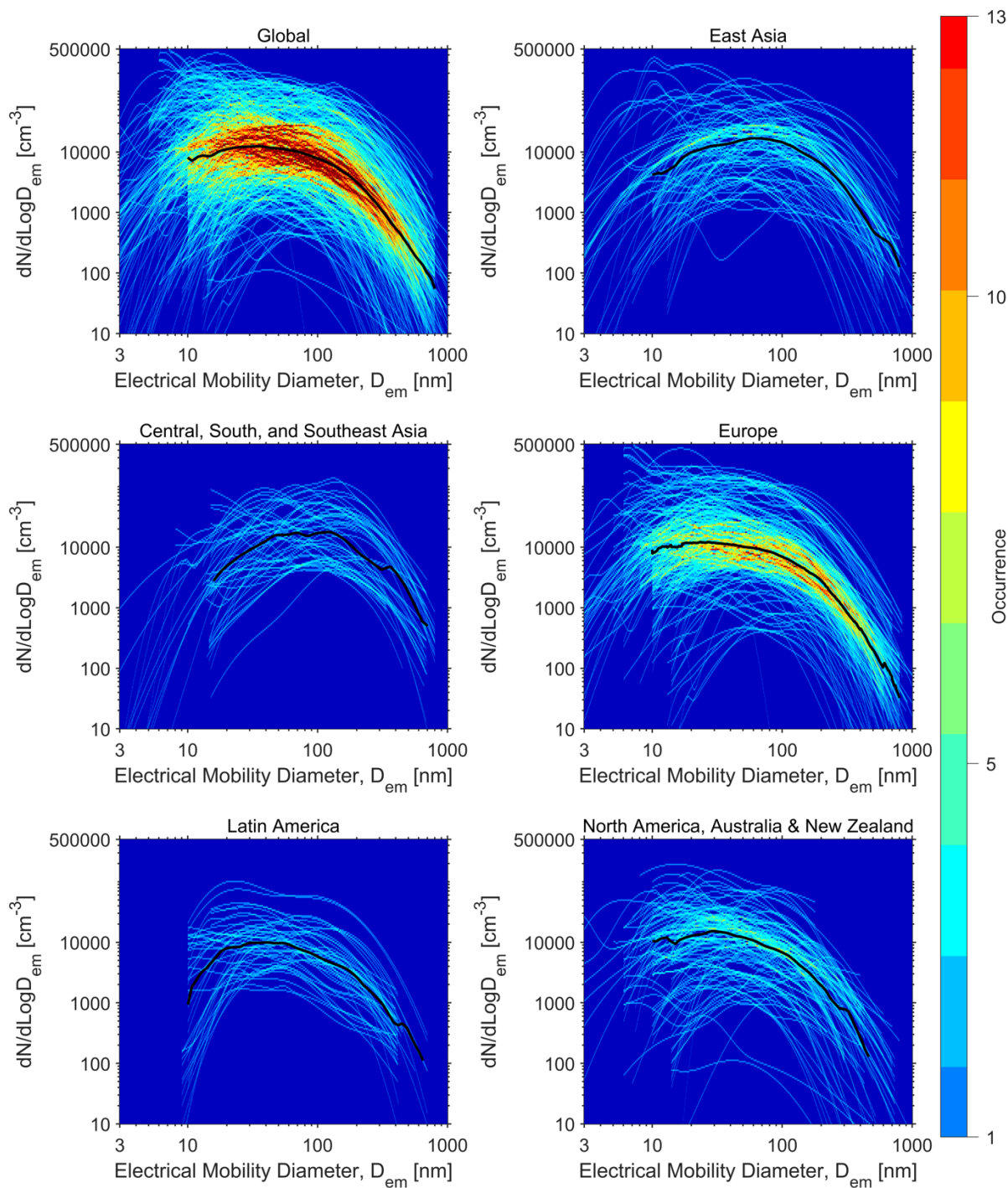
Figure 6. Urban aerosol number PSDs analyzed in this study, grouped by geographical region. The figure incorporates all sub-micron number PSDs measured by electrical mobility-based techniques (624 PSDs). The color represents the occurrence frequency of the number PSDs at a given particle size with a certain concentration. The black lines indicate the median number PSDs in each group.
