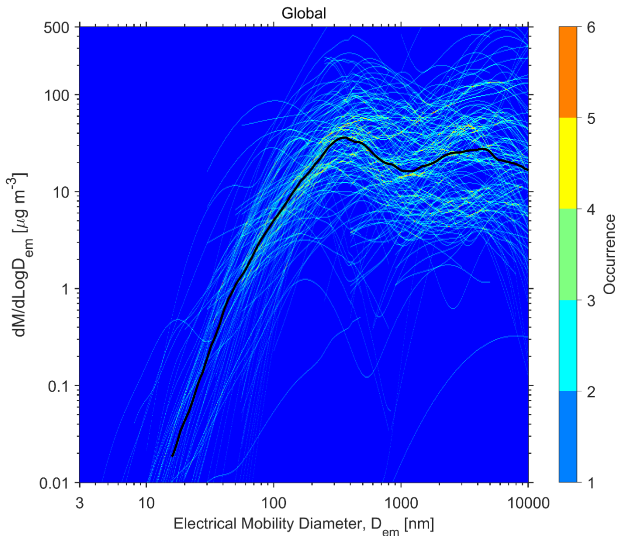
05 Figure 9. Urban aerosol mass PSDs analyzed in this study from around the globe (122 PSDs). The figure incorporates mass PSDs measured by gravimetric methods with inertial impactors and measurements made with electrical mobility-based and aerodynamic-/optical-based techniques that cover both the sub-micron and coarse modes. The color represents the occurrence frequency of the mass PSDs at a given particle size with a certain concentration. The black line indicates the median mass PSD.
