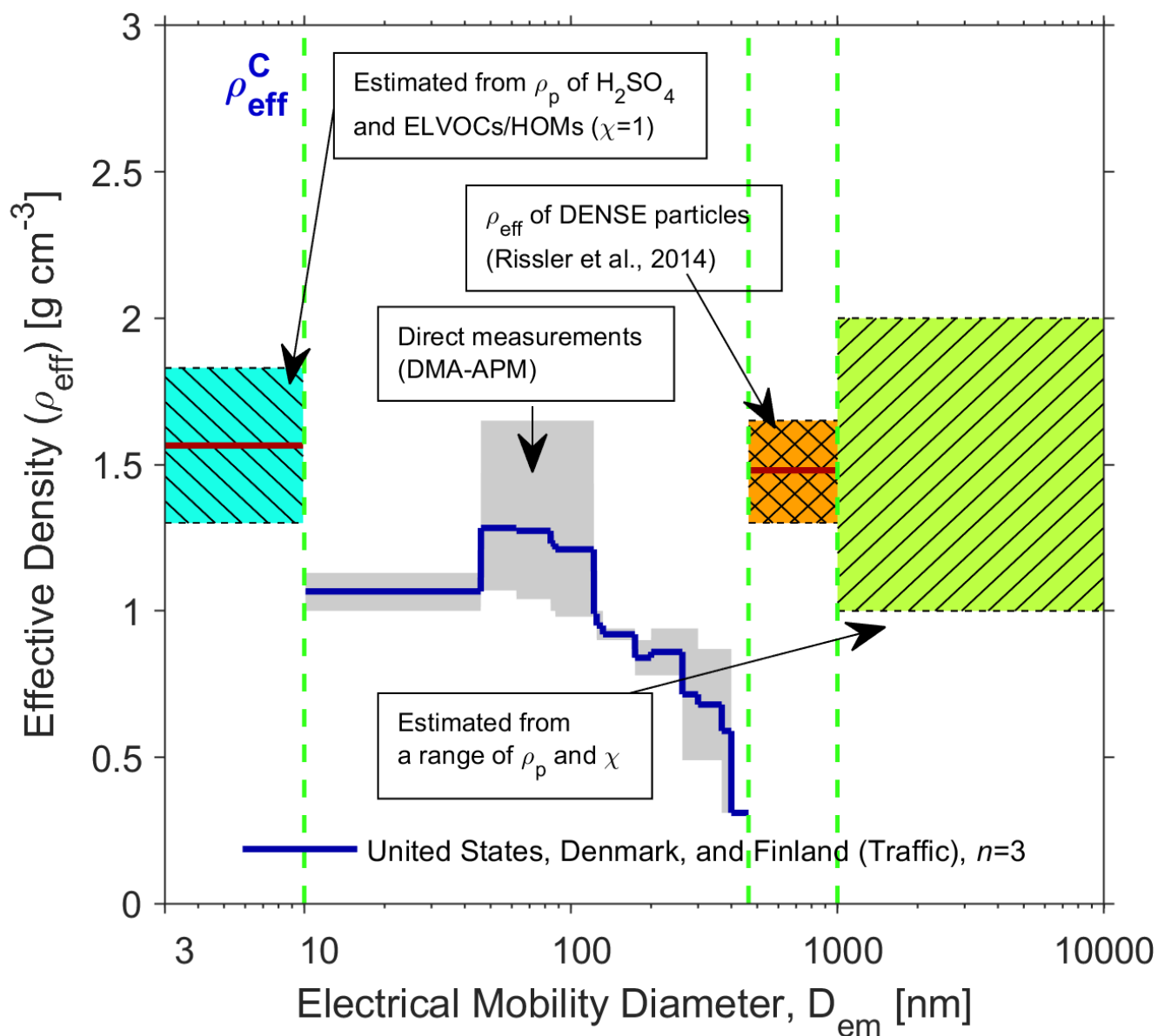
Figure 1. Size-resolved urban aerosol effective density functions ( \rho_{\text{eff}} ) for Group A ('urban'; obtained from measurements in China), Group B ('urban'; obtained from measurements in the United States), and Group C ('traffic'; obtained from measurements in the United States, Finland, and Denmark). Details of the \rho_{\text{eff}} measurements are summarized in Table S2. \rho_{\text{eff}} values for different combinations of \chi and \rho_p are illustrated in Fig. 2. Measurement technique nomenclature: DMA: Differential Mobility Analyzer, APM: Aerosol Particle Mass Analyzer, SMPS: Scanning Mobility Particle Sizer, APS: Aerodynamic Particle Sizer, MOUDI: Micro-Orifice Uniform Deposit Impactor.
