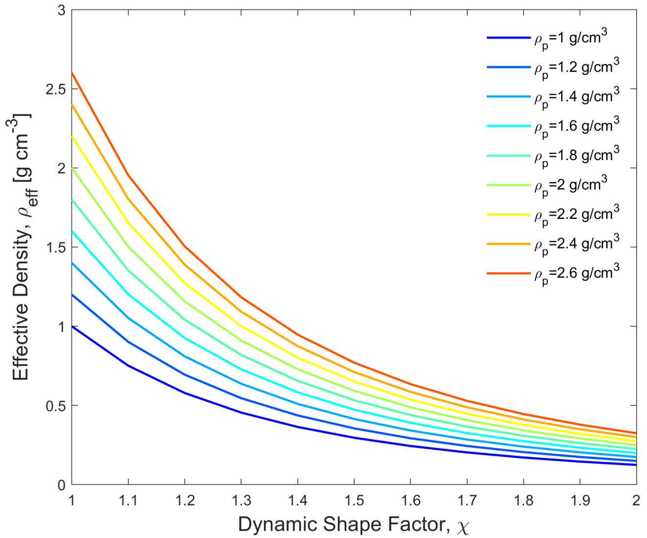
Figure 2. Effective densities ( \rho_{\text{eff}} ) as derived from different values of dynamic shape factors ( \chi ) and particle densities ( \rho_p ), assuming the value of \frac{c_c(D_{ve})}{c_c(D_{em})} is approximately unity for coarse particles.
