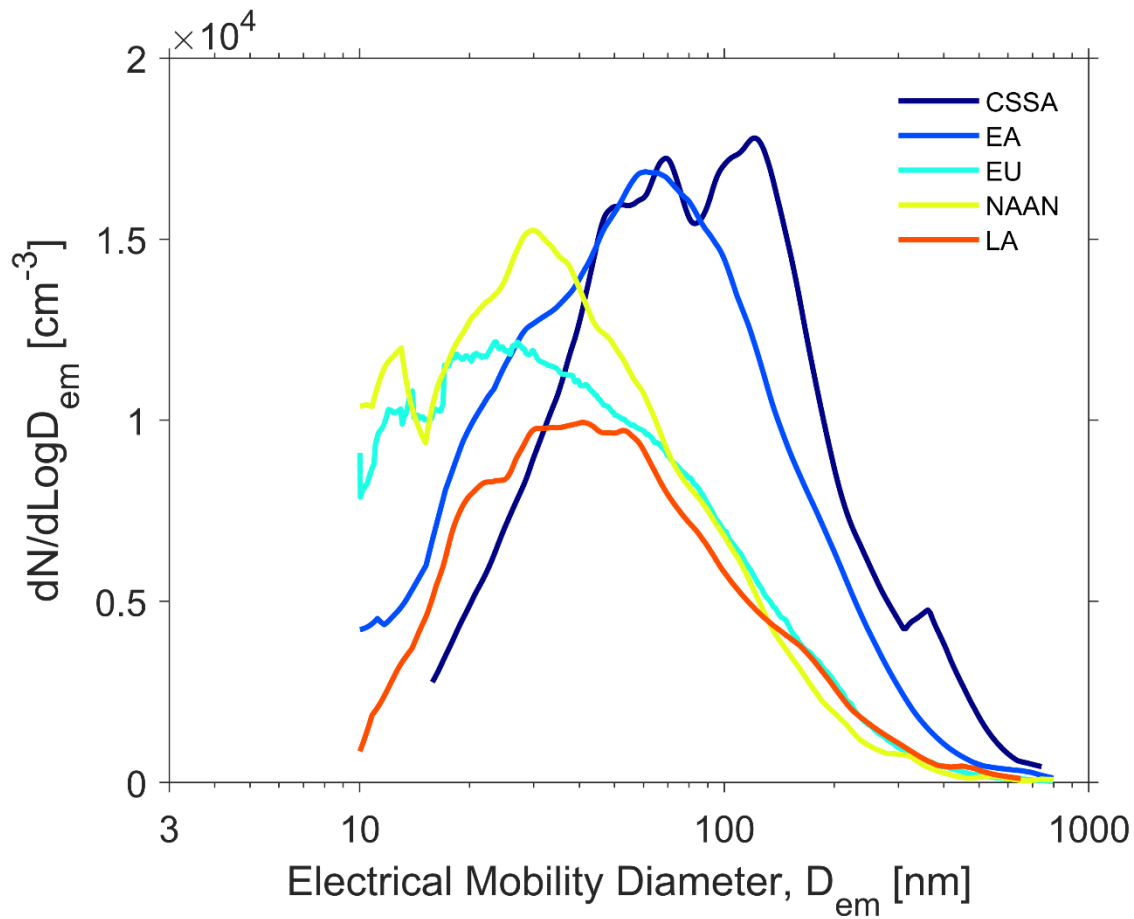
Figure 7. Median number PSDs for each geographical region.
