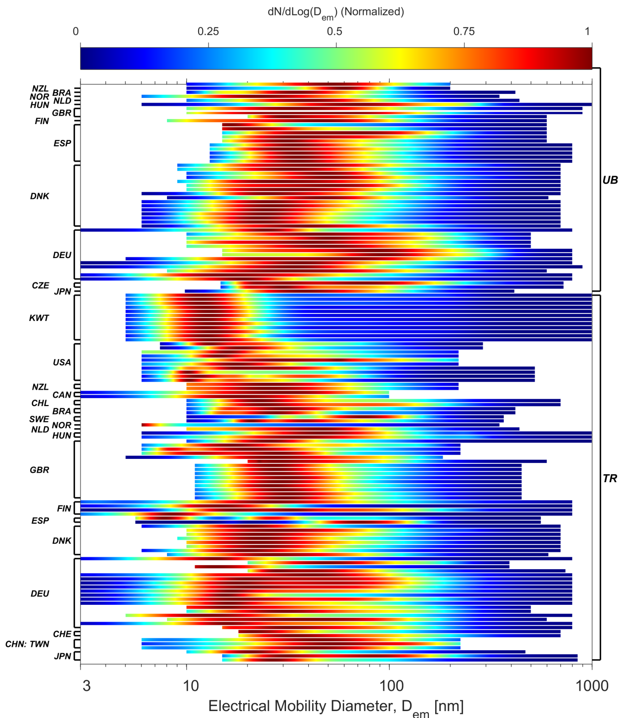
15 Figure 11. Comparison between normalized urban aerosol number PSDs measured at urban background (UB) and traffic-influenced (TR) sites. Only the number PSDs with a measurement period greater than one week are presented. The country codes are listed on the left and the site type is listed on the right.
