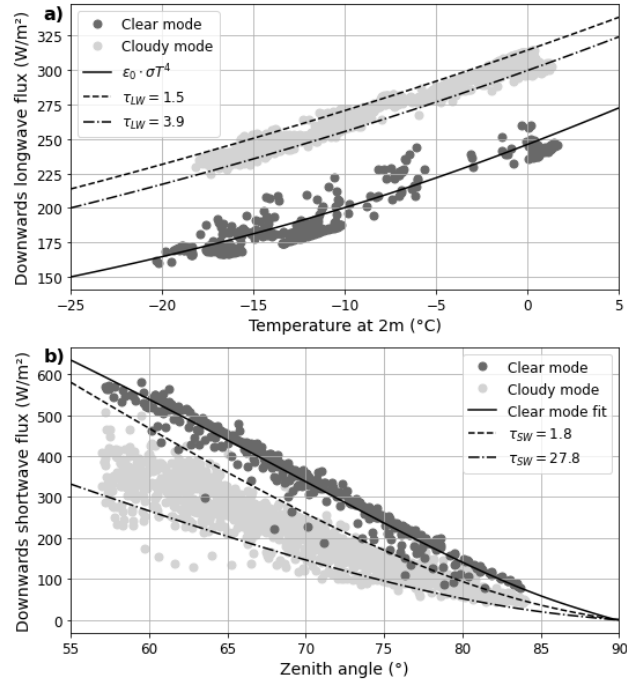
Figure 6. Panel a: longwave downwards radiative flux with near-surface (2 m) temperature as measured during the spring/summer period of the N-ICE field campaign. Dark grey points correspond to values for which \text{netLW} < -50 \text{ W m}^{-2} ("radiatively clear" mode) while for light grey points \text{netLW} > -20 \text{ W m}^{-2} ("opaquely cloudy" mode). The filled line correspond to the results of a simple parametrisation of LWd (Eq. (6)) in the absence of clouds, while the dashed lines represent the results of the parametrisation for \tau_{LW} = 1.5 and \tau_{LW} = 4.1 . Panel b: same, for shortwave downwards radiative flux vs solar zenith angle. The dashed lines are the results of Eq. (7) for \tau_{SW} = 1.7 and \tau_{SW} = 28.2 . For both panels, points are 30-minute averages of measurements.
