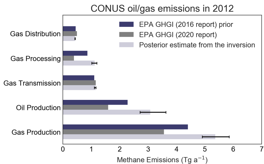
Figure 5. Methane emissions from the oil/gas sector in the contiguous US (CONUS) in 2012. The figure shows the original EPA GHGI estimates for 2012 used as prior in the inversion (EPA, 2016), the updated EPA GHGI estimates for 2012 based on revised methodology (EPA, 2020), and the posterior results from the inversion. Horizontal bars give the ranges of the inversion ensemble.
