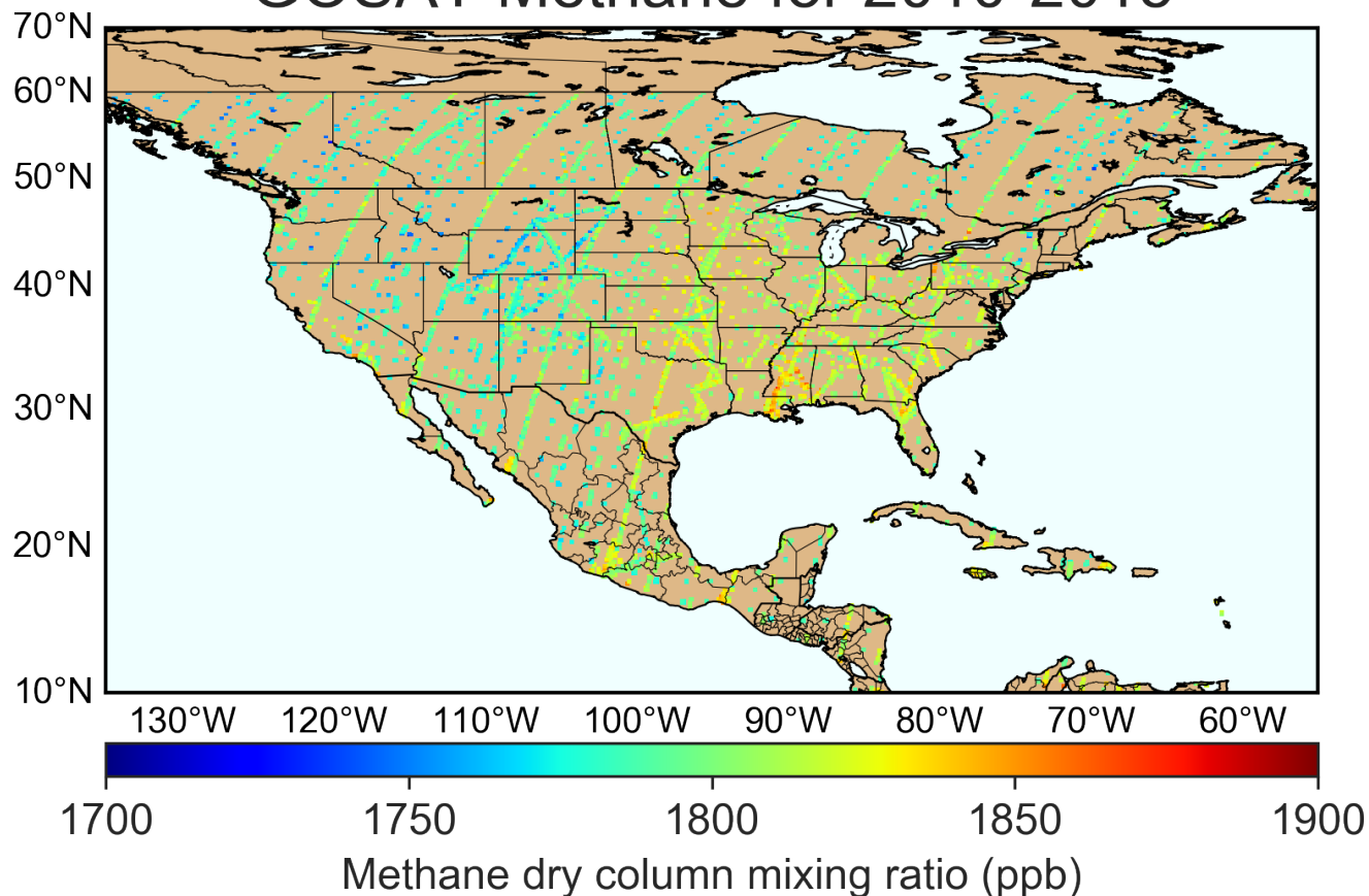
Figure 1. Average 2010-2015 methane dry column mixing ratios over North America observed by GOSAT. There are 156110 individual observations over land used in the inversion. The GOSAT data have 10km pixel resolution but we inflate them here to 0.3^{\circ} \times 0.3^{\circ} for visibility. GOSAT generally takes repeated observations of the same pixels so that most pixels shown here average a number of observations. The apparent north-south tracks that are GOSAT's default mode observations with a repeat cycle of 3 days, while the off-track data are target mode observations. GOSAT observations north of 60^{\circ}\text{N} are excluded because of their seasonal limitation and uncertainty about the stratospheric correction.
