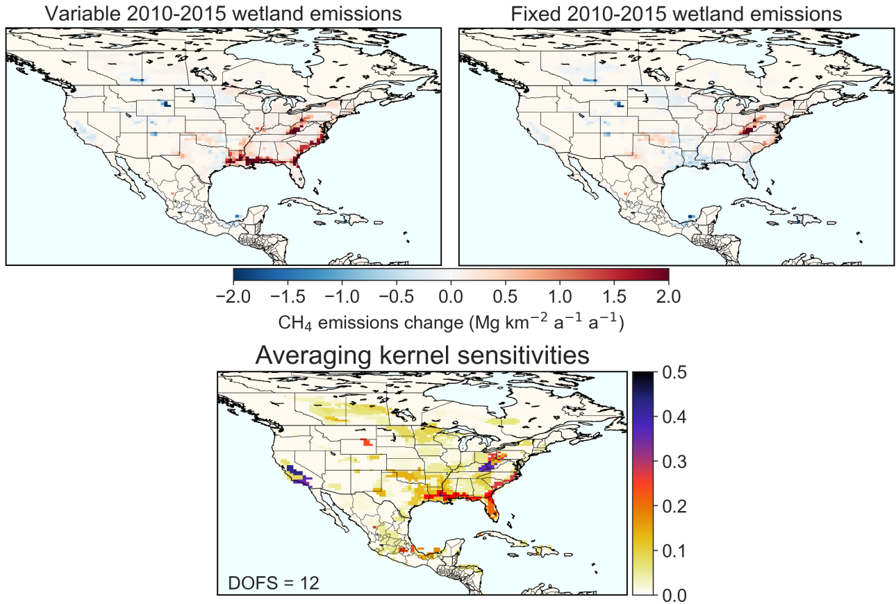
Figure 6. 2010-2015 methane emission trends in North America. The top panels show the posterior estimates from the inversion of GOSAT satellite data, allowing for 2010-2015 interannual variability in the prior estimates for wetlands and open fires (base inversion, left) and assuming constant not allowing for that prior estimates interannual variability (right). The results not allowing for 2010-2015 prior interannual variability of wetland and open fire emissions (right) are more reliable. The bottom figure shows the averaging kernel sensitivities, with the degrees of freedom for signal (DOFS) indicated inset.
