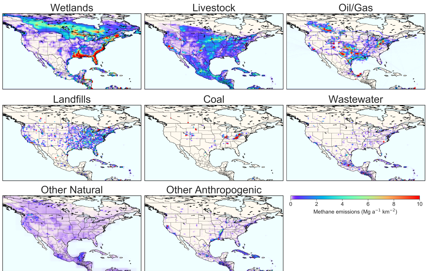
Figure 2. Methane emissions taken as Mean prior estimate estimates of methane emissions for 2010-2015. National totals, subsector breakdowns, and references are in Table 1.
