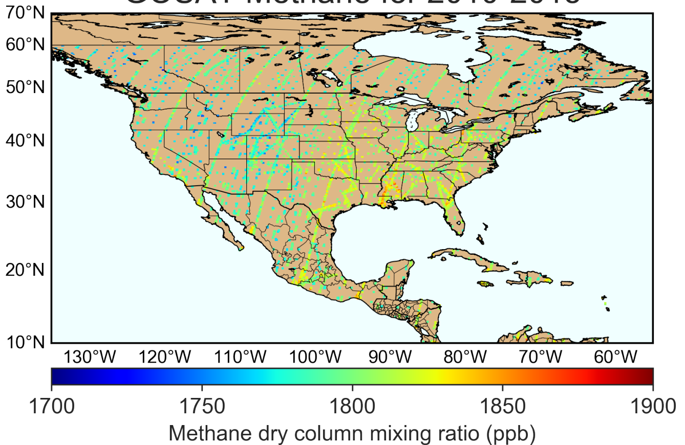
Figure 1. Average 2010-2015 methane dry column mixing ratios over North America observed by GOSAT. There are 156110 individual observations over land used in the inversion. The GOSAT data have 10km pixel resolution but we inflate them here to 0.3^{\circ} \times 0.3^{\circ} for visibility. GOSAT generally takes repeated observations of the same pixels so that most pixels shown here average a number of observations. The apparent north-south tracks that are GOSAT's default mode observations with a repeat cycle of 3 days, while the off-track data are target mode observations. GOSAT observations north of 60^{\circ}\text{N} are excluded because of their seasonal limitation and uncertainty about the stratospheric correction.
