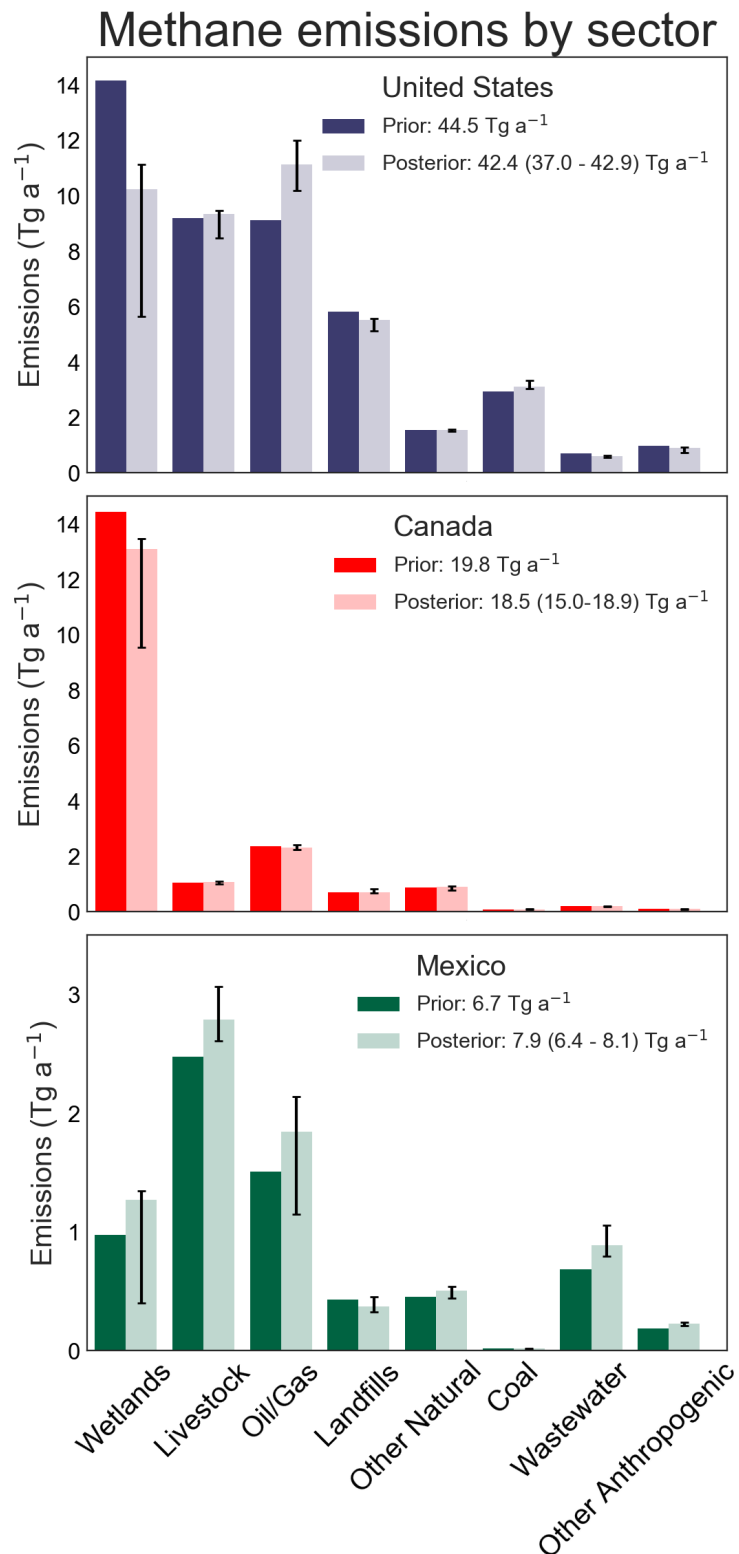
Figure 4. Mean 2010-2015 methane emissions per source sector for the contiguous US (CONUS), Canada, and Mexico. Values are shown for the prior estimates (Table 1) and for the posterior estimates from the after inversion of GOSAT data. Vertical bars show the ranges of results from the inversion ensemble.
