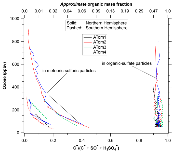
925 Figure 6. The organic content of two types of stratospheric particles using ozone as a surrogate for altitude. Shown are the relative areas of the C^+ peak in the mass spectra relative to two peaks indicative of sulfate. The top axis is an approximate mass fraction. The organic-sulfate particles are about 40 to 70% organic by mass, consistent with a tropospheric source. The sulfuric acid particles have near-zero organic content well into the stratosphere, increasing up to a few percent by mass near the tropopause. There was a strong difference in the organic content of the sulfuric acid particles between the hemispheres. Each point is the average of about 200 mass spectra.
