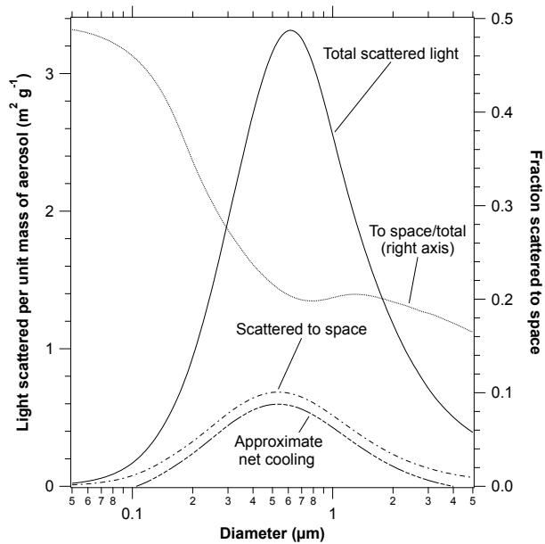
Figure 7. The mass scattering efficiency of particles with a refractive index similar to sulfuric acid. Shown are the total scattered light, the light scattered away from the Earth to space, and their ratio. Larger particles have more forward scattering and therefore a smaller fraction scattered to space. The lowest curve shows the climate impact after an approximate correction for warming due to infrared absorption. Particles smaller than about 0.1 \mu\text{m} or larger than about 4 \mu\text{m} warm the Earth (Lacis et al., 1992). Tropospheric particles containing ammonium sulfate or organic material with higher refractive indices would shift the curves to slightly larger diameters.
