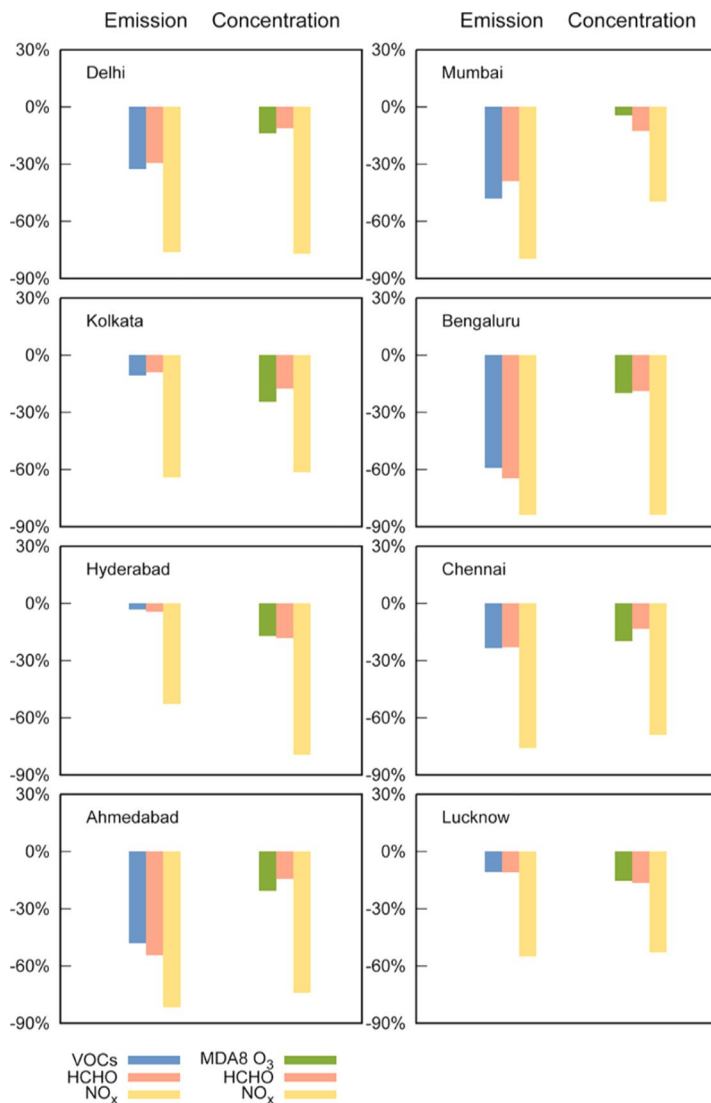
Figure 8: Predicted relative changes in concentrations of O_3 , HCHO, and NO_x and emissions of VOCs, HCHO, and NO_x in eight major cities of India in Case 2 to Case 1.
