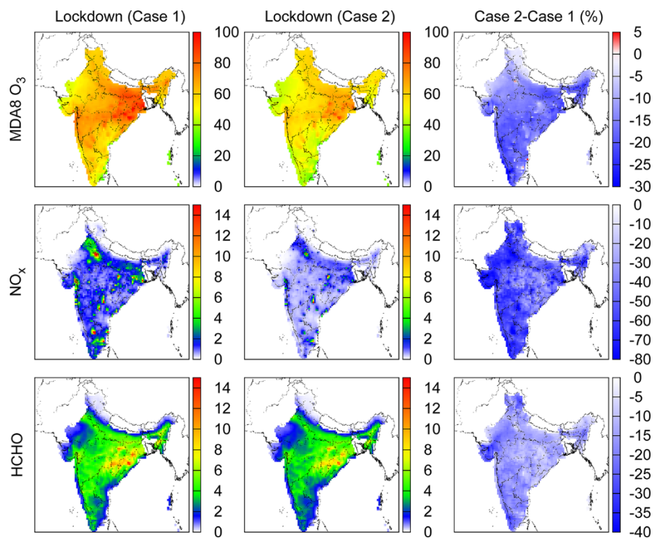
Figure 7: Predicted O 3 , NO x , HCHO, and the changes caused by nationwide lockdown measures from March 24 to April 24, 2020 in India. The unit is ppb. “Case2 - Case1” indicates (Case 2 – Case 1)/Case 1, reported as %.
