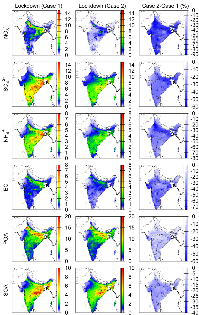
560 Figure 5: Predicted PM 2.5 components and the changes caused by lockdown measures from March 24 to April 24, 2020 in India. The unit is µg m -3 . “Case2 - Case1” indicates (Case 2 – Case 1)/Case 1, reported as %.
