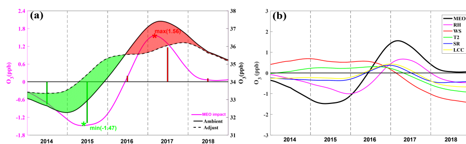
Fig. 1. (a) 5-year trends of ambient O 3 (solid black line), meteorological adjusted O 3 (dashed black line), and the meteorological impact (pink line) over the YRD during 2014–2018. Periods with positive and negative meteorological impacts are shaded in red and green, respectively; red and green bars represent the O 3 increases and decreases attributable to meteorological influences in each year. (b) 5-year variations in the meteorological impact of different meteorological factors (MEO), including relative humidity (RH), solar radiation (SR), air temperature (T2), wind speed (WS) and low cloud cover (LCC).
