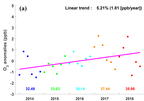
Fig. 5. (a) Anomalies of monthly average O 3 concentration from April to September during 2014–2018. The purple solid line represents the linear fitted curve, and the color number represents the annual (April–September) mean of O 3 concentration.
