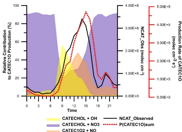
Figure 9. Diurnal variation in the relative contribution of the hydroxyphenoxy (CATEC1O) pathway to overall nitrocatechol formation. Also shown are the observed concentrations of nitrocatechol and the summed rates of CATEC1O production.
