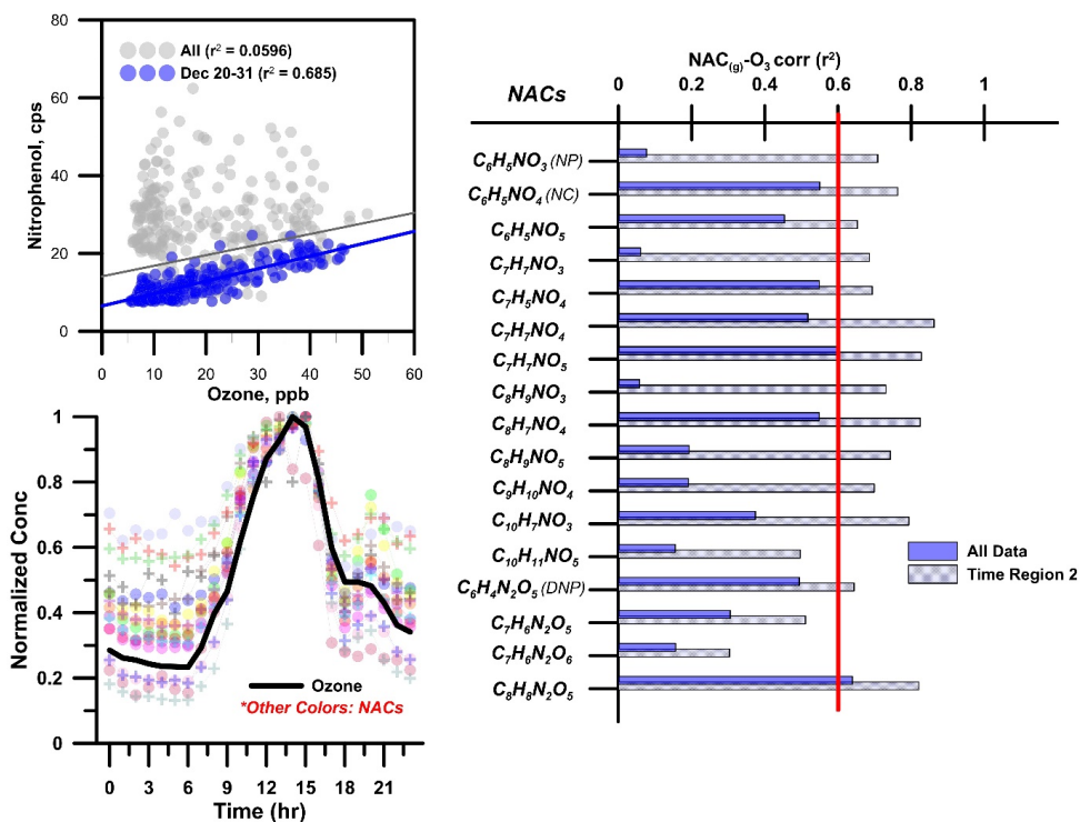
Figure 5 (Top left) Correlation between levels of nitrophenol and ozone ( O_3 ) (Bottom left) Normalized diurnal profiles of gas phase NACs and ozone under the second NAC formation regime observed during the field campaign (Right) Coefficients of determination ( r^2 ) between gas phase NACs and O_3 for the whole data set and for regime 2 only.
