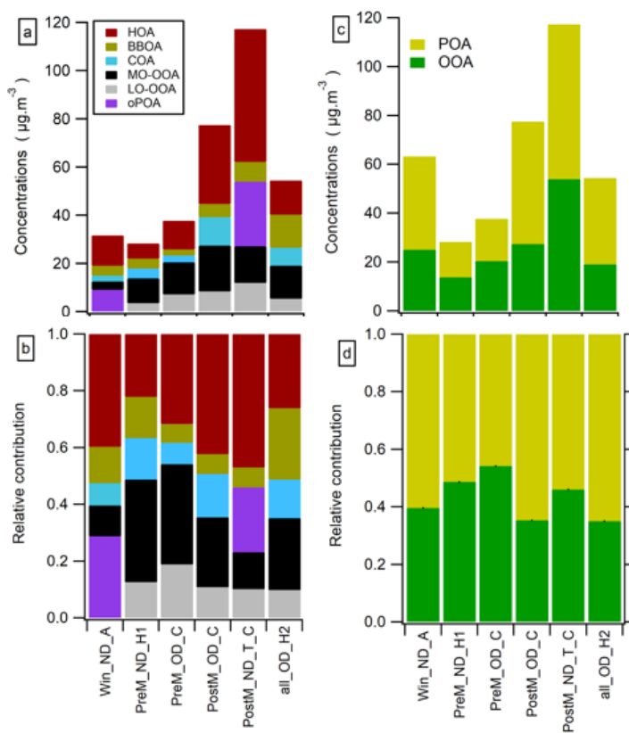
Figure 6. OA average concentrations (6.a) and relative contribution (6.b). The whiskers represent the standard deviation of POA/OOA contribution after running PMF with different F_{\text{peaks}} between -1 to 1 with steps of 0.2 to prove the stability of the separation.
