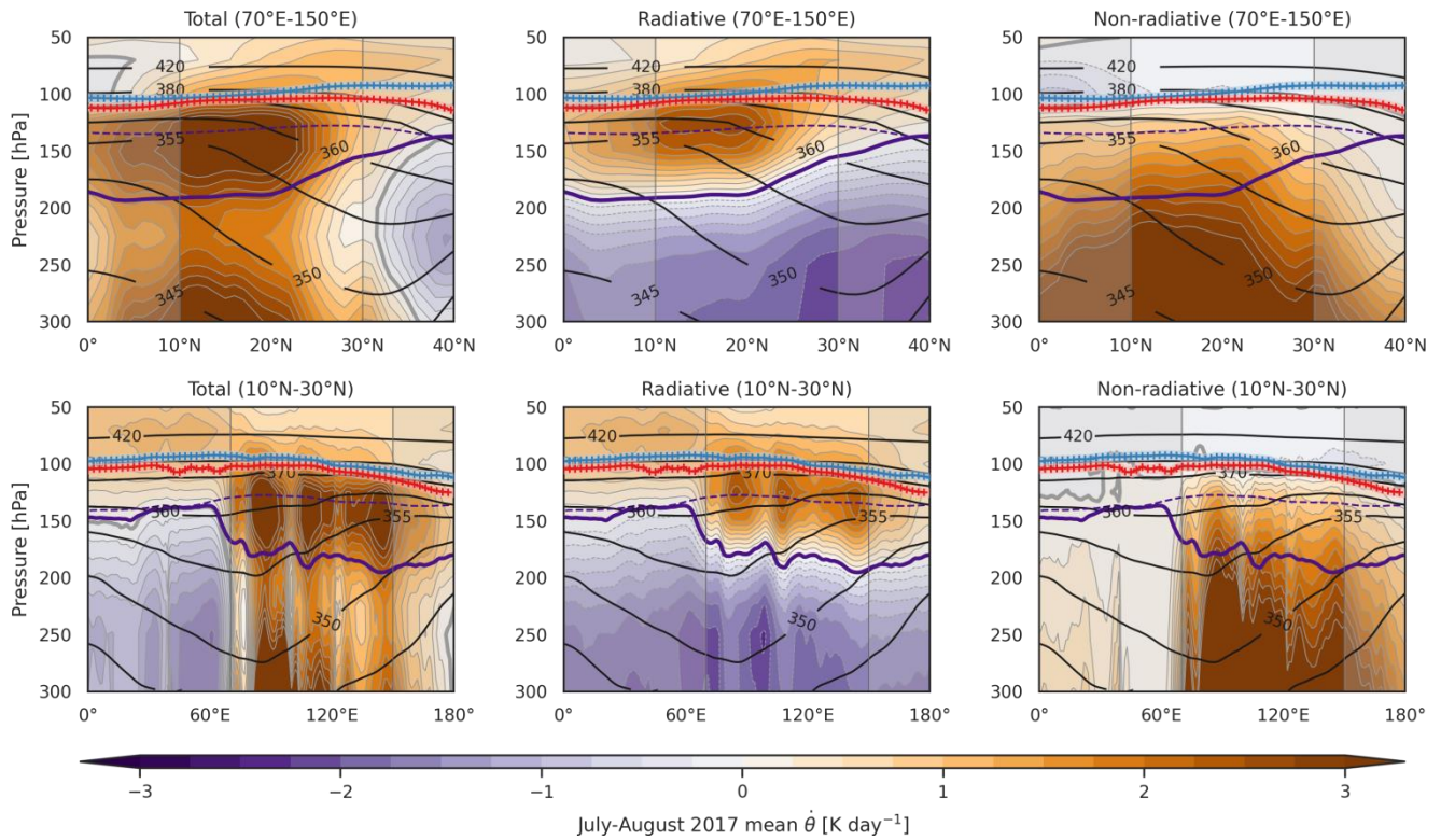
820 Figure 8 Zonally (top) and meridionally (bottom) averaged total (left), radiative (centre) and non-radiative (right) diabatic potential 825 temperature tendencies (d\theta/dt)_{diab} based on the ERA-Interim reanalysis for July-August 2017. As demarcated by the vertical grey lines and bolder colors on the respective panels, zonal averages are calculated over 70 – 150°E and meridional averages over 10 – 30°N with area weights applied. Black contours show potential temperature. Purple contours show the vertical location of the LZRH based on the zero contour in time-mean radiative heating rates under all-sky (solid) and clear-sky (dashed) conditions. LRT and CPT are shown in red and blue respectively. Averaging ranges for \theta contours, LZRH, LRT and CPT are the same as those for (d\theta/dt)_{diab} .
