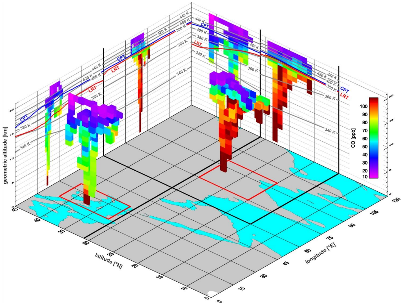
765 Figure 2 3D Map of averaged CO mixing ratios observed during all StratoClim flights (raw CO profiles for all individual flights are shown in supplementary Figure S1). Values in 3D space represent averages in 1^\circ \times 1^\circ \times 1 km longitude – latitude – altitude bins. Longitude-altitude averages over all latitudes and latitude-altitude averages over all longitudes are projected onto the x-z and y-z planes respectively. Grey contour lines in the x-z and y-z planes show potential temperature levels averaged meridionally and zonally over the areas marked on the map by the thick black lines; red and blue lines show LRT and CPT heights averaged over the same areas (based on ERA-Interim reanalysis products during the respective campaign phases).
