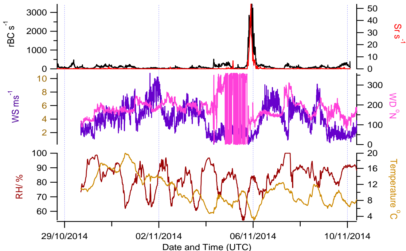
190 Figure 1: Meteorological measurements Relative humidity (RH), Temperature, Wind direction (WD) and Wind speed (WS) along with the time series of BC and Strontium (Sr), a firework tracer emitted during the bonfire night.
