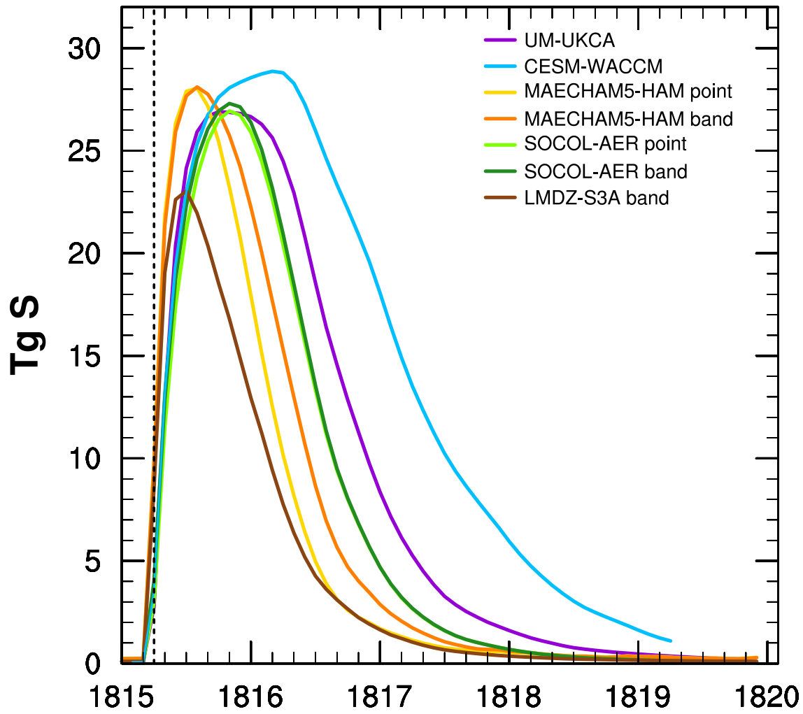
Figure 2: Global stratospheric burden of SO 4 in TgS vs time. Vertical dashed black line indicates month of injection.
