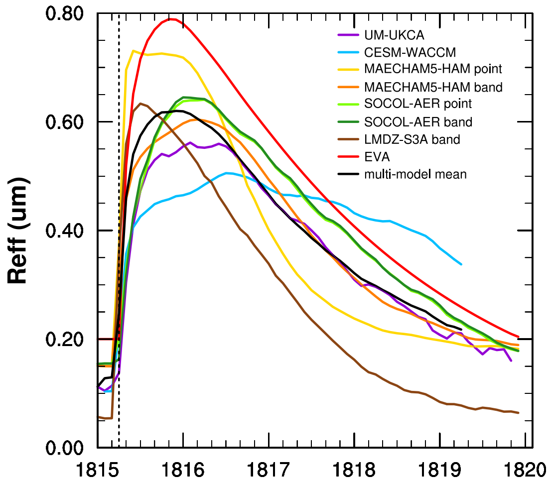
Figure 3: Global stratospheric mean effective radius ( Reff ) time series. Vertical dotted line marks date of injection of SO_2 . The calculation of Reff is weighted by surface aerosol density and gridcell volume, as explained in Appendix A.
