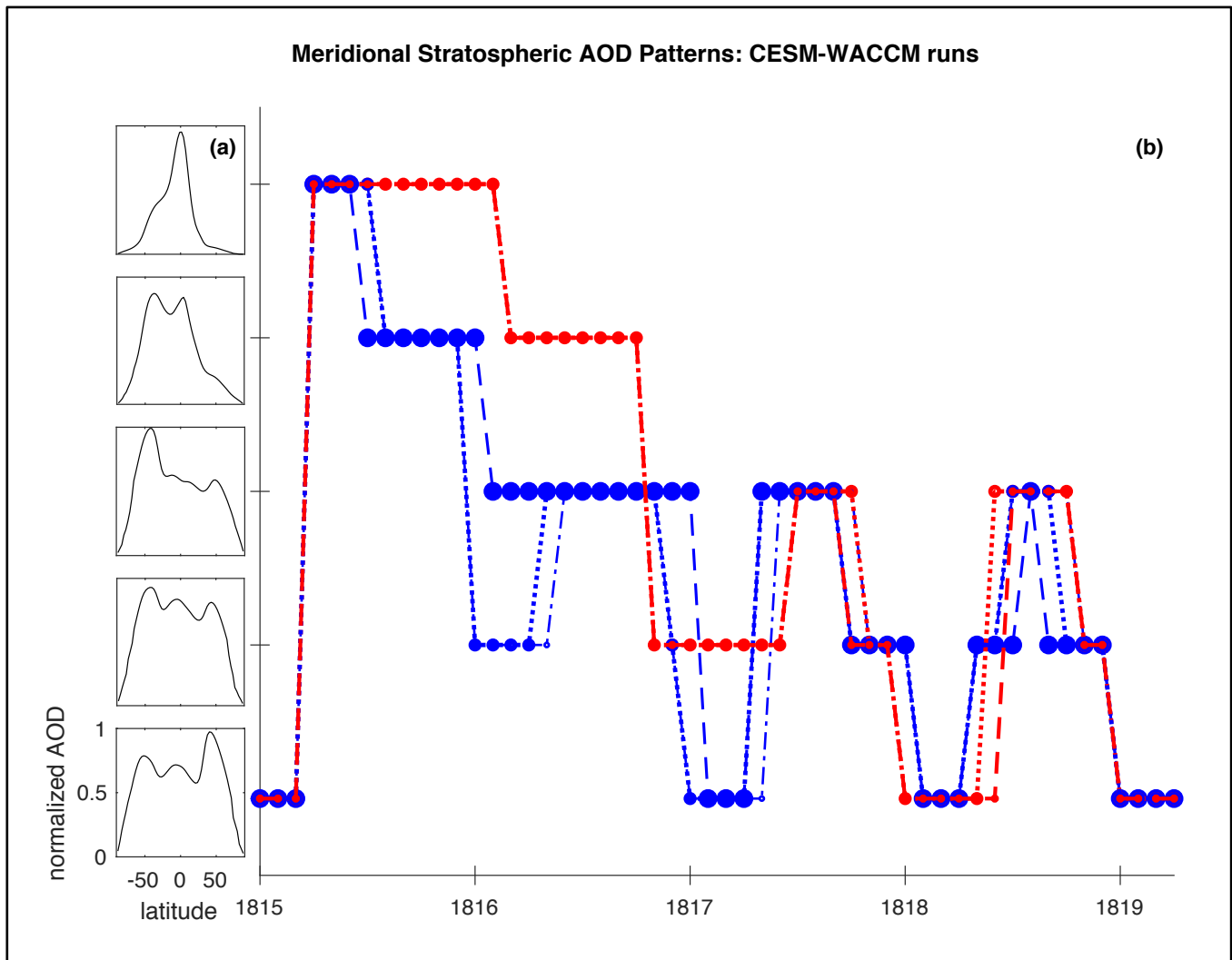
1170 Figure D2: Time evolution of stratospheric meridional circulation patterns of aerosol in terms of AOD for the five CESM-WACCM ensemble runs. This is presented in the same format as Fig. D1 except the meridional AOD patterns in (a) are now derived from only the CESM-WACCM ensemble runs when training the SOM. (b) Time evolution of CESM-WACCM ensemble runs using the easterly QBO forcing observed during 1982 (red) and easterly QBO forcing of 1991 (blue) mapping to which characteristic pattern in (a) best represents the run at each month.
