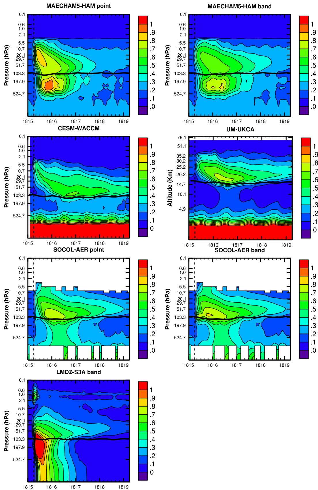
Figure 4: Vertical profile of tropical mean [23S, 23N] effective radius contours in units of \mu\text{m} marked by the colorbar. Vertical dashed line marks April 1815 injection. Horizontal solid black line marks tropopause height. The large particles in the lower troposphere in this figure (CESM-WACCM and UM-UKCA) are due to background particles such as sea spray and dust.
