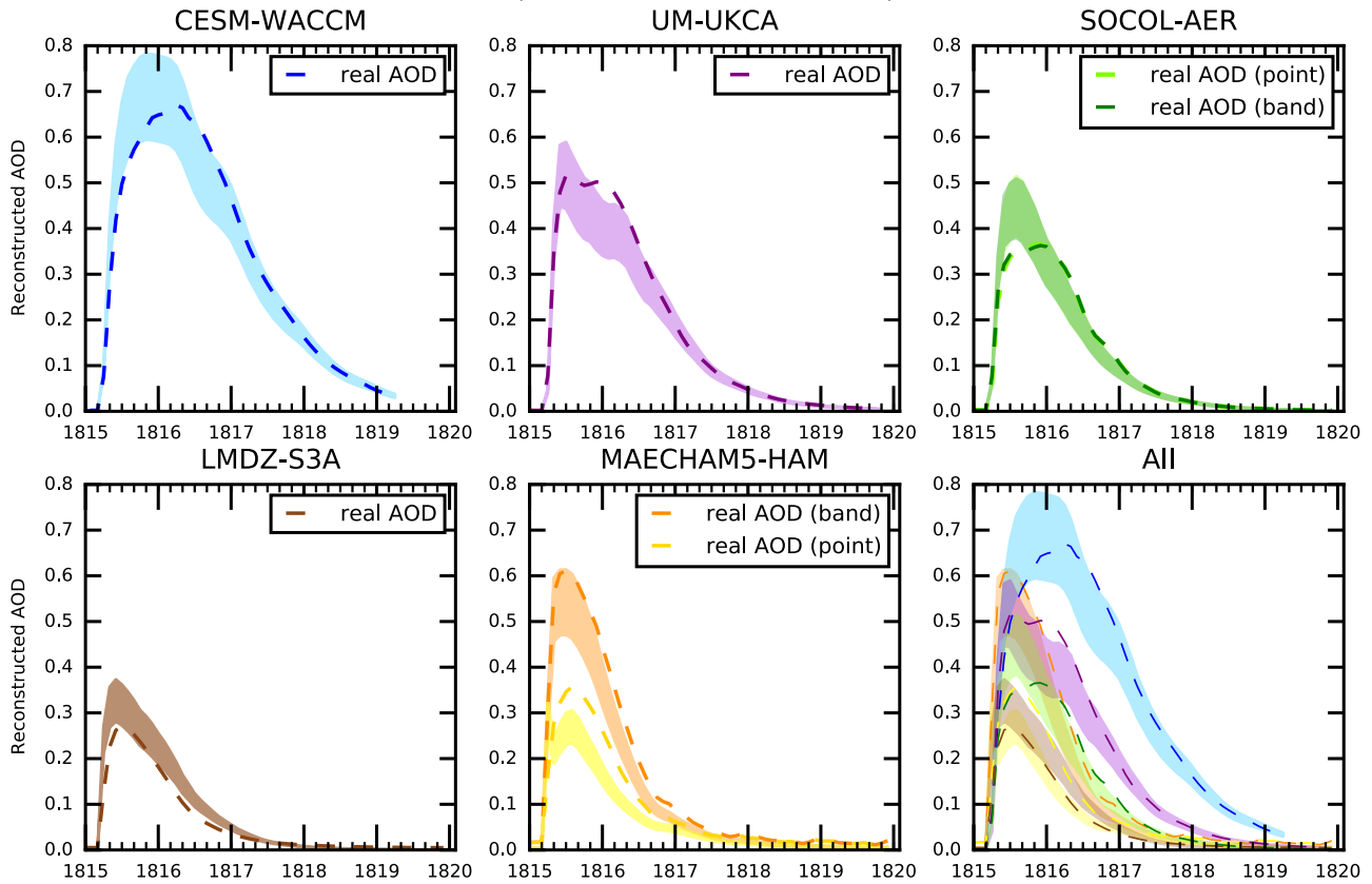
Reconstructed AOD from Eq.(1&2) (shaded \omega from 0.75 to 0.9)
