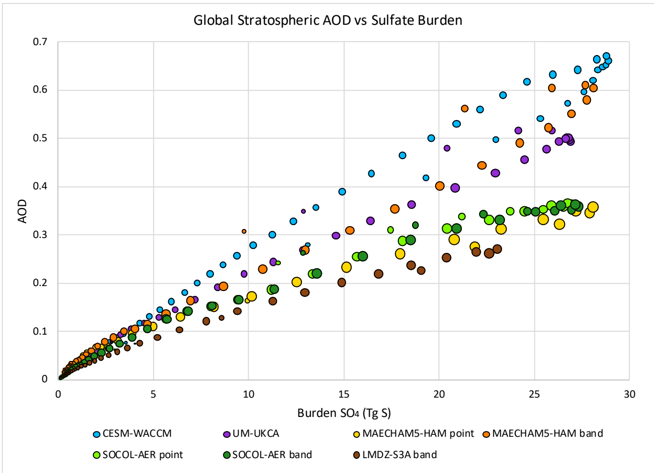
1130 Figure 5: Global stratospheric AOD in the visible vs sulfate burden from VolMIP-Tambora ISA ensemble means. Circle size is scaled by \pi(R_{eff})^2 .
