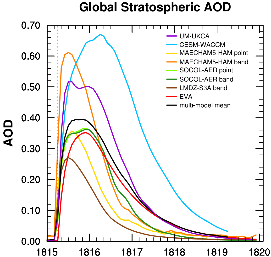
Figure 1: Ensemble mean global mean stratospheric AOD in the visible of participating models. The black line (the VolMIP-Tambora ISA ensemble mean) is the mean of CESM-WACCM (blue), UM-UKCA (purple), SOCOL-AER point (green), MAECHAM5-HAM point (gold), LMDZ-S3A band (dark brown) and EVA (red) models. SOCOL-AER and MAECHAM5-HAM band injection experiments are in green and orange respectively. Vertical dotted line marks date of injection of SO 2 , which is slightly offset from the zero AOD in the models due to the temporal resolution of the model output and curve smoothing in the plotting program.
