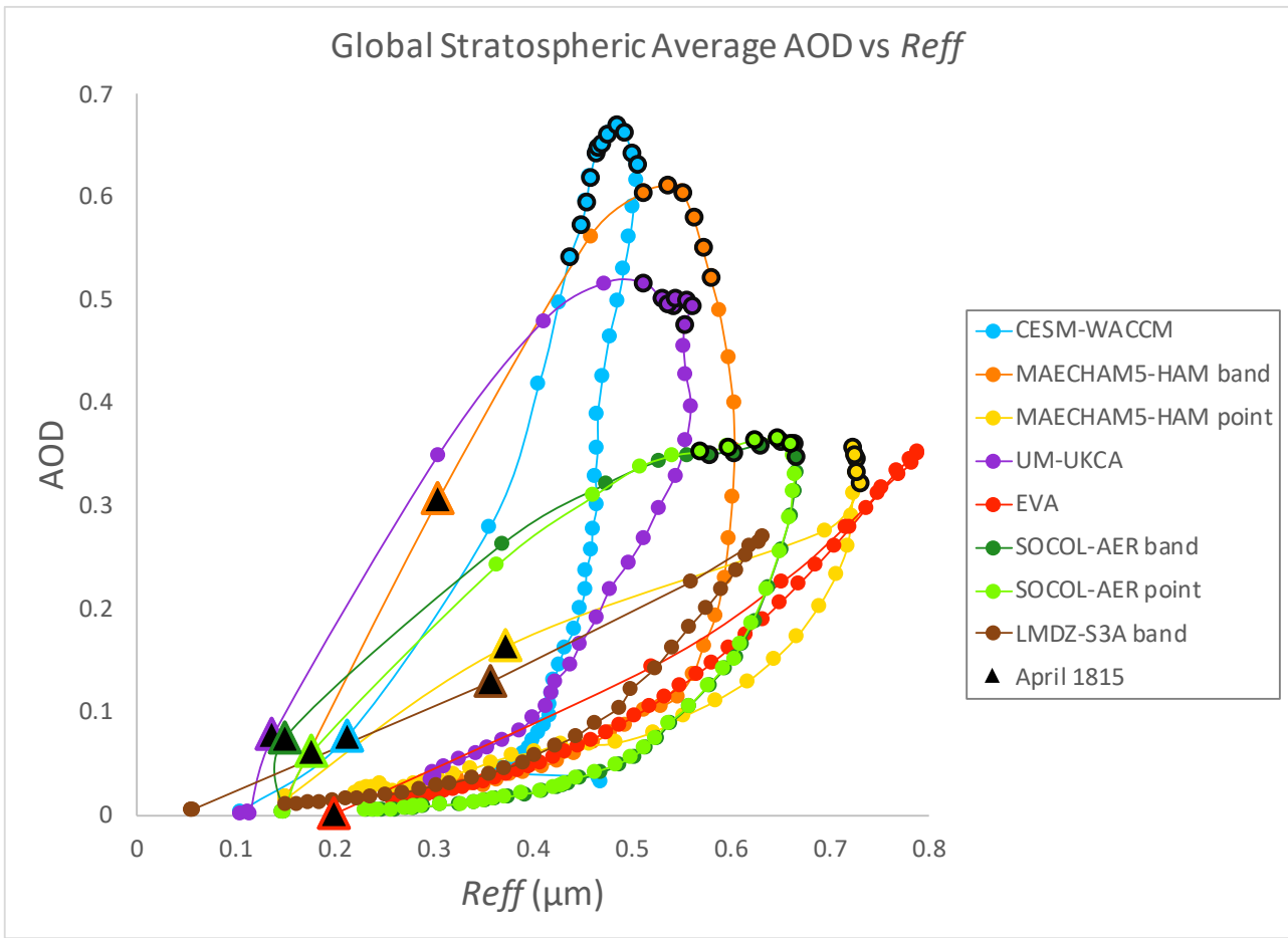
1135 Figure 6: Global stratospheric mean AOD in the visible vs effective radius ( \mu\text{m} ). Points are connected in order (clockwise) of monthly values from January 1815- April 1819. Circles with black outlines are for months when global stratospheric sulfate burden > 25 TgS. The injection date of April 1815 is indicated by triangles
