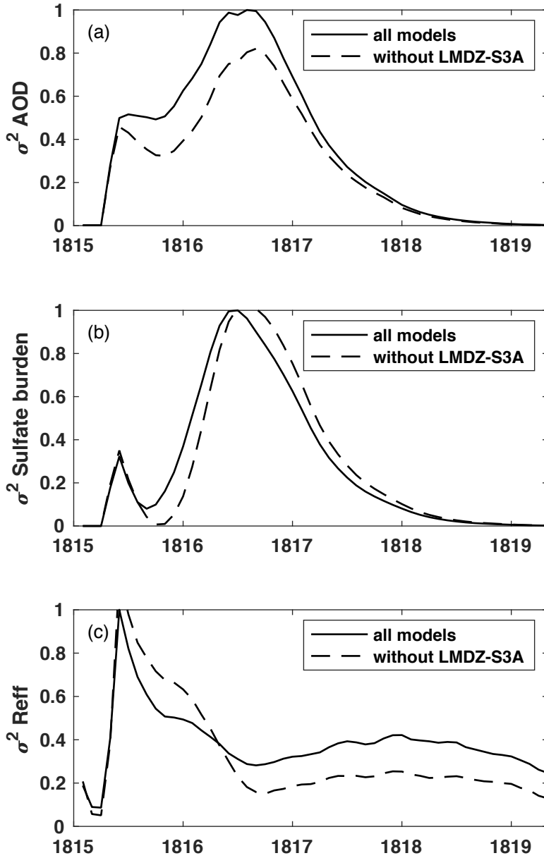
Figure 7: Variance between VolMIP-Tambora ISA ensemble models for global mean stratospheric a) AOD, b) sulfate burden, and c) effective radius. All models are included in the solid line. All models except for LMDZ-S3A are included in the dashed line. In both cases (solid and dashed lines), the plots have been normalized to the maximum value of the intermodel variance of all models (including LMDZ-S3A) at each corresponding variable. The peak values for the dashed line which are therefore slightly cut off from view by the y-axis of the subplots for the sulfate burden and effective radius are (b) 1.03 and (c) 1.16. Sulfate burden and effective radius are two of the key output variables dominating the AOD equation, Eq. (1), that generate intermodel variance of AOD.
