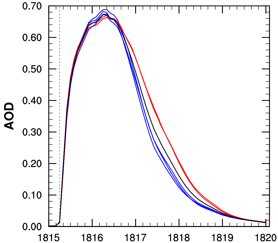
Figure 9: Global stratospheric mean AOD of the 5 CESM-WACCM ensemble runs. Easterly phase nudged QBO forcing is used from the observed strength starting with 1982 for two runs (red), and from the observed strength starting with 1991 for three runs (blue). The ensemble mean of the five runs is in black. Vertical dotted line marks date of injection of SO 2 .
