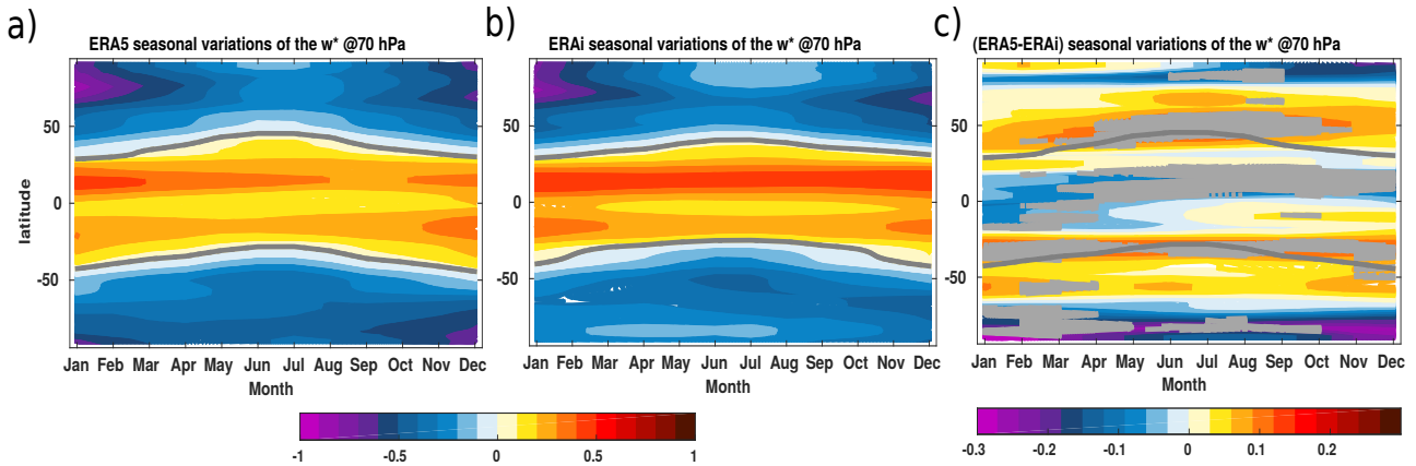
Figure 3. Monthly and latitudinal variations of monthly mean \overline{w^*} (in \text{mm} \cdot \text{s}^{-1} ) at 70 hPa from the ERA5 reanalysis (a), the ERA-Interim reanalysis (b), and the difference between the ERA5 and the ERA-Interim reanalyses (c) for the 1979–2018 period. Grey horizontal lines indicate the zero \overline{w^*} contours. Grey shading in panel (c) indicate regions where the differences between the ERA5 and ERA-Interim reanalyses are statistically significant at 95% confident level estimated using student t-test.
