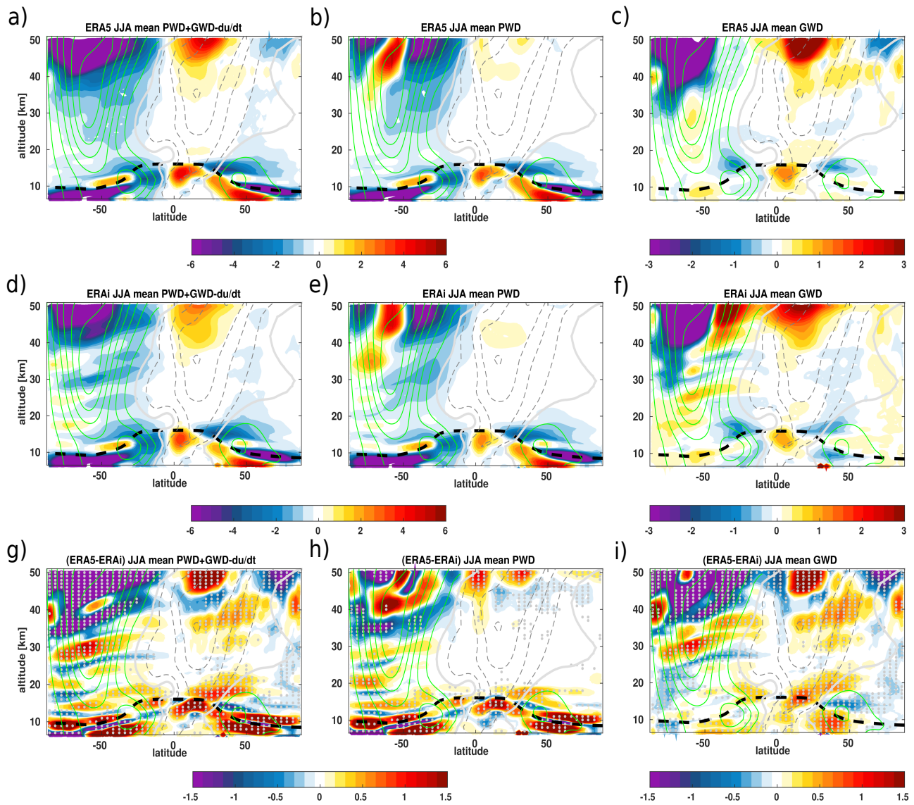
Figure A2. Zonal mean distribution of the summer seasonal mean (JJA) net wave forcing (a, d), planetary wave drag (b, e) and gravity wave drag (c, f), together with the associated differences (g-i) between the ERA5 (a-c) and ERA-Interim (d-f) reanalyses for the 1979–2018 time period. The unit of the wave drag is in \text{m} \cdot \text{s}^{-1} \cdot \text{day}^{-1} . Grey dots in panels (g, h, i) indicate regions where the differences between the ERA5 and ERA-Interim reanalyses are statistically significant at 95% estimated using student t-test. The climatological tropopause from the ERA-Interim is indicated as the black dashed horizontal line. The thick white line indicates the zero line zonal mean wind. The thin green and grey lines indicate the climatological zonal mean wind.
