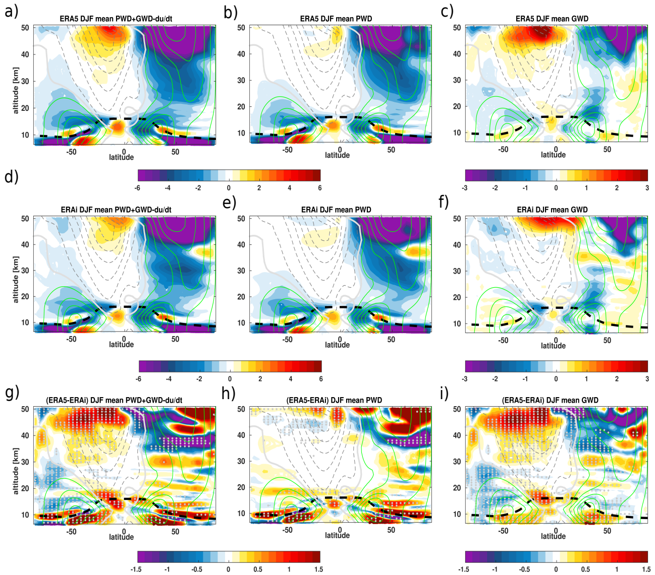
Figure A1. Zonal mean distribution of the winter seasonal mean (DJF) net wave forcing (planetary wave drag + gravity wave drag - du/dt ) ( a , d ), planetary wave drag ( b , e ) and gravity wave drag ( c , f ) together with the associated differences ( g-i ) between the ERA5 ( a-c ) and ERA-Interim ( d-f ) reanalyses for the 1979–2018 time period. The unit of the wave drag is in \text{m} \cdot \text{s}^{-1} \cdot \text{day}^{-1} . Grey dots in panels ( g , h , i ) indicate regions where the differences between the ERA5 and ERA-Interim reanalyses are statistically significant at 95% estimated using student t-test. The climatological tropopause from the ERA-Interim is indicated as the black dashed horizontal line. The thick white line indicates the zero line zonal mean wind. The thin green and grey lines indicate the climatological zonal mean wind.
