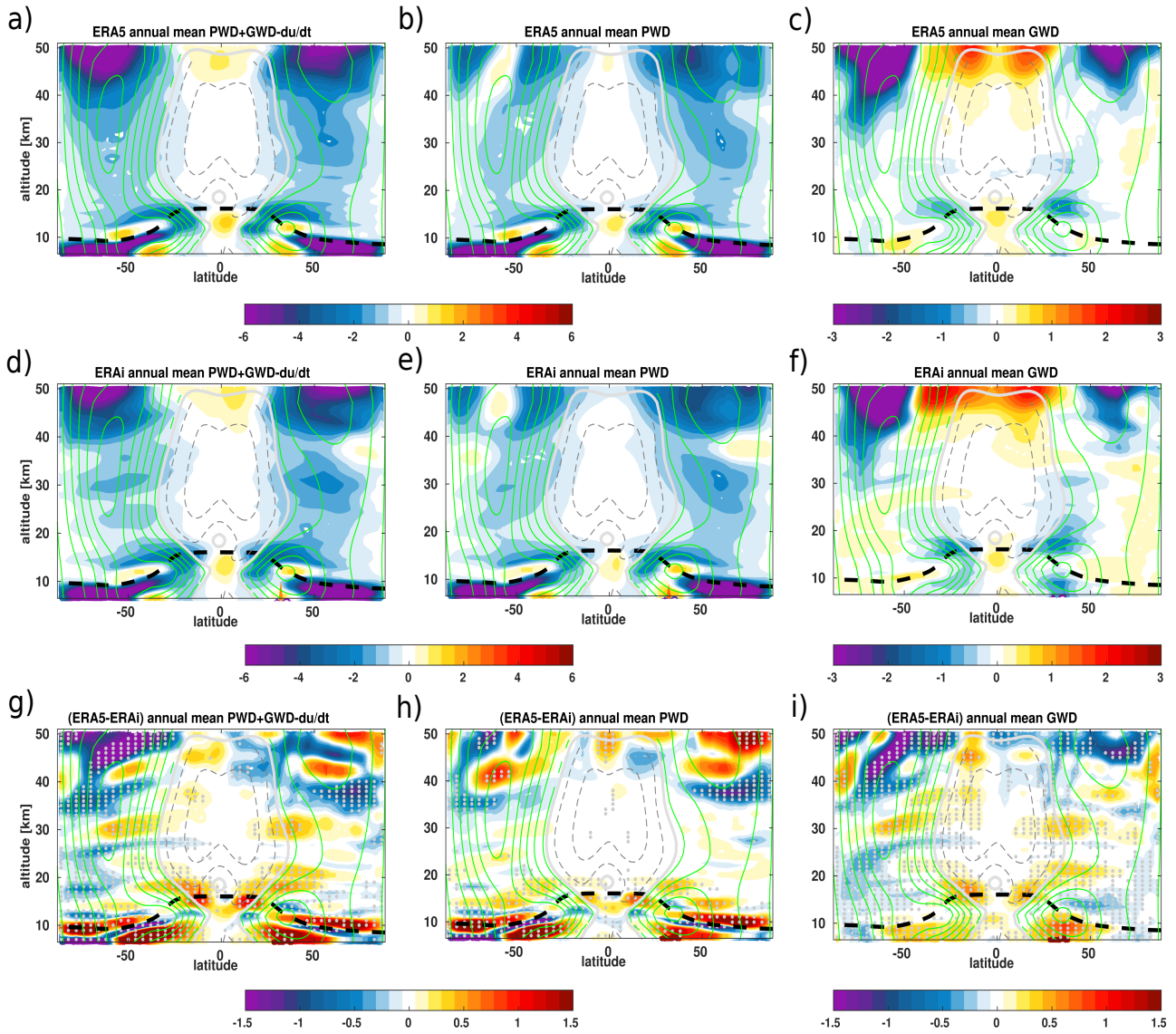
Figure 10. Zonal mean distribution of the annual mean net wave forcing (planetary wave drag + gravity wave drag - du/dt ) (a, d), planetary wave drag (b, e) and gravity wave drag (c, f) together with the associated differences (g-i) between the ERA5 (a-c) and ERA-Interim reanalyses (d-f) for the 1979–2018 time period. The unit of the wave drag is in m \cdot s^{-1} \cdot day^{-1} . The climatological tropopause from the ERA-Interim is indicated as the black dashed horizontal line. The thick white line indicates the zero line zonal mean wind. The thin green and grey lines indicate the climatological zonal mean wind. Grey dots in panels (g, h, i) indicate regions where the differences between the ERA5 and ERA-Interim reanalyses are statistically significant at 95% estimated using student t-test.
