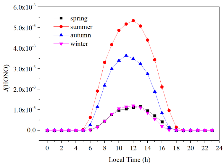
Figure S5: Diurnal variations of J(\text{HONO}) .
