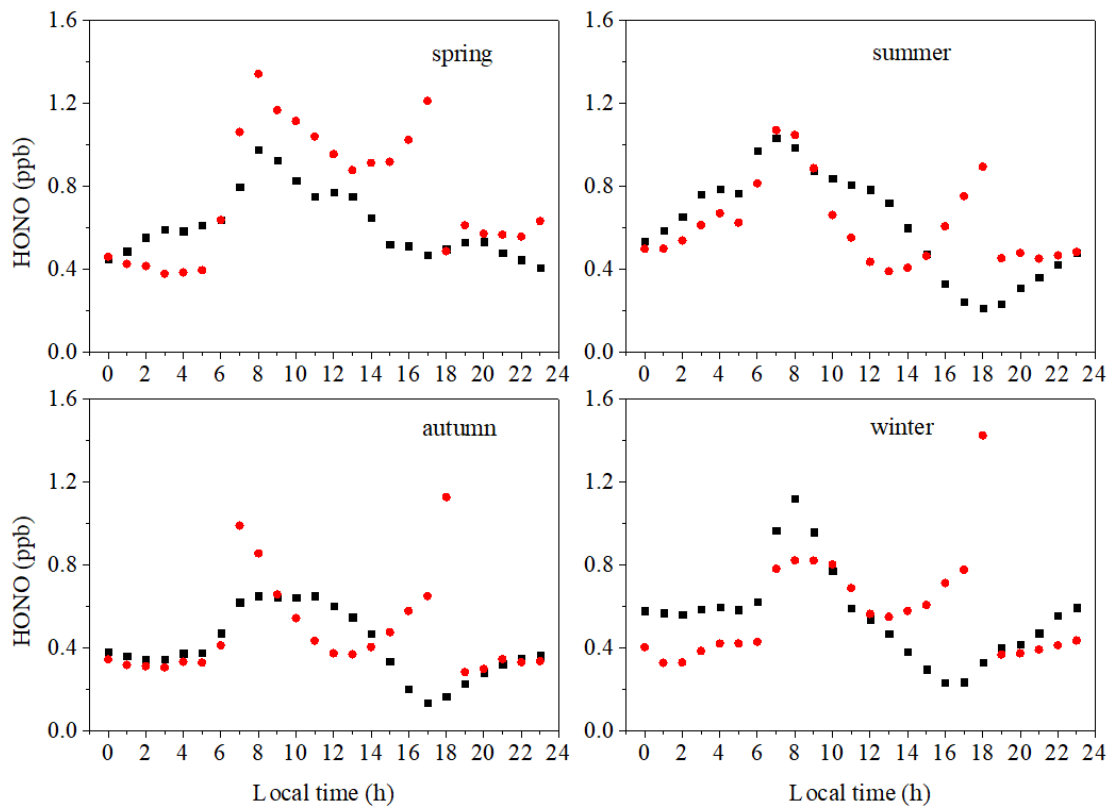
Figure S3: Diurnal profile of the measured values of HONO and the value estimated using the parameterized formula.
