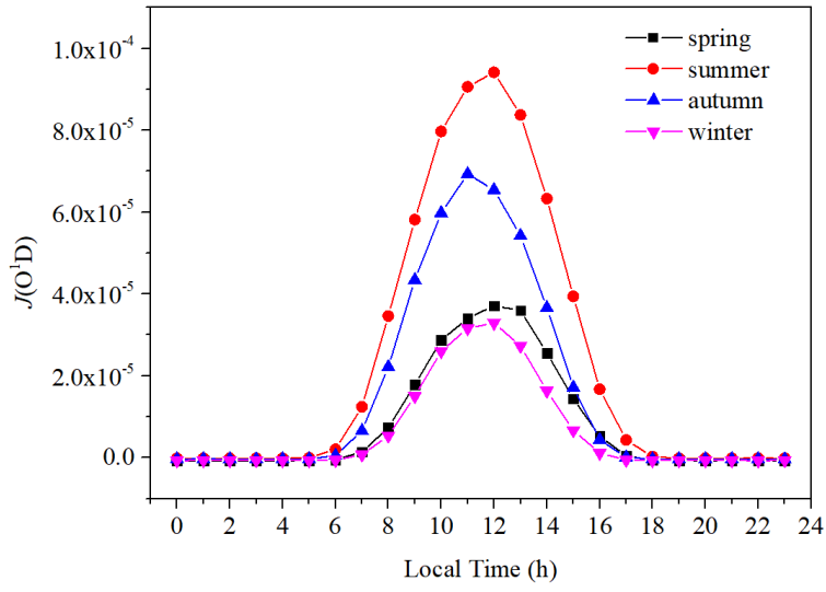
10 Figure S4: Diurnal variations of J(O^1D) .
