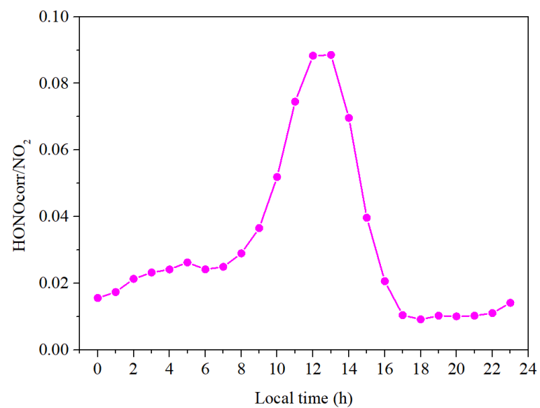
Figure S1: Diurnal variations of \text{HONO}_{\text{corr}}/\text{NO}_2 .
