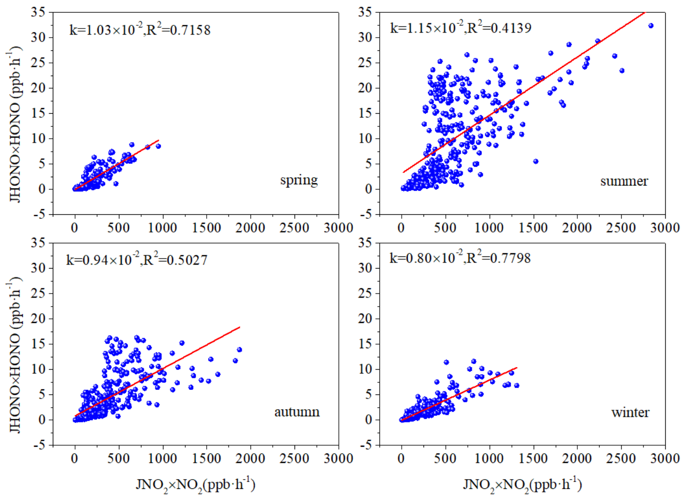
5 Figure S2: Correlations between J(\text{HONO}) \times \text{HONO} and J(\text{NO}_2) \times \text{NO}_2 .
