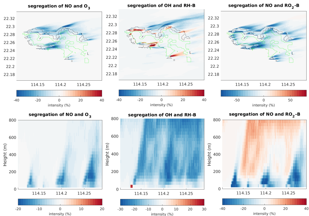
830 Figure 7: Segregation intensities at the first level (top panel) and the vertical cross section along latitude 22.275 °N (bottom panel) 835 at hour 4 for HETF case. The black line shows the urban area and the green line shows the forest area.
