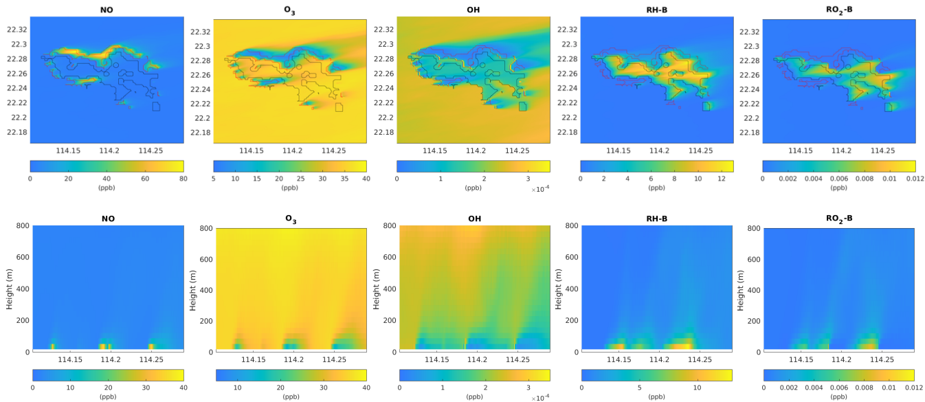
Figure 6: Volume mixing ratio of the chemical species at the first level (top panel) and vertical cross section along latitude 22.275 °N (bottom panel) at hour 4 for HETF case. The red line shows the urban area and the black line shows the forest area.
