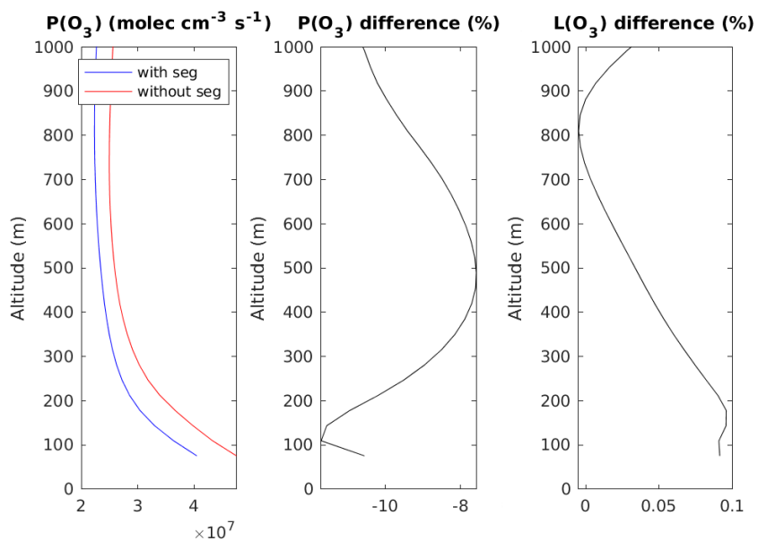
885 Figure 15b. Left panel: vertical distribution of the ozone production rate (molecules cm^{-3} s^{-1} ) averaged over the central 14 \times 14 km^2 of the inner domain with the effect of segregation taken into account (red curve) or ignored (blue curve). Middle and right panels: percentage difference between the two cases for the photochemical production and destruction rates.
