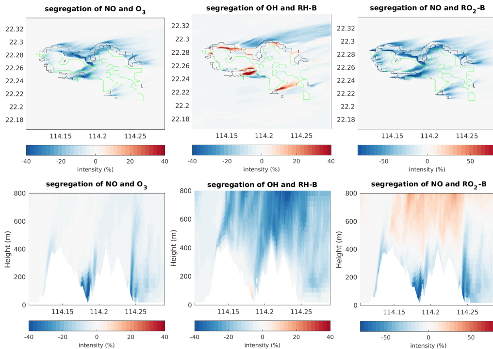
Figure 10: Same as Fig. 6, but for TERW case.
