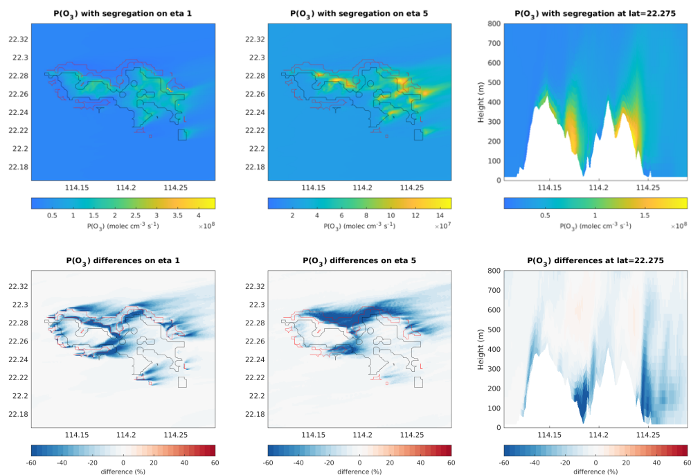
Figure 15a. Upper panels: production rate of ozone (molecules \text{cm}^{-3} \text{s}^{-1} ) in and around the Hong Kong Island. From left to right: values at the lowest model level, values at model level 5 and values as a function of height along the constant latitude of 22.275 °N. Lower panels: Same, but for the percentage difference between ozone production rates with and without segregation effects taken into account.
