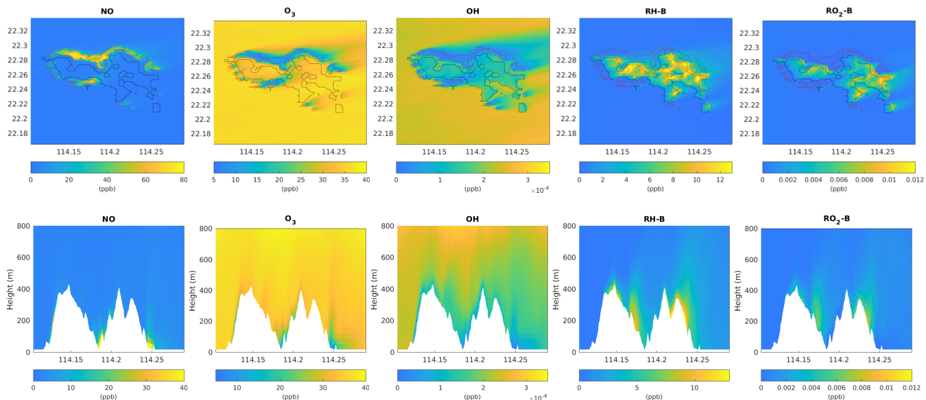
Figure 9: Same as Fig. 5, but for TERW case.
