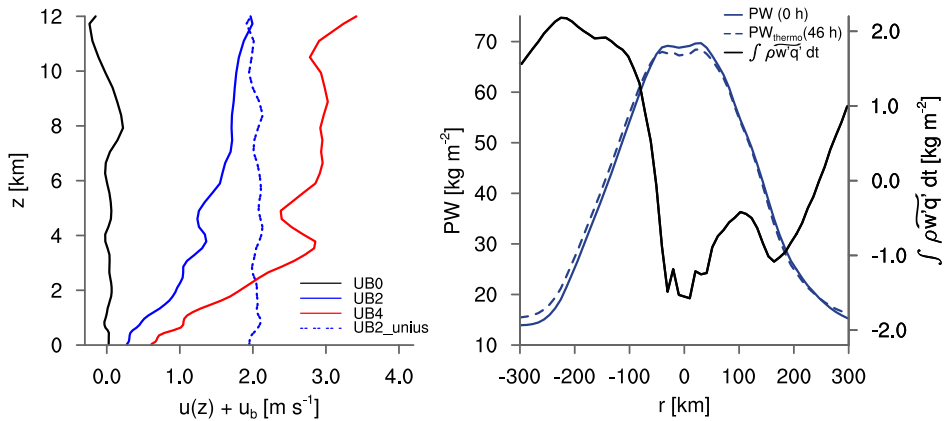
Figure 5. (Left) vertical profile of the domain-mean horizontal x -component wind as sum of the modeled wind u(z) in the x -direction and u_b for the quasi-stationary stage. Note that the horizontal wind considers the Galilean transformation by including u_b . Colors as in Fig. 2. (Right) radial distributions of PW at 0 h, the estimated PW at 46 h due to the thermodynamic process alone, and the accumulated surface moisture flux anomaly from 0 h to 46 h. The quantities are azimuthally averaged.
