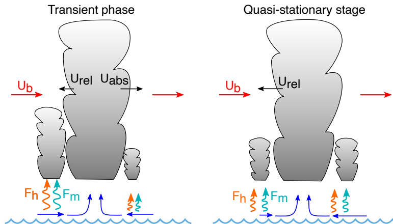
Figure 7. Sketch of the convective cluster, the surface wind field, the imposed mean wind ( u_b ), the surface enthalpy flux ( \text{SEF } F_h ) and the momentum flux ( F_m ).
