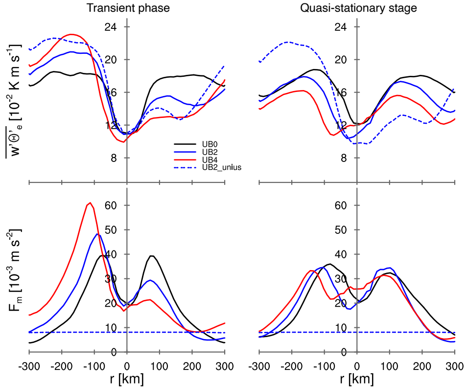
Figure 3. Radial distributions of the azimuthally averaged (top) \overline{w'\theta'_e} and (bottom) F_m . Quantities are averaged over 5 days and 10 km in r -direction . The averaged quantities for (left) transient stage over day 0 to 4 and (right) quasi-stationary stage over 15 to 19 are illustrated. The negative and positive values of r represent the upwind area and downwind area, respectively. Colors as in Fig. 2.
