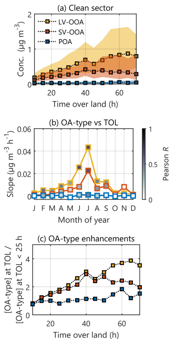
Figure 12 (a) The different rolling rCMB factors ( y axes in \mu\text{g m}^{-3} ) vs TOL ( x axes in hours) for the clean sector (least polluted north-western sector as defined by Tunved et al., 2006; see Fig. S.2 for a more precise sector definition). The data are binned to 5-hourly TOL bins. The shaded areas represents the concentration interquartile ranges (25 th to 75 th percentile) and the square markers the median concentrations. (b) The slopes (in \mu\text{g m}^{-3} \text{ h}^{-1} ) are calculated for a linear fit between TOL ([20, 70] h) and the three different OA types. (c) The OA type concentration in the TOL bin divided by the median OA type concentration when TOL was < 25 h as a function of TOL. The plot visualizes how the SV-OOA and LV-OOA have similar behaviour until TOL = 40 h.
