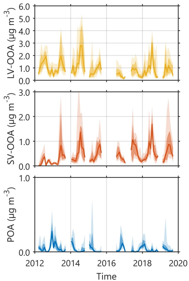
760 Figure 7 Monthly resolution time series of LV-OOA (panel a), SV-OOA (panel b) and POA (panel c) mass concentrations obtained with rolling rCMB. The light shadings indicate the area between the 10 th and 90 th percentiles, and the dark shadings the area between the 25 th and 75 th percentiles. The solid line represents the monthly medians for each month of measurements in 2012 – 2019. Note the different y-axis scales (grid lines are drawn every 1 \mu\text{g m}^{-3} ).
