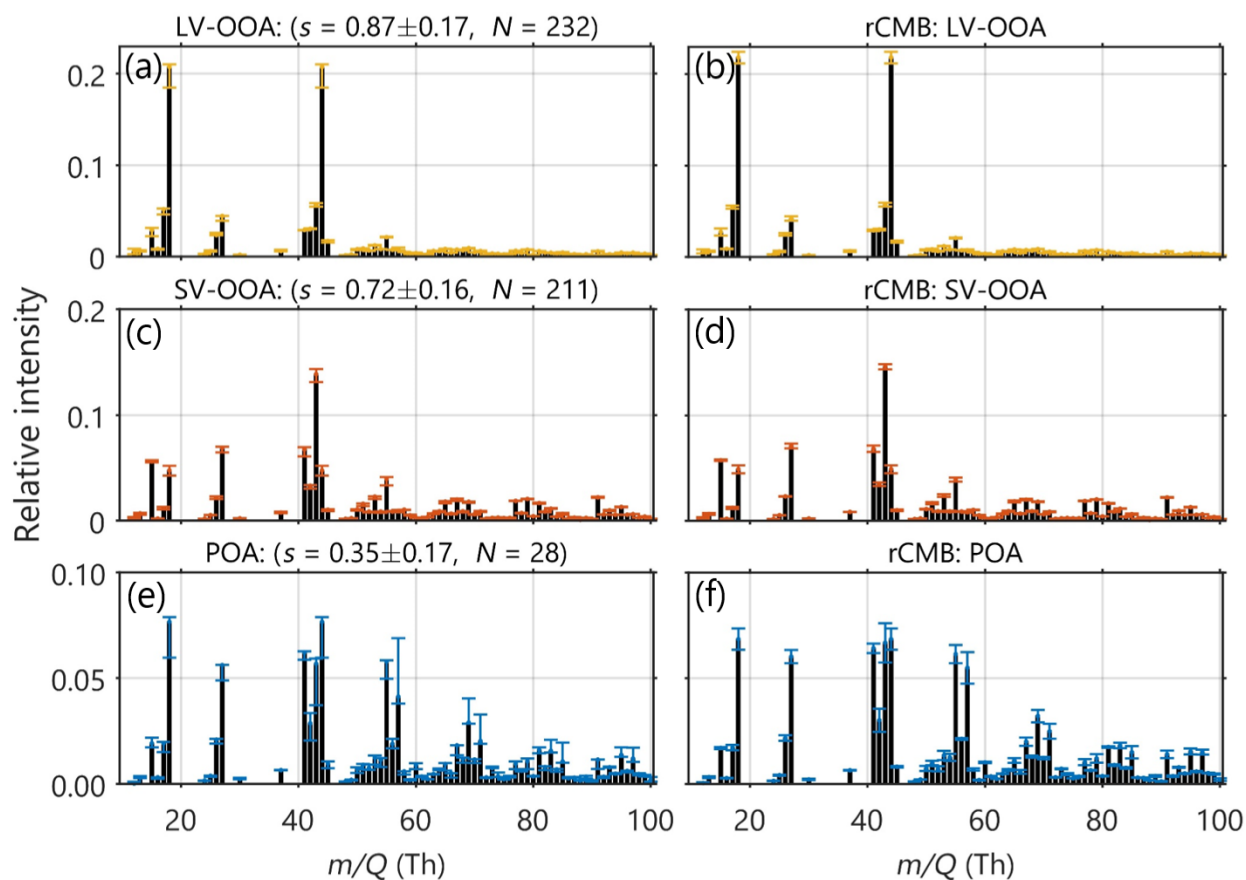
645 Figure 5 The left panels (a, c, e) represent silhouette-weighted median cluster centroid mass spectra obtained when the number of clusters (k) equals 3 in Phase II K-Means clustering (final result). Here, y-axis indicates the relative signal intensity and x-axis the mass-to-charge ratio ( m/Q ) the cluster centroid mass spectra identified as low volatility oxygenated organic aerosol (LV-OOA), semi-volatile oxygenated organic aerosol (SV-OOA) and primary OA (POA). The panel titles include the mean \pm standard deviation of the cluster silhouette score ( s ), and the number of spectra belonging to each cluster ( N ). The error bars visualize the 25 th and 75 th percentiles (i.e. the lower and higher 650 quartiles). The right panels (b, d, f) show the mean LV-OOA, SV-OOA and POA mass spectra obtained from rolling rCMB. The error bars visualize the standard deviation of each m/Q signal fraction.
