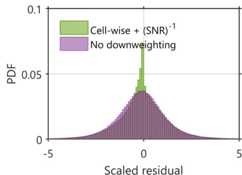
Figure 4 Normalized histograms (probability density function, PDF) of the scaled residuals obtained from rolling rCMB. The effect of downweighting weak/bad variables is visible by the high scaled residual frequencies at negative near-zero readings. If rolling rCMB was conducted without downweighting the scaled residual distribution behaves in a highly normal manner.
