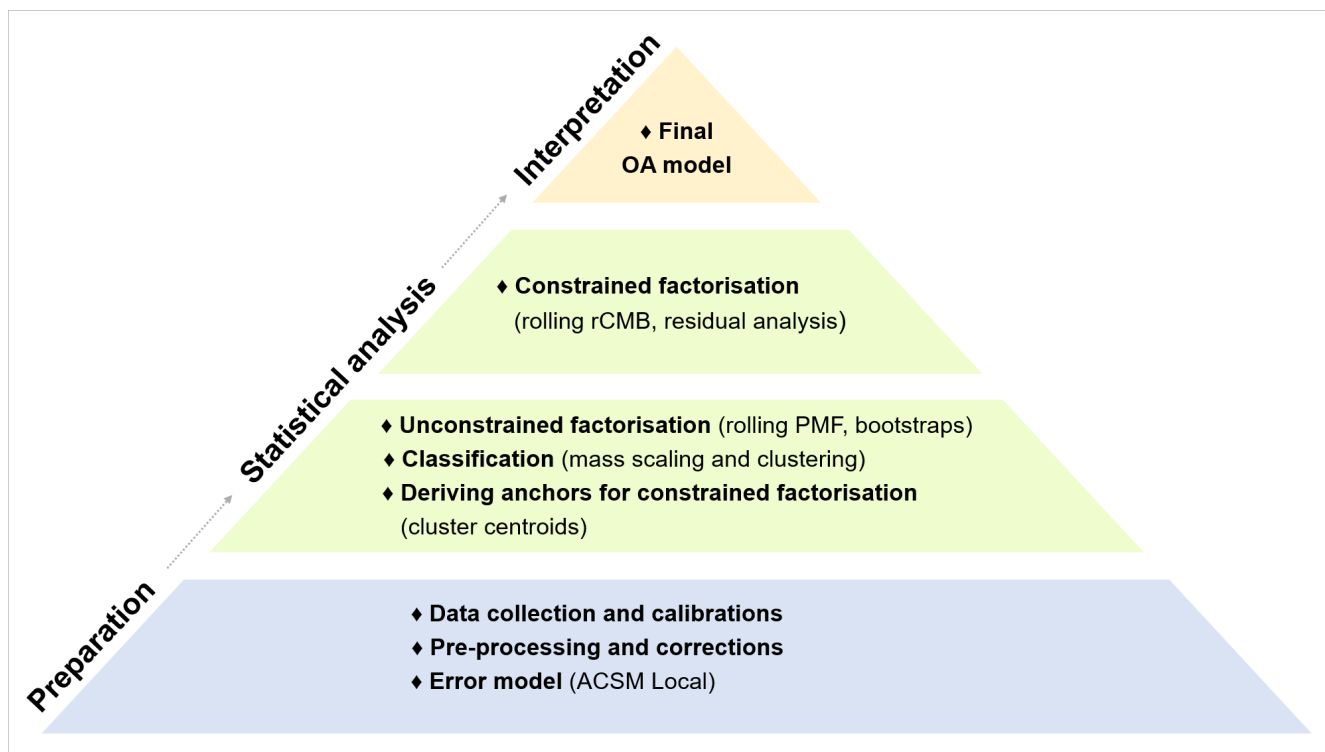
375 Figure 1 A pyramid flow chart, roughly describing the steps from data collection to the final OA model (i.e. the time series of OA components making up the total OA signal). The statistical analysis steps (in green) are explained further in detail in sections 4 and 5 in the paper as well as listed in Appendix A.
