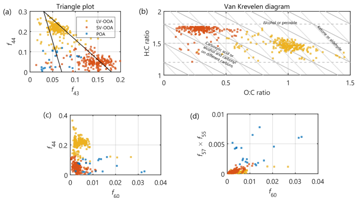
655 Figure 6 (a) A triangle plot visualizing the mass spectra distribution in each cluster in f_{44} vs f_{43} space, (b) Van Krevelen diagram visualizing the mass spectra in H:C vs O:C space for LV-OOA and SV-OOA, (c) mass spectra in f_{44} vs f_{60} space for indications of fresh BBOA, (d) f_{55} \times f_{57} vs f_{60} space for indications of HOA and BBOA.
