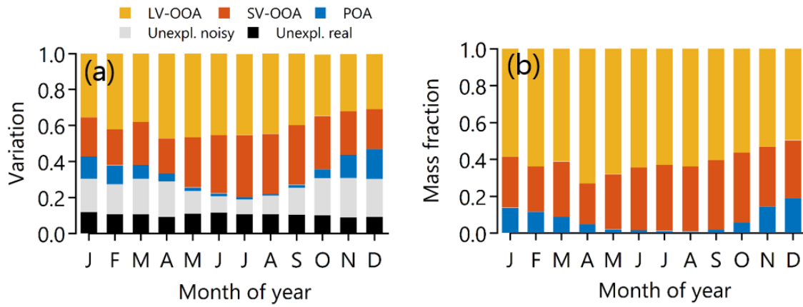
Figure 8 The panel (a) depicts the variability of the rolling rCMB compared to measurement variability (scaled by uncertainty). The unexplained fraction is ca. 30% outside summer, when its ca. 25%. This variation in the unexplained variation is due to increased noisy fraction (light grey) outside summer. The real unexplained fraction (in black) stays at rather constant of ca. 11%. Panel (b) shows f_{LV-OOA} , f_{SV-OOA} and f_{POA} in different months. This panel only visualizes their variability in rolling rCMB.
