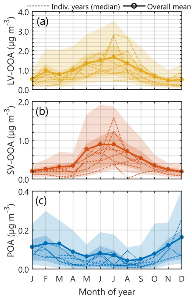
775 Figure 9 The monthly mass concentrations of LV-OOA (panel a), SV-OOA (panel b) and POA (panel c) obtained with rolling rCMB. The light shadings indicate the area between the 10 th and 90 th percentiles, and the dark shadings the area between the 25 th and 75 th percentiles. The narrow dotted lines represent monthly medians for individual years and the dark lines with circled markers represent the overall monthly mean concentrations. Note the different y-axes scales (grid lines are drawn every 0.2 \mu\text{g m}^{-3} ).
