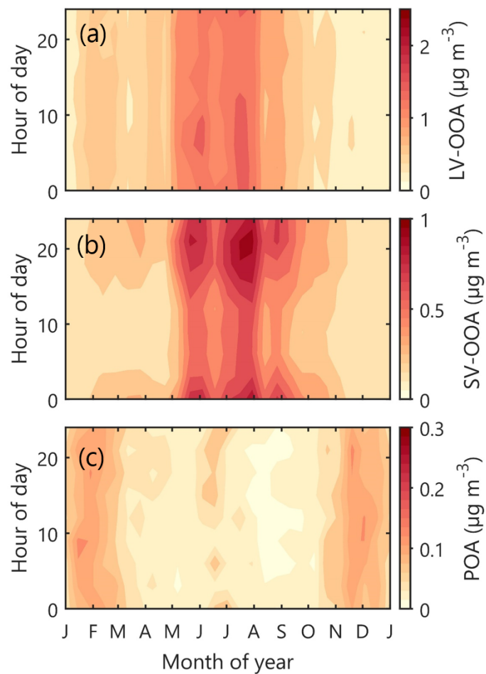
Figure 10 The median diel cycles of LV-OOA (panel a), SV-OOA (panel b) and POA (panel c) obtained via rolling rCMB. The y-axes represent the local time of day (UTC+2) and x-axes the month. The colour scales represent the mass concentration of each OA type. Note the different scales for each plot. Each grid point represents a 14d \times 3h period, visualized with the MATLAB 2017a contourf function.
