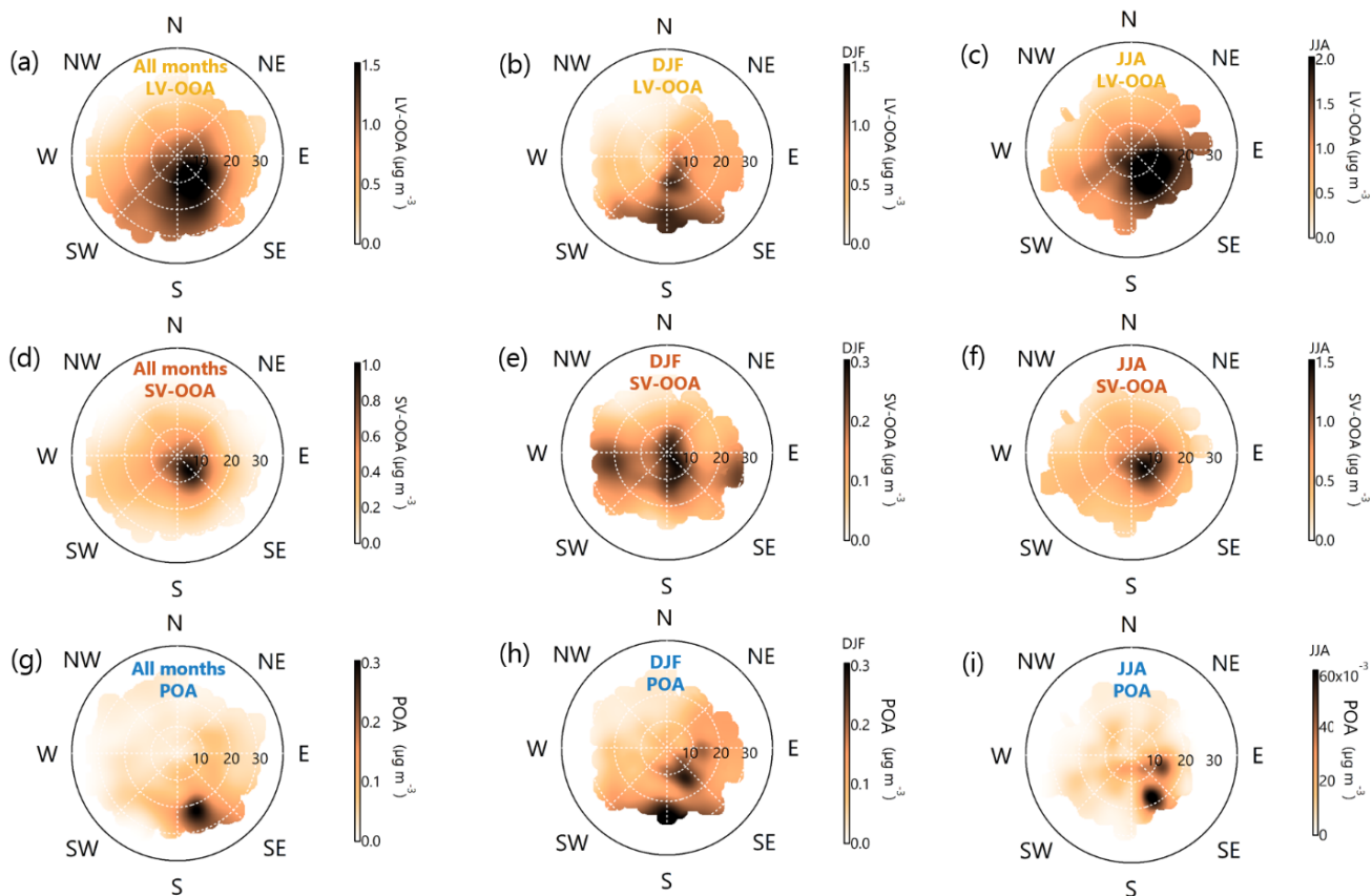
Figure 11 Openair polar plots (Carslaw and Ropkins, 2012) for LV-OOA (first row), SV-OOA (second row) and POA (third row) obtained via ZeFir pollution tracker Wavemetrics Igor Pro toolkit (Petit et al., 2017). The first column represents the median over all seasons, the second column the median over wintertime and third the median summertime. The distances from the circle origins indicate wind speeds (in \text{km h}^{-1} ). Wind speed grid lines are presented with dark grey dashed lines. The colour scales represent the mass concentration of each OA type modelled via rolling rCMB during the specific wind direction and speed combinations. Note that the scales are different among the subplots. As these figures do not indicate any likelihood of these wind direction and speed combinations, Fig. S.1 is important to keep in mind while interpreting them. Briefly, N-NE-E is the least likely direction of wind, and S-SW-W is the most likely. Wind speeds rarely exhibit 20 \text{ km h}^{-1} . The wind direction and speed data are collected above the boreal forest canopy.
