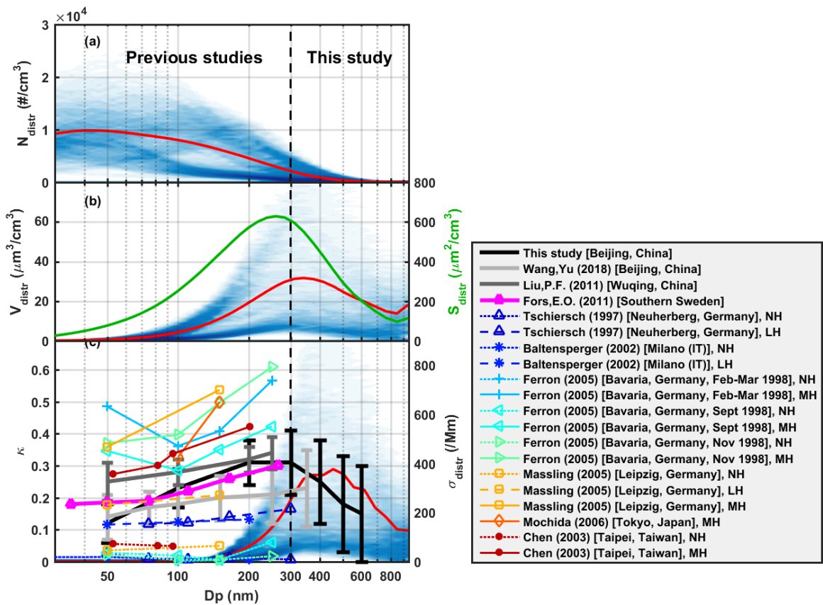
625 Figure 24: Frequency distribution of (a) aerosol number size distribution during the whole measurement period, (b) corresponding volume size distribution and (c) size-resolved light extinction coefficient contribution calculated from Mie theory. The red lines in (a-c) represent the mean values. The lines with marks in Fig. 1(c) denote the hygroscopicity measurement by HTDMA in previous and our studies.
