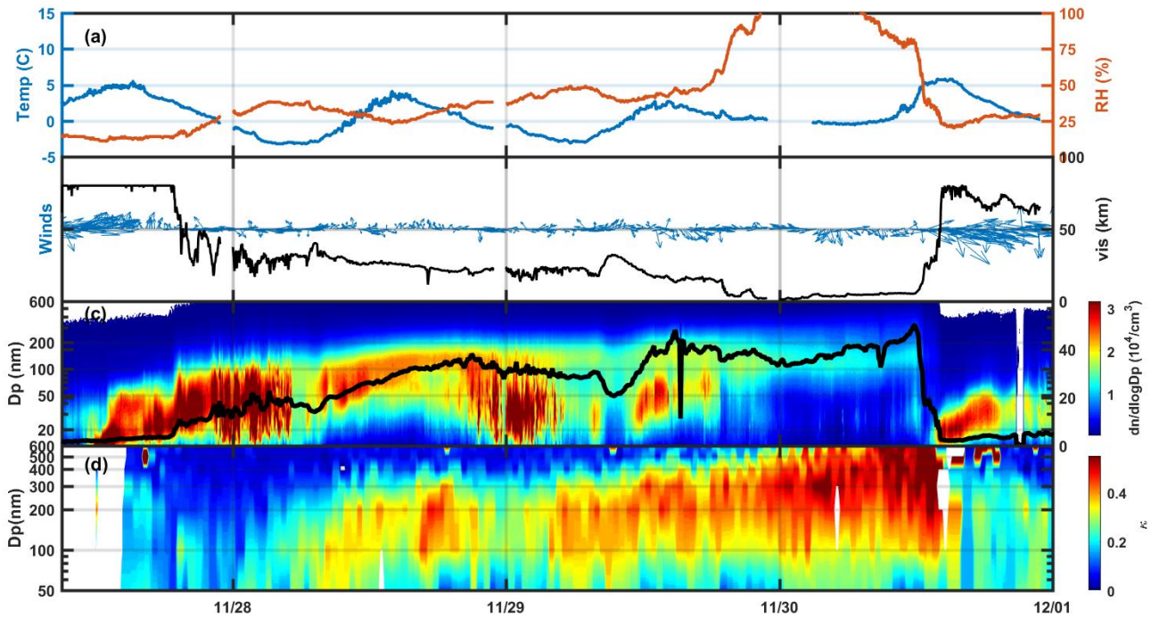
Figure 7: A pollution cycle from 11/27/2019 to 12/01/2019. (a) is the temporal evolution of temperature (blue line) and RH (orange line); (b) is the time series of visibility (black line) and wind speed. The length of the arrow indicates the wind speed, and the direction of the arrow indicates the wind direction. colour of the points denotes the direction of wind. (c) stands for the time series of particle number size distribution and the black line is the integrated volume concentration. Left axis is the log scale of particle diameters and right axis is for the volume concentration. (d) is the size-resolved hygroscopicity parameter \kappa .
