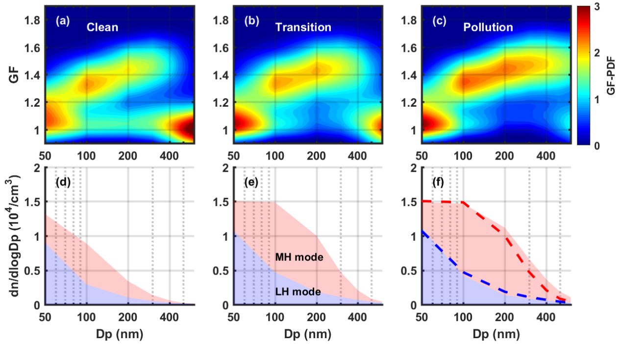
650 Figure 5: (a-c) are the growth factor probability distribution under different pollution conditions. (d-f) are the corresponding mean number size distribution for LH and MH mode. For comparison, we also mark the mean number size distribution under transition stage in dashed lines in panel (f).
