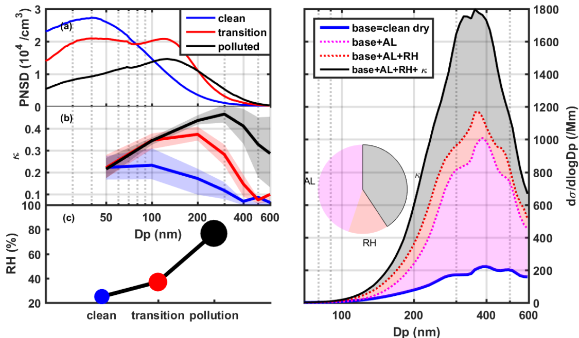
670 Figure 8: (a) is the mean PNSD under different pollution conditions. (b) is the mean size-resolved \kappa under different pollution conditions. (c) is the mean RH under different conditions. (d) shows the effects of different factors (aerosol loading, RH and \kappa variation) to the size-resolved light extinction. The areas of different colors are shown in the pie chart on the left.
