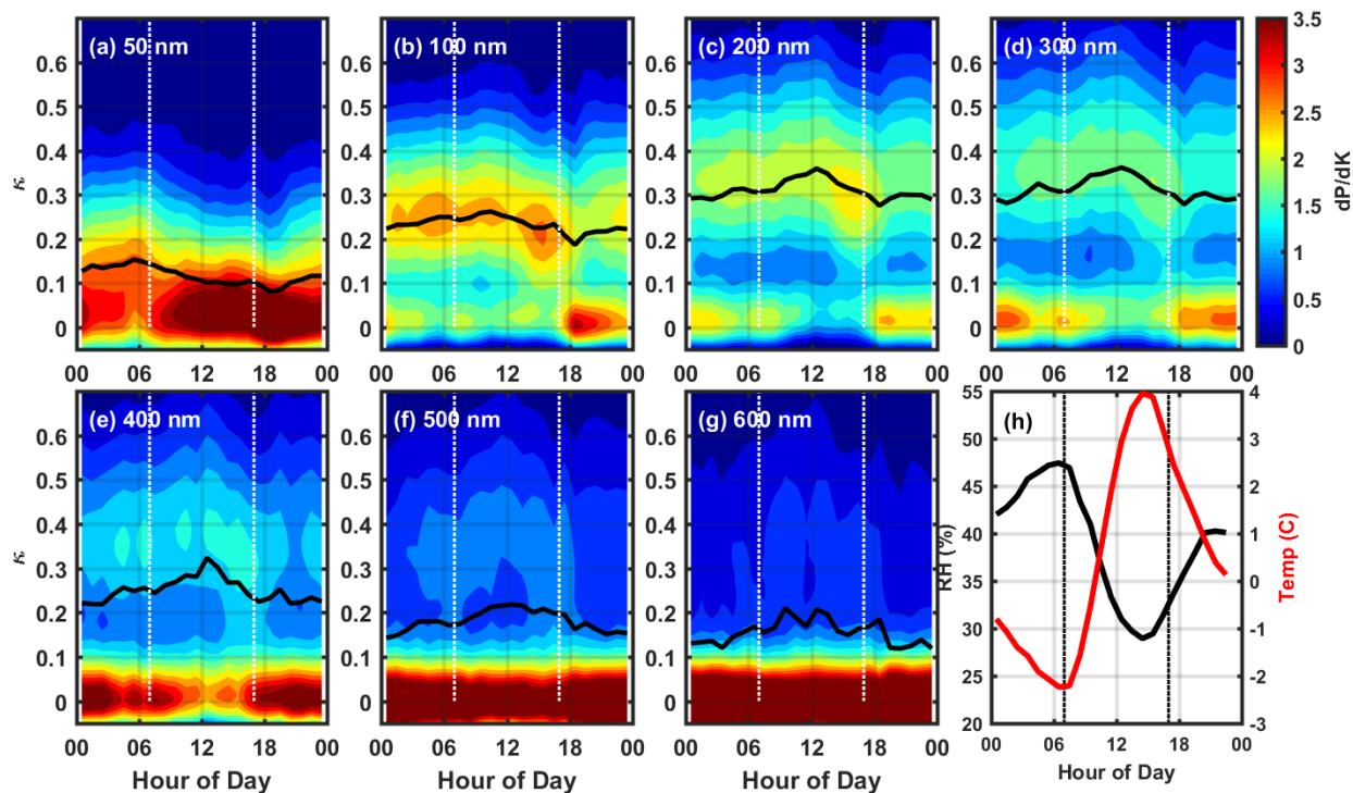
645 Figure 4: Diurnal variations of aerosol hygroscopicity distribution function over different sizes from 50 nm to 600 nm. Panel (h) shows the mean diurnal temperature and relative humidity. The black lines in (a-g) are the mean hygroscopicity calculated from the average \kappa -PDF. The vertical dotted lines in all the figures denote the time of sunrise (~7.00 a.m.) and sunset (~5.00 p.m.).
