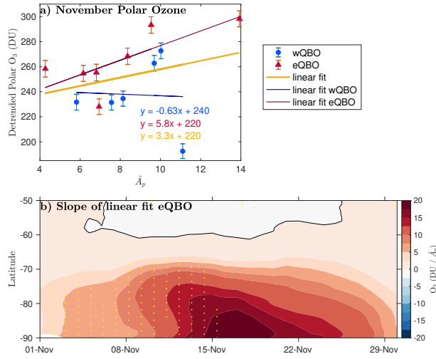
Figure 5. a) \hat{A}_p vs. OMI detrended polar ozone averaged over 60°S to 90°S with \cos(\text{latitude}) weighting. Blue circles indicate years with wQBO phase and red triangles indicate with eQBO (eQBO and wQBO years as given in Table 1). The lines show linear best fit with yellow fitting all data, blue fitting wQBO and red fitting eQBO. Corresponding equations for these are included in corresponding colours. Error bars are 2 times the standard error in the mean. b) Evolution of the slope of the linear best fit between \hat{A}_p and OMI O 3 over November in the polar stratosphere in eQBO years. The horizontal axis is time from the 1st to 30th of November and the y-axis is latitude from 90°S to 50°S. Contour interval is 2.5 DU/ \hat{A}_p . Stippling from Figure 4b) is superimposed as reference to show where the OMI O 3 and \hat{A}_p correlation was found to be significant at 95 % or higher.
