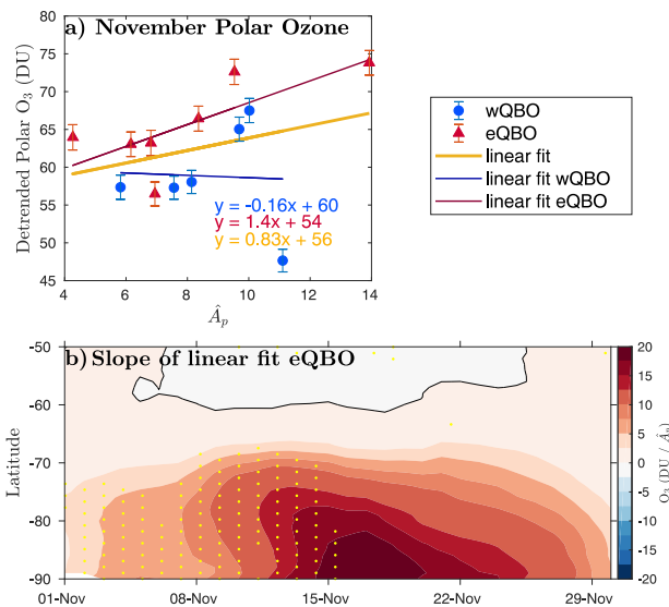
Figure 5. a) \hat{A}_p vs. OMI detrended polar ozone averaged over 60°S to 90°S with \cos(\text{latitude}) weighting (note that this results in DU values that appear low when contrasted to non-area weighted values such as those in Figure 3a). Blue circles indicate years with wQBO phase and red triangles indicate with eQBO (eQBO and wQBO years as given in Table 1). The lines show linear best fit with yellow fitting all data, blue fitting wQBO and red fitting eQBO. Corresponding equations for these are included in corresponding colours. Error bars are 2 times the standard error in the mean. b) Evolution of the gradient slope of the linear best fit between \hat{A}_p and OMI O 3 over November in the polar stratosphere in eQBO years. The horizontal axis is time from the 1st to 30th of November and the y-axis is latitude from 90°S to 50°S. Contour interval is 2.5 DU/ \hat{A}_p . Stippling from Figure 4b) is superimposed as reference to show where the OMI O 3 and \hat{A}_p correlation was found to be significant at 95 % or higher.
