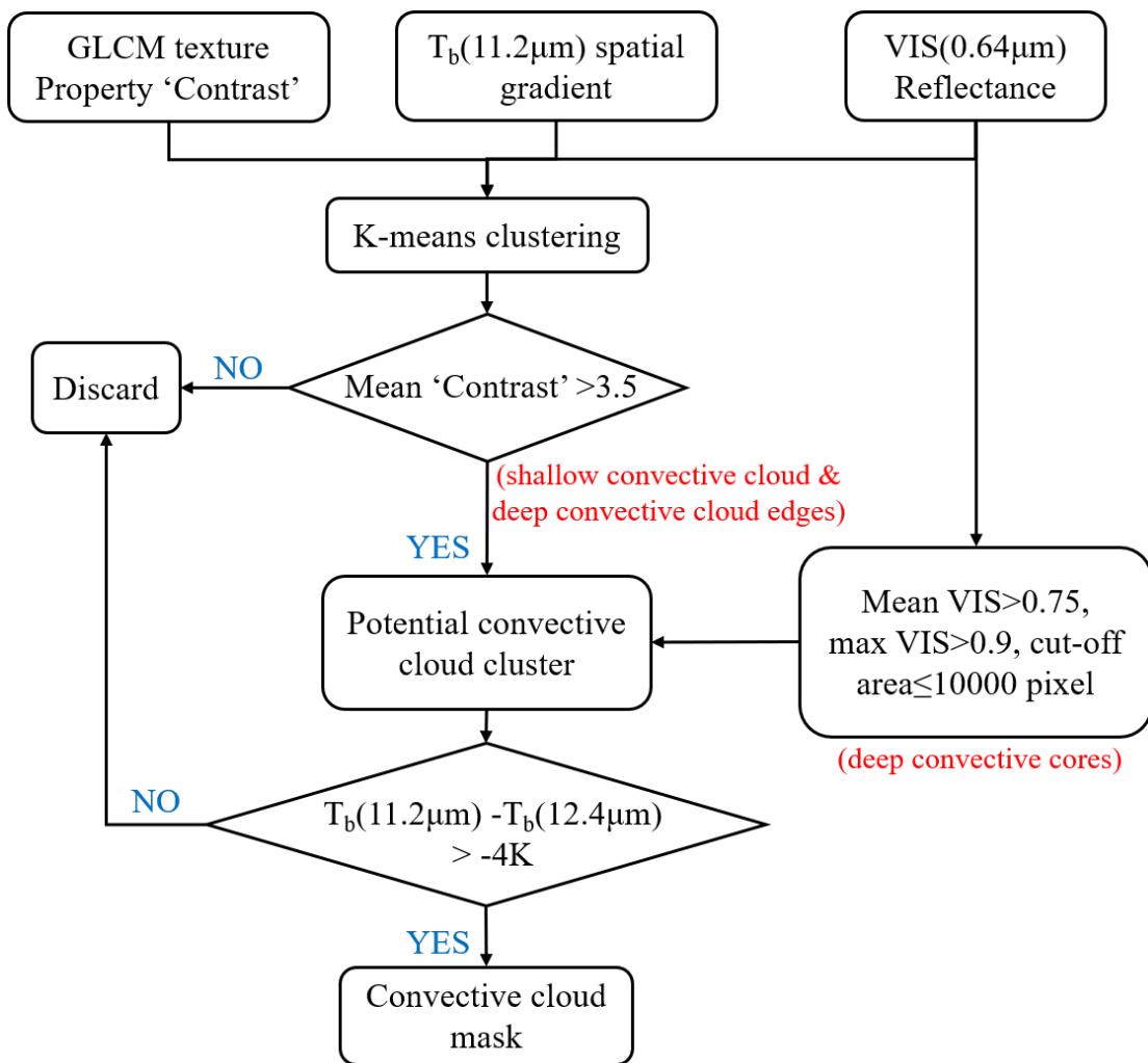
Figure 2. Flowchart of the convective cloud identification method.
