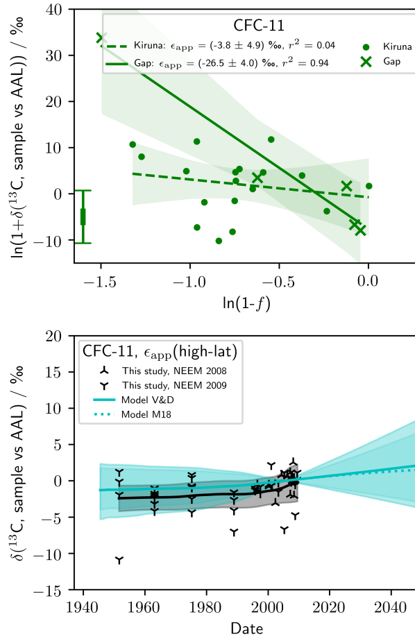
Figure D1. Rayleigh plot showing observations of \delta^{13}\text{C} (C, CFC-11), and derived \epsilon_{\text{app}}(\text{CFC-11, high-lat}) and \epsilon_{\text{app}}(\text{CFC-11, mid-lat}) (top). Also shown is measured and modelled \delta_{\text{T}}(\text{CFC-11}) (see Figure 4 and Section 2.5 for a description of the model). The model was forced with \epsilon_{\text{app}}(\text{CFC-11, high-lat}) . The errorbar in the bottom left corner of each graph shows the median repeatability of the reference gas measurements over the measurement days and the median error deriving from the fractional release factor.
