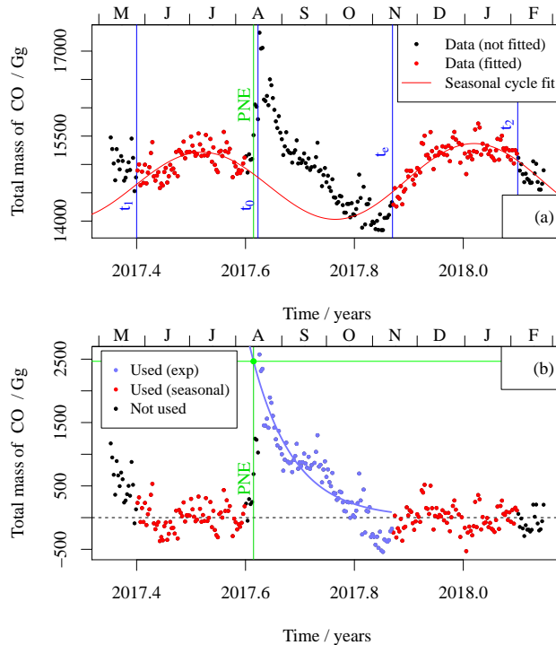
Figure 5. (a) Total mass of CO observed by MLS poleward of 27.5^\circ N and at altitudes between 215 hPa and 31 hPa. The four times t_1, t_0, t_e and t_2 are discussed in the text. The seasonal fit includes both annual and semiannual components; the annual component is much smaller in this case. (b) As (a), but with the seasonal fit subtracted from the data, and an exponential fitted to the measurements made after the fire. Both the exponential fit and the data used to construct it are shown in blue.
