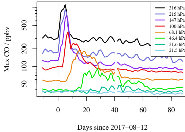
Figure 2. Time series of maximum CO values observed polewards of 27.5^\circ N. The values shown are averages of the ten highest observed values on each day between 27.5^\circ N and 83^\circ N. A 3-day smoothing has been applied to each curve.
