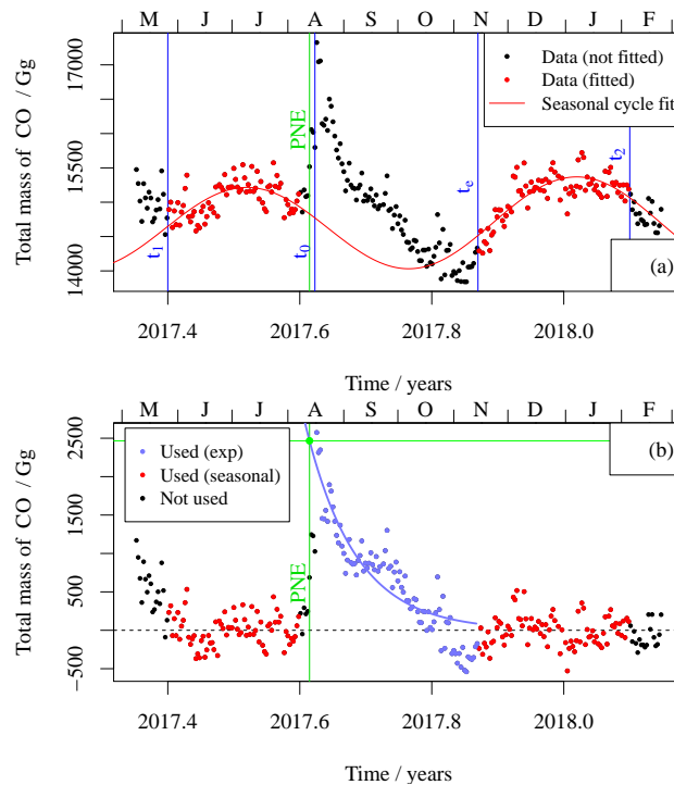
Figure 5. (a) Total mass of CO observed by MLS poleward of 27.5° N and at altitudes between 215 hPa and 31 hPa. The four times t_1, t_0, t_e and t_2 are discussed in the text. The seasonal fit includes both annual and semiannual components; the annual component is much smaller in this case. (b) As (a), but with the seasonal fit subtracted from the data, and an exponential fitted to the measurements made after the fire. The vertical dashed orange line marks 16 August 2017: Both the time of exponential fit and the earliest data used to construct it are shown in the exponential fit blue.
