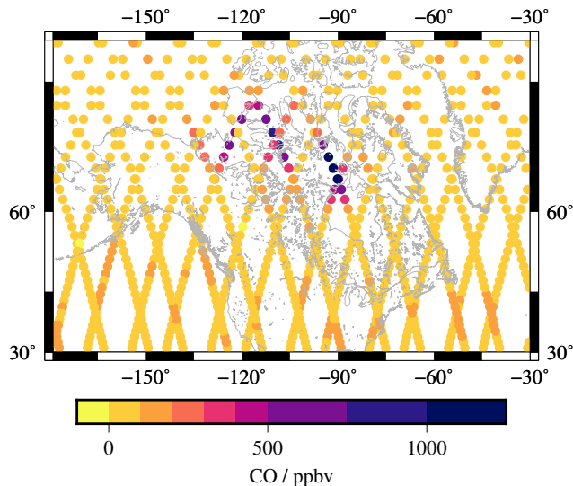
Figure 1. MLS measurements of CO (in ppbv) at 215 hPa ( \approx 11 km altitude) on 14-15 14-15 August 2017. These are the first two days after the PNE on which MLS observed the enhanced CO values.
