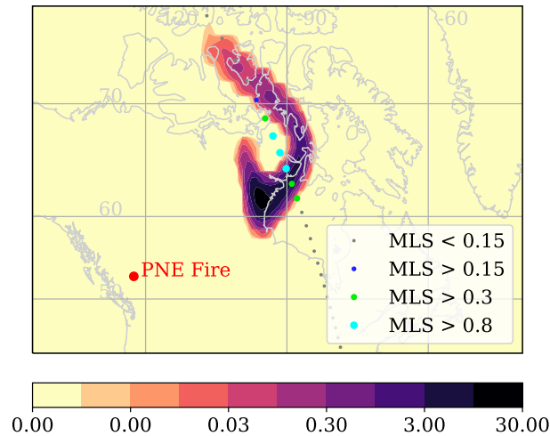
Figure 11. FLEXPART CO mixing ratio in ppmv at altitude 12 km on 15 August 2017 at 18:00, with 00. Dots show the location of MLS CO mixing ratio (also in ppmv) profiles from an orbit at a matching time. The dots are coloured to show where MLS CO, interpolated to an altitude of 12 km, is below 0.15 ppmv, and where it exceeds 0.15, 0.3 and 0.8 ppmv.
