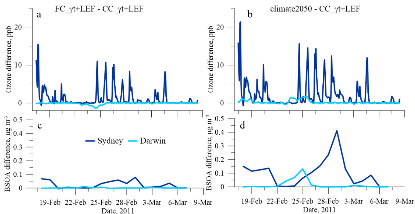
Figure 6. Differences in hourly ozone (panels a and b) and biogenic secondary organic aerosol (panels c and d) at Sydney and Darwin during SPS1 duration. Left panels (a and c) show \text{FC}_{\gamma\text{T}+\text{LEF}} - \text{CC}_{\gamma\text{T}+\text{LEF}} whilst right panels (b and d) show \text{climate2050} - \text{CC}_{\gamma\text{T}+\text{LEF}} .
