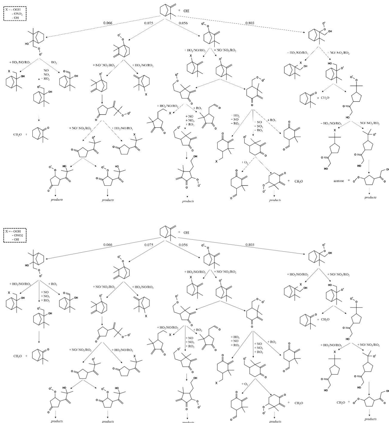
Figure 3: Initial oxidation pathways of camphene oxidation with OH as represented in GECKO-A ( inorganic products are not shown ).
