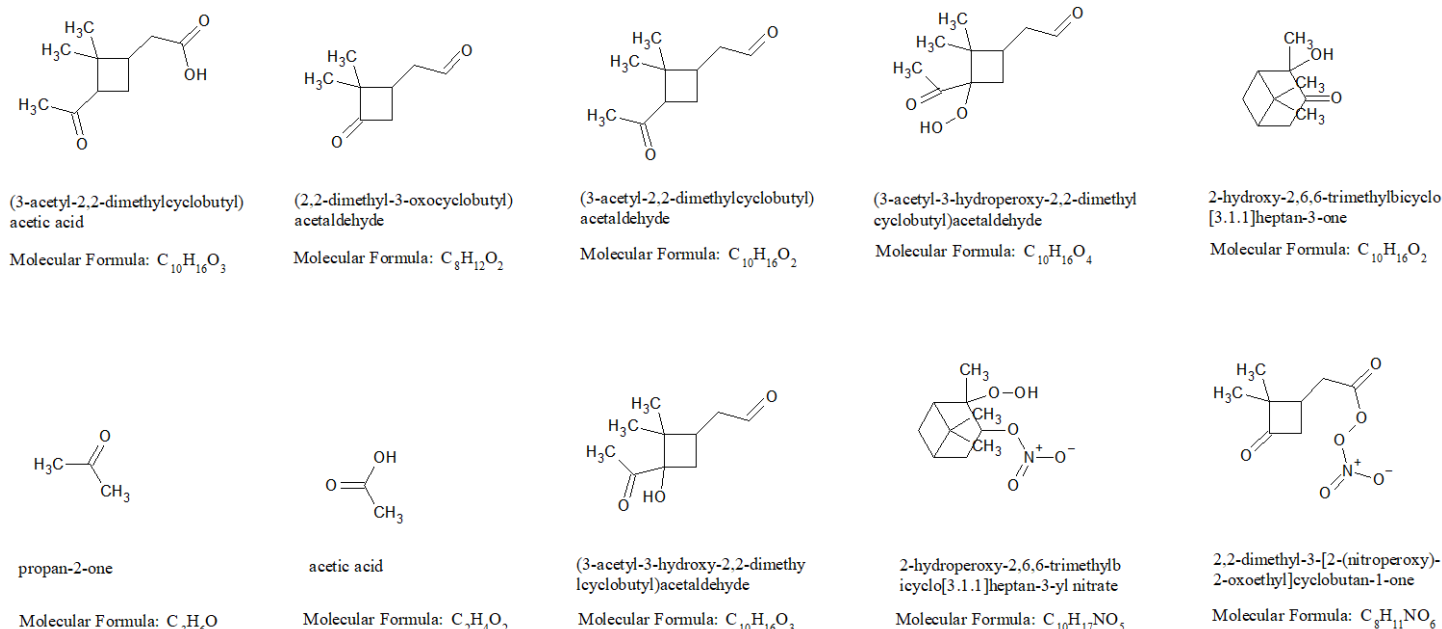
Figure 6a: Top 10 gas-phase products from \alpha -pinene dark ozonolysis at the end of the low hydrocarbon (DO_LHC) simulations .
