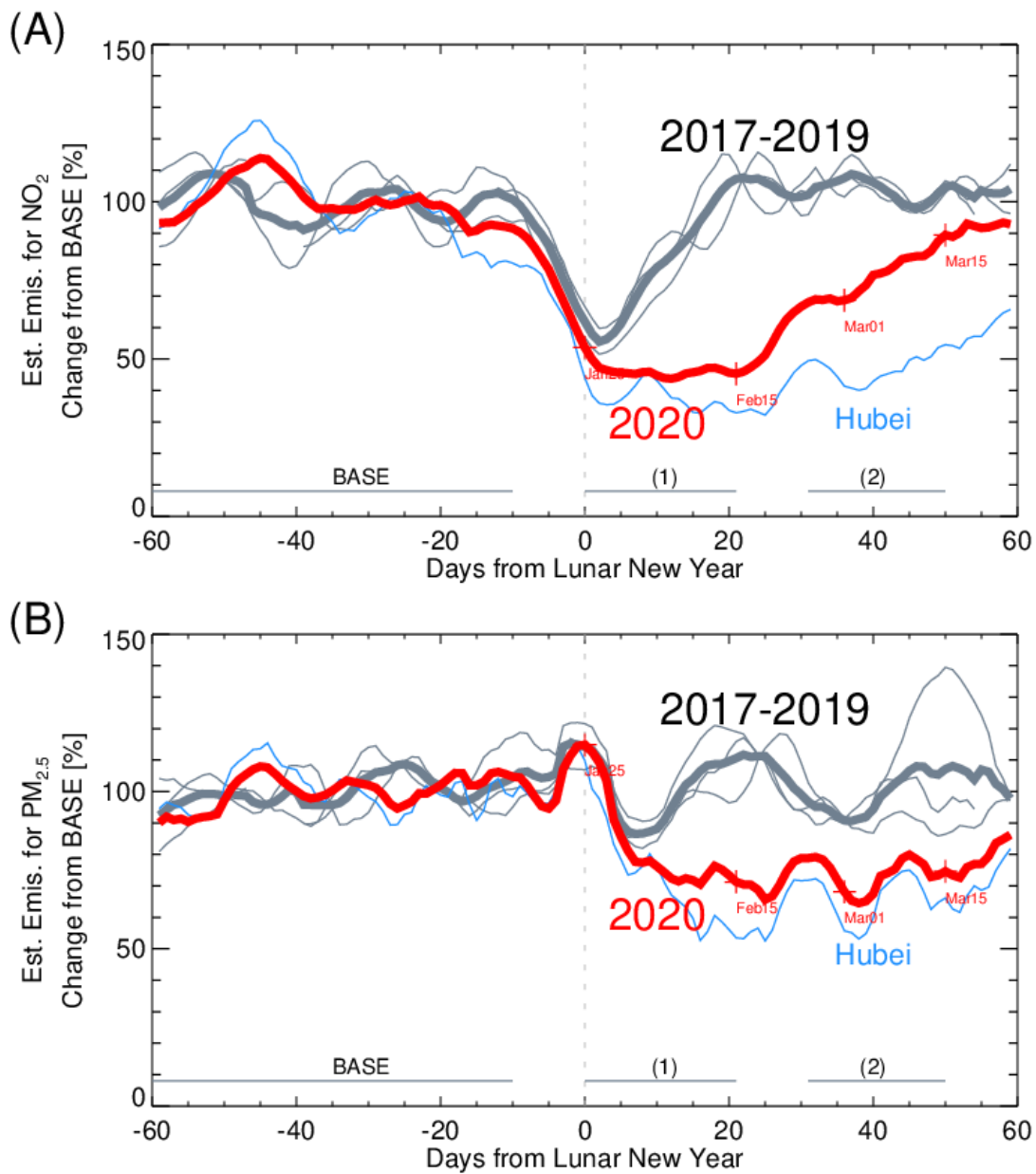
555 Figure 2. Time series of estimated emissions for (a) \text{NO}_2 and (b) \text{PM}_{2.5} using 1,332 surface monitoring sites across China. The gray lines indicate 2017–2019 variations, with their average in the thick gray line, whereas the red line indicates the 2020 variation. The blue line indicates the 2020 variations in Hubei province (46 sites). BASE is used as the pre-LNY period, and (1) and (2) denote the period of maximum impact and the recovery period, respectively.
