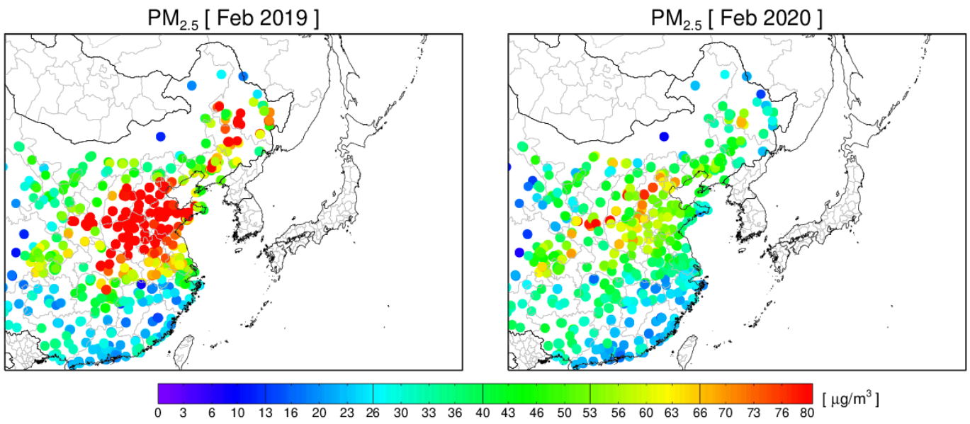
550 Figure 1. Geographical coverage of modeling domain and surface-monitoring sites. Monthly mean surface PM 2.5 concentrations in February 2019 and February 2020 are shown.
