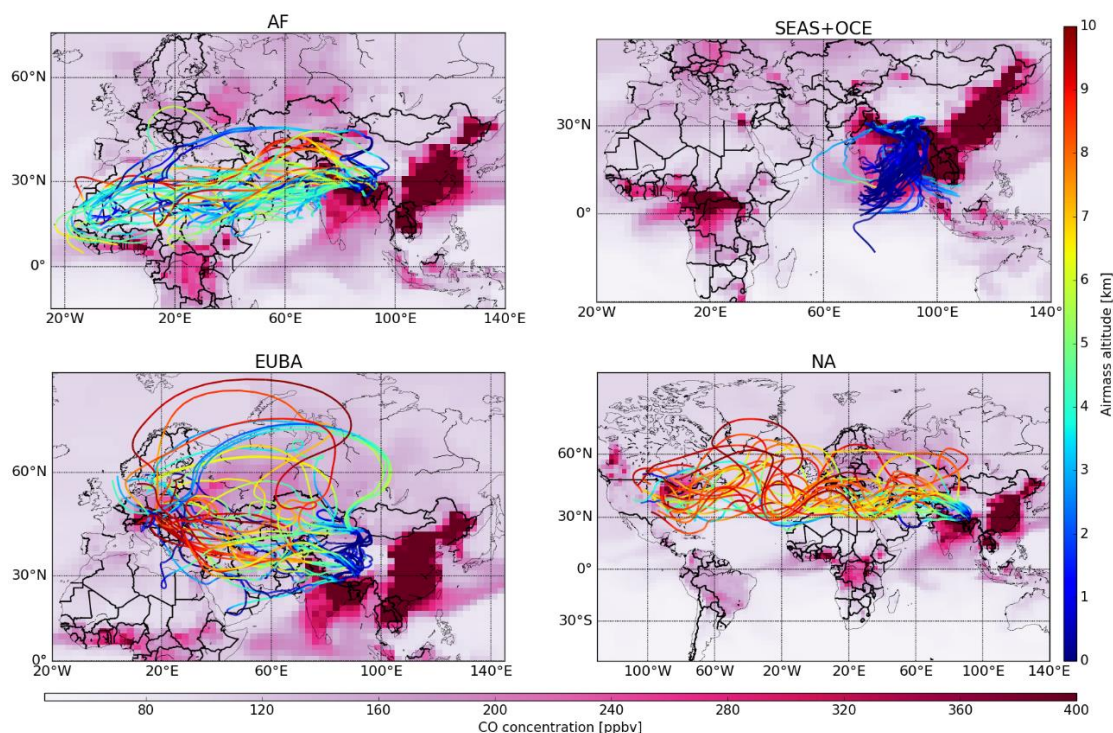
Fig. 11. Travel trajectories of polluted air masses originated in AF (SON/DJF), SEAS & OCE (MAM/JJA), EUBA (SON/DJF), and NA (SON/DJF) that reached Naqu ( 31.5^\circ\text{N} ) through long range transport. For clarity, only few trajectories are selected for demonstration. Travel times are 13, 7, 10, and 14 days, respectively. Global surface CO distribution based on GEOS-Chem simulations are shown for 13, 7, 10, and 14 days prior to the arrival time, respectively. The deeper the color, the higher the CO concentration.
