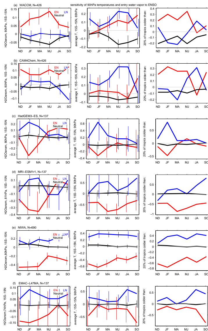
Figure 2. (left) Tropical water vapor from 15S-15N near 80hPa in each of the 6 CCMI models considered here from the late fall as the event is developing through the following summer for (red) El Niño, (blue) La Niña, (black) neutral ENSO. 5% confidence intervals on the anomalous response based on a two-tailed Student-t test are shown. (middle) response of zonally averaged temperature anomalies from 15S-15N near 90hPa for each model. (right) evolution of the temperature of the coldest 20% of the tropics at 90hPa for each model in each ENSO phase as compared to the model's climatology.
