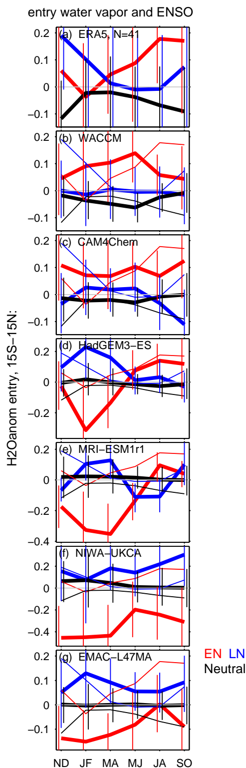
Figure 5. (a) As in Figure 2a but for ERA5, (b-g) As in Figure 2 but subsampling the model output for each model to match the sample size in observations for each ENSO phase. The uncertainty (marked with vertical lines) of the model response is determined by the Monte Carlo subsampling as described in the text.
