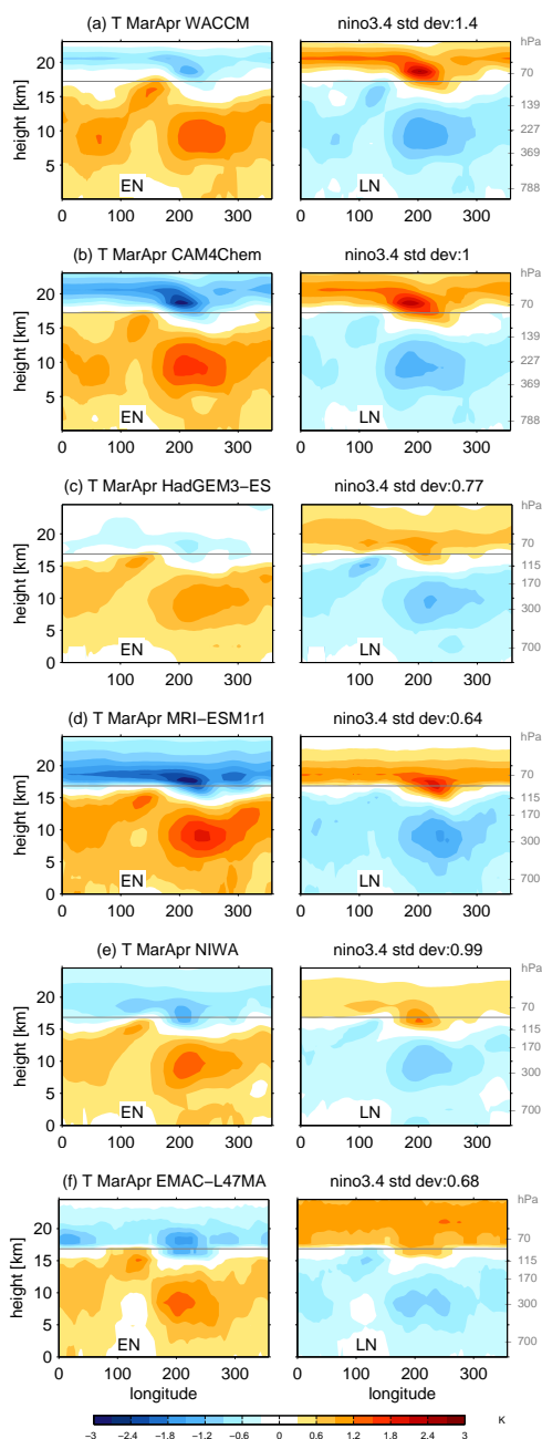
Figure 3. Longitude versus height cross section of the 15S-15N temperature anomalies during (left) El Niño, (right) La Niña in each of the CCM1 models
