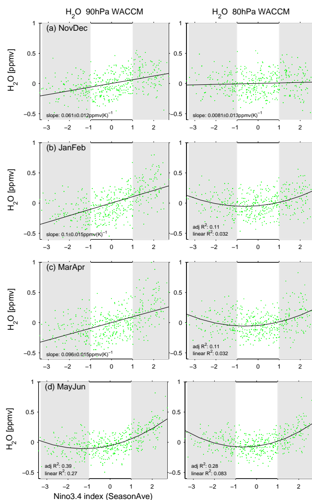
Figure 1. Anomalous 90hPa and 80hPa water vapor in WACCM as compared to the value of the Nino3.4 index for (a) November and December; (b) January and February; (c) March and April; (d) May and June. Each dot corresponds to one model-year. When a polynomial fit better describes the dependence on ENSO than a linear fit, we show the R^2 for a linear fit and adjusted R^2 for the polynomial fit (see section 2.2). Otherwise we show a linear least-squares best fit in each panel.
