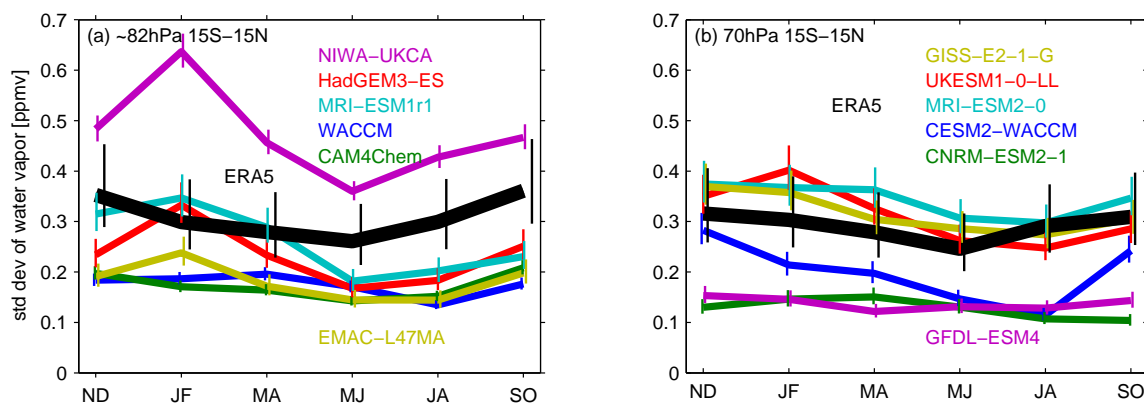
Figure 6. Standard deviation of tropical entry water vapor for each model in (a) CCMI near 82hPa and (b) CMIP6 at 70hPa, and for ERA5 water vapor (thick line). The vertical lines denote 95% confidence bounds as discussed in the text.
