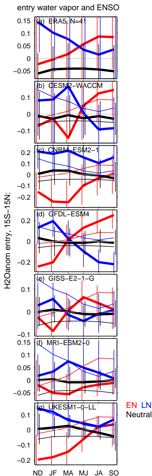
Figure 7. (a) As in Figure 2a but for ERA5, (b-g) As in Figure 2 but subsampling the model output for six CMIP6 models with interactive chemistry to match the sample size in observations for each ENSO phase for water vapor at 70hPa. The uncertainty (marked with vertical lines) of the model response is determined by the Monte Carlo subsampling as described in the text.
