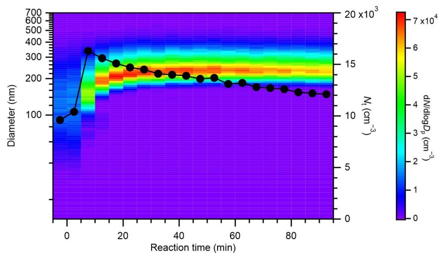
Figure S6: The evolution of particle number-size distributions (image plot) and total particle number concentrations ( N_t ) during a typical experiment run (Exp. No. 27).
