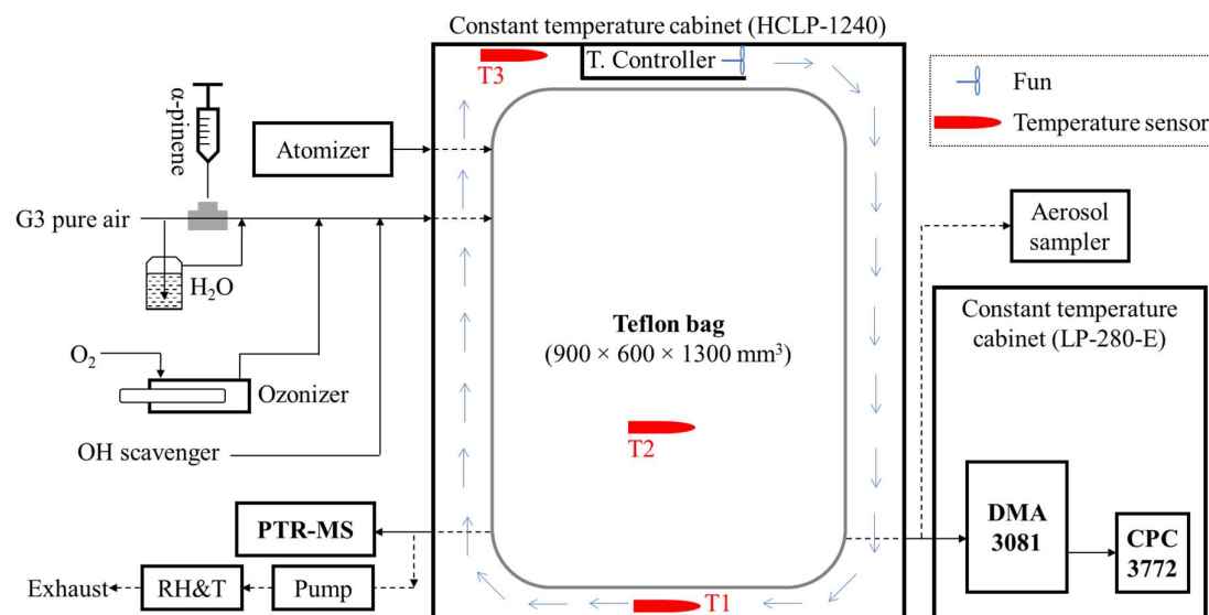
130 Figure S1: A schematic of the compact chamber system. Arrows in light blue indicate the general air circulation inside the HCLP-1240. PTR-MS, proton transfer reaction mass spectrometry; DMA, differential mobility analyser; CPC, condensation particle counter; T. Controller, temperature controller; T1, temperature near the floor of the HCLP-1240; T2, temperature inside the Teflon bag; T3, temperature measured by the T. Controller.
