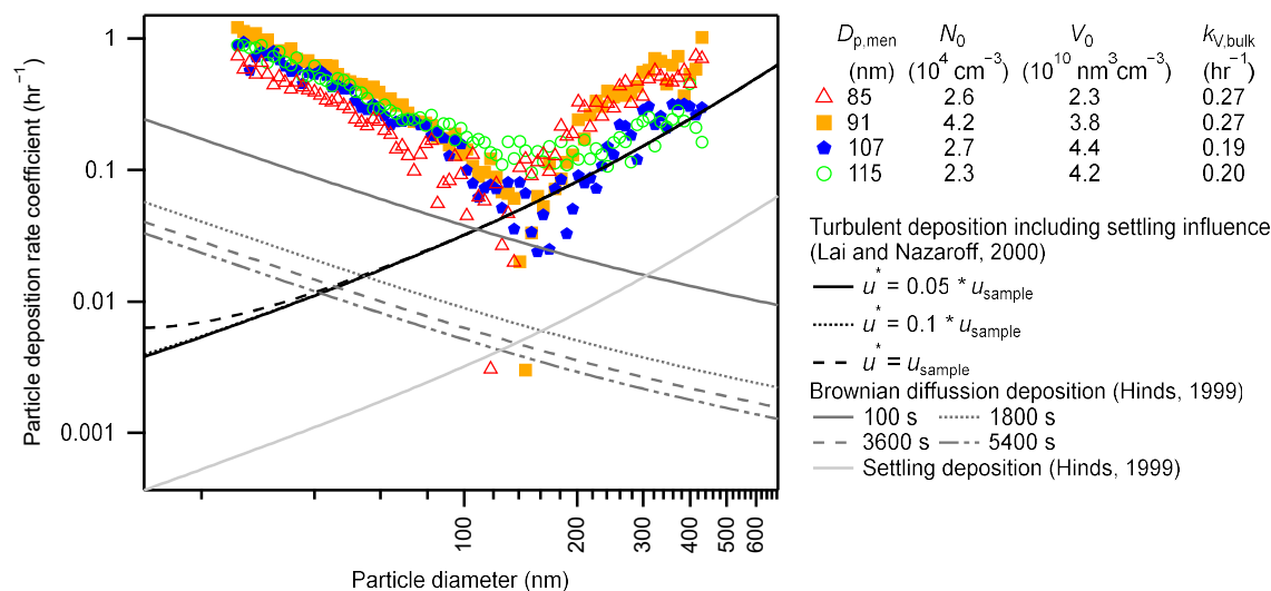
Figure S4: Size-resolved wall loss rates measured under a 17–23 % RH range at a temperature of 298 K (color markers) and model simulations of wall-loss caused by different mechanisms (black and grey curves). The legend of the measured data indicates the mean particle diameter during the wall loss rate measurement ( D_{p,mean} ), the initial total particle number ( N_0 ) and volume ( V_0 ) concentrations, and the bulk volume wall-loss constant ( k_{V,bulk} ). Model simulations of turbulent deposition based on Lai and Nazaroff (2000) considered the influence of gravitational settling deposition but neglected the influence of Brownian diffusion; simulations when the friction velocity ( u^* ) was 5, 10, and 100 % of the sample velocity ( u_{sample} , 1.2 \times 10^{-5} \text{ m s}^{-1} ) are presented. Simulations of Brownian diffusion deposition and settling deposition assuming still state of Brownian diffusion deposition and settling deposition. For the former, the deposition rate coefficients at 100, 1800, 3600, and 5400 s after an assumed still state have begun are presented.
