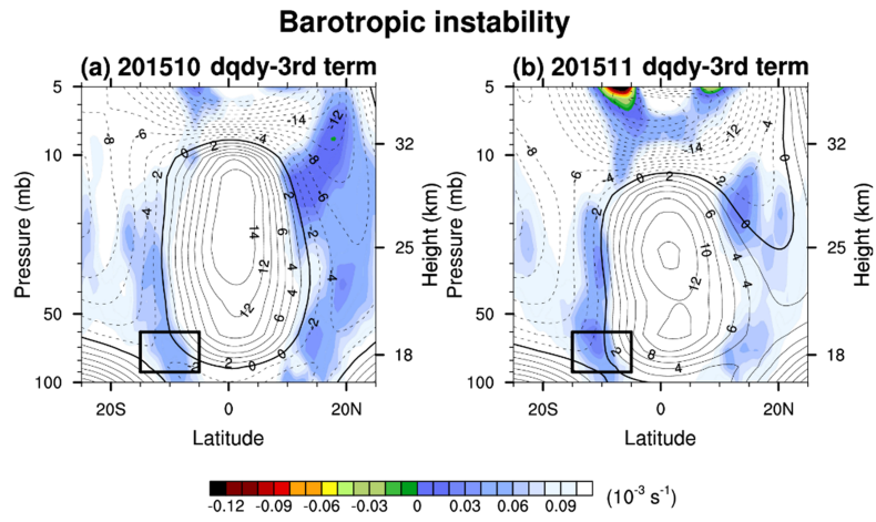
Fig. 2. Figure A1. The same as Figs. 8a–b but for q_{\phi} excluding the third term in the righthand side of Eq. (3).
