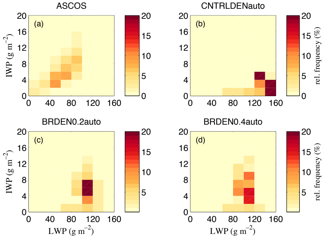
Figure 8: Relative frequency distribution of IWP ( g m -2 ) as a function of LWP ( g m -2 ) for (a) ASCOS, (b) CNTRLDENauto, (c) BRDEN0.2auto and (d) BRDEN0.4auto (see Table 3). Cloud ice-to-snow autoconversion is active in all model simulations. Collisional break-up is included only in panels (c-d) with the cloud ice/snow rimed fraction set to (c) 0.2 and (d) 0.4. In all simulations a dendritic cloud ice habit is assumed.
