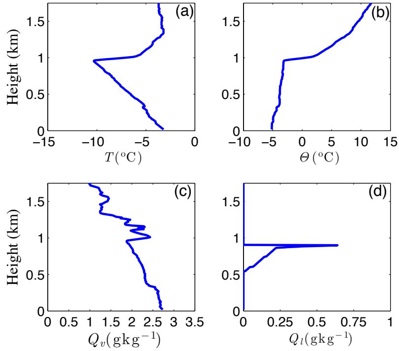
Figure 1: Radiosonde profiles of (a) temperature ( T ), (b) potential temperature ( \Theta ), and (c) specific humidity ( Q_v ) used to initialize the LES. The profile of cloud liquid ( Q_l ) in panel (d) is integrated from radiometer measurements.
