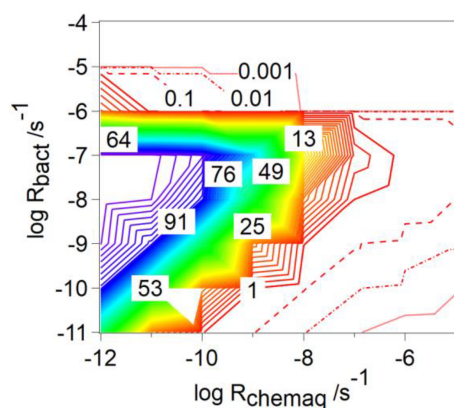
Figure 3. Relative contribution of bacteria to the total loss rate of CCN-derived organics ( fr_{bact} , Eq. 7) as a function of R_{bact} [ s^{-1} ] and R_{chemaq} [ s^{-1} ].
