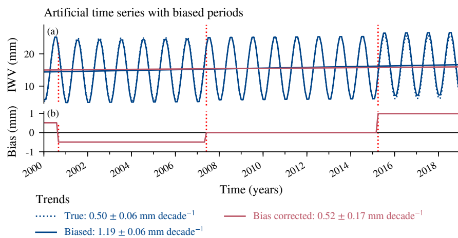
Figure 2. Artificial time series (a) and added biases (b). The linear trends for the true (unbiased) data, the biased data and the bias corrected data are given.
