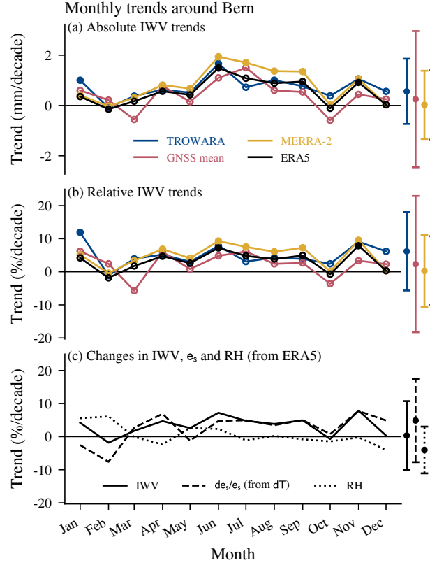
Figure 6. Trends of IWV for different months for TROWARA in Bern, GNSS stations close to Bern (arithmetic mean), and reanalysis grids (MERRA-2 and ERA5) at Bern. Uncertainty bars show the maximum range of 2\sigma uncertainties of each dataset. Filled dots represent trends that are significantly different from zero at 95% confidence interval. Monthly IWV trends are given in panel (a) as absolute trends in mm per decade and in panel (b) as relative trends in percent per decade. Panel (c) presents again the monthly IWV trends from ERA5, and in addition the relative humidity (RH) trends and the theoretical change in saturation vapour pressure e_s due to the observed temperature change from ERA5 data (both averaged below 500 hPa).
