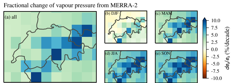
Figure 14. Same as Fig. 13 but using MERRA-2 temperature data averaged below 500 hPa (1995-2018).
