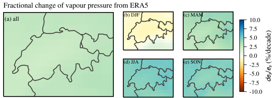
Figure 13. Fractional change of water vapour pressure ( e_s ) derived from temperature trends from ERA5 (1995-2018) for the whole year (a) and different seasons ((b) to (e)) . The temperature data have been averaged below 500 hPa.
