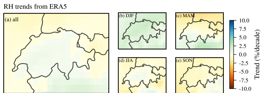
Figure 15. Relative humidity (RH) trends from ERA5 reanalysis data in Switzerland from 1995 to 2018 (averaged below 500 hPa) for the whole year (a) and for the different seasons ((b) to (e)).
