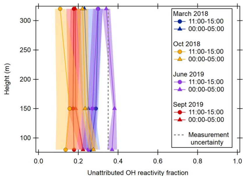
Figure S2. Unattributed OH reactivity fraction profiles for noon- and nighttime in each measurement period. The shaded areas represent the standard deviation. The measurement uncertainty given is the average over all observation periods. Note that the unattributed fraction is usually below the measurement uncertainty.
