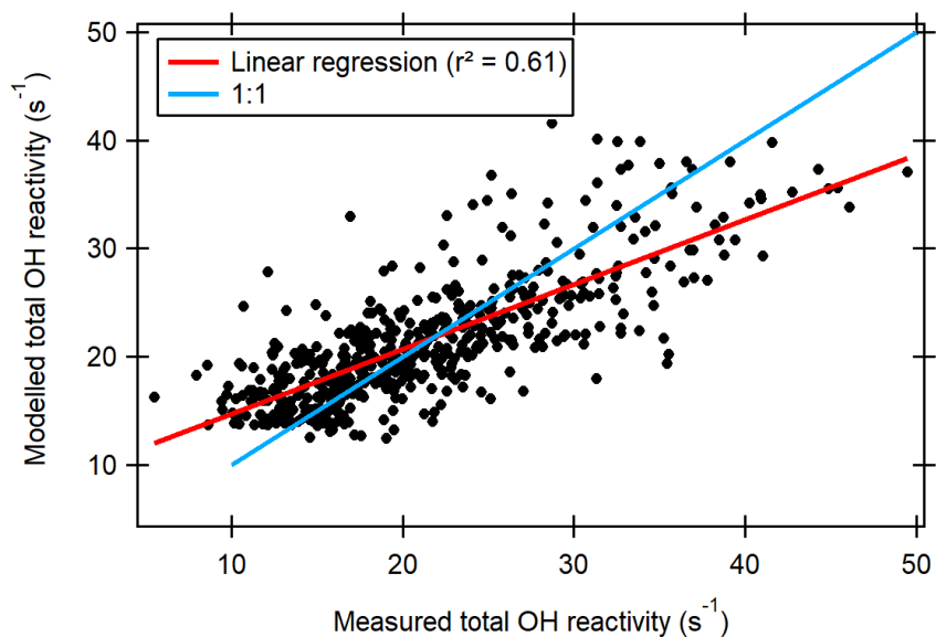
10 Figure S4. Modelled total OH reactivity from the temperature-dependent parameterization (Sect. 3.3.1) vs. measured total OH reactivity. Linear regression: y = 8.7 + 0.6x , r^2 = 0.61 .
