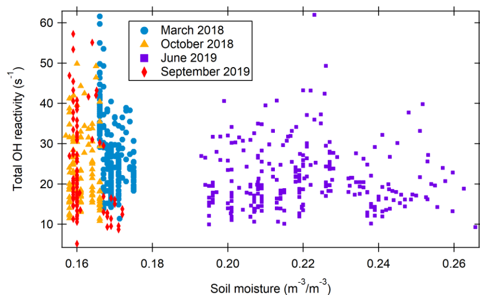
Figure S1. Soil moisture and total OH reactivity in hourly time resolution for the four measurement periods.
