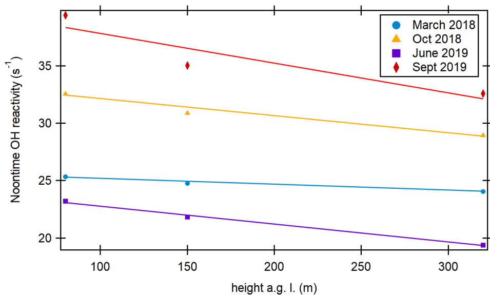
5 Figure S3. Campaign average noontime total OH reactivities as a function of height with linear regressions for gradient determination. The results of the linear regressions were: March 2018: R = -0.005 \cdot h + 25.7 ; October 2018: R = -0.015 \cdot h + 34.0 ; June 2019: R = -0.016 \cdot h + 24.3 ; September 2019: R = -0.026 \cdot h + 40.4 .
