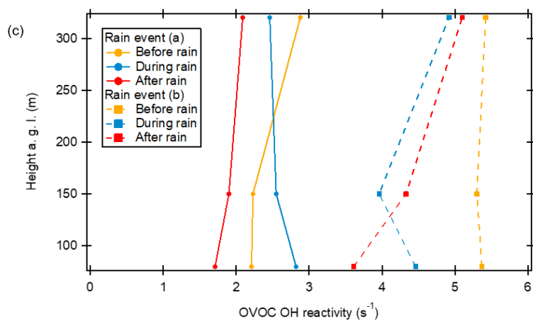
5 Figure S5. Timeseries of meteorological parameters (wind speed at 320 m, precipitation at 320 m, PAR at 80 m), OVOC OH reactivity and acetaldehyde mixing ratios around (a) a daytime rain event and (b) an evening rain event. (c) Vertical profiles of OVOC-attributed OH reactivity for two rain events.
