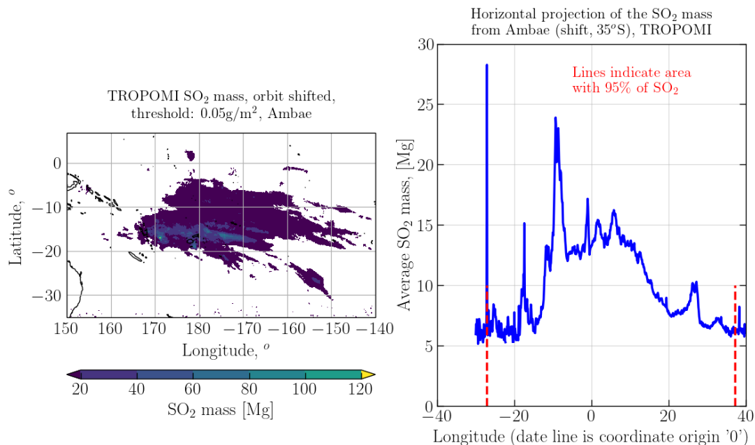
Fig. 1. Left: average of the SO 2 mass over all batches. Right: the time averaged SO 2 mass was averaged over each latitude to estimate the expansion of the plume. The red dotted lines mark an area that contain
