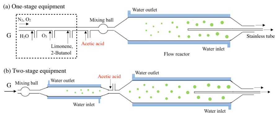
765 Figure 1: Diagram of the experimental setup. The (a) one-stage and (b) two-stage apparatuses are used to investigate the first- and second-generation oxidation. The green circles represent the process of SOA growth.
