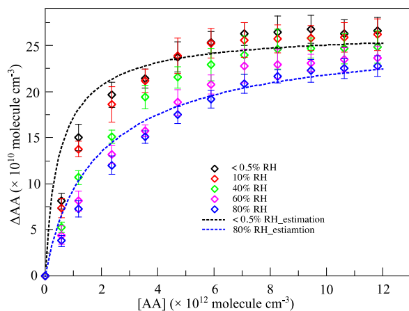
770 Figure 2: The variations of the consumption of acetic acid ( \Delta AA ) with the concentration of acetic acid ( [AA] ) at different relative humidity (RH) in the first-generation oxidation. Scatters: measured \Delta AA ; Black line: estimated \Delta AA at < 0.5% RH; Blue line: estimated \Delta AA at 80% RH.
