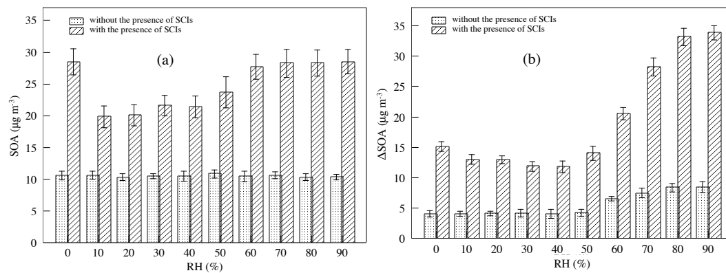
775 Figure 3: Impact of the presence of SCIs on (a) SOA mass concentration (SOA) in the first-generation oxidation and (b) the increment of SOA mass concentration ( \Delta\text{SOA} ) in the second-generation oxidation at different relative humidity (RH).
