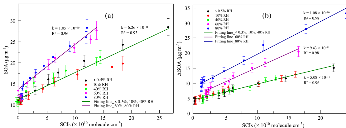
Figure 6: (a) The dependence of SOA mass concentration (SOA) on the amount of SCIs at different relative humidity (RH) in the first-generation oxidation. (b) The dependence of SOA mass concentration increment ( \Delta\text{SOA} ) on the amount of SCIs at different relative humidity (RH) in the second-generation oxidation.
