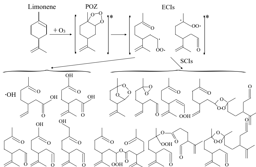
Figure 7: Reaction scheme of limonene ozonolysis.
