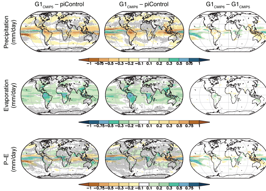
Figure 9. Precipitation (top), evaporation (middle), and precipitation minus evaporation (P-E; bottom) change from preindustrial for the CMIP5 (left) and CMIP6 (middle) ensembles, as well as the ensemble differences (right). All shaded values are ensemble means. Lack of stippling in the left and middle panels indicates agreement on the sign of the values across at least 75% of the models.
