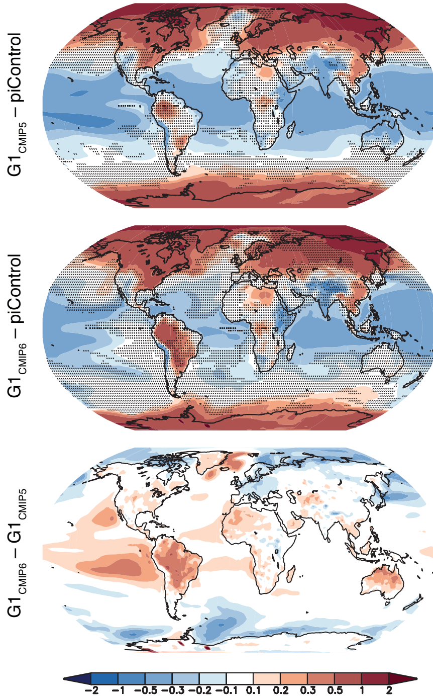
Figure 8. Ensemble average temperature changes (K) for G1 (as compared to the preindustrial control) for CMIP5 (top) and CMIP6 (middle), as well as their difference ( G1_{\text{CMIP6}} minus G1_{\text{CMIP5}} , bottom panel). In the top two panels, stippling indicates regions where fewer than 75% of the models in their respective ensembles agree on the sign of the response.
