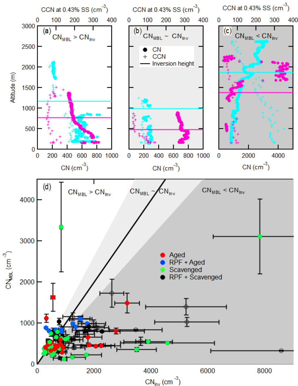
845 Figure 7. Vertical profiles of CN and CCN at 0.43% supersaturation corresponding to (a) elevated CN concentrations in the MBL, (b) well-mixed CN profiles and (c) elevated CN concentrations aloft. The cyan and magenta points in (a-c) represent 2 different vertical profiles. (d) Comparison of CN measured in the surface coupled MBL and decoupled layer or FT. Error bars represent standard error. Empty markers do not have a corresponding CCN_{0.3} measurement.
