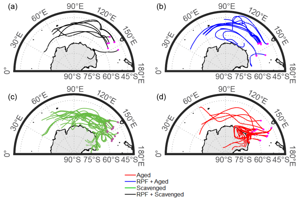
Figure 3. Five-day HYSPLIT back trajectories starting from MBL legs (at 50-500 m amsl., magenta points) for each particle regime.
