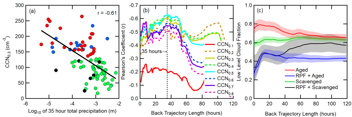
Figure 4. (a) Correlation of MBL CCN_{0.3} and total precipitation that occurred along a 35-hour HYSPLIT back trajectory. Marker colors correspond to legend in (c). (b) CCN and back trajectory total precipitation correlation coefficient as a function of back trajectory length. Vertical dashed line indicates peak in correlation with CCN_{0.3} at 35-hours. (c) Particle regime averaged ERA5 low-level cloud fraction over the five-day back trajectory. Shaded areas represent one standard error.
