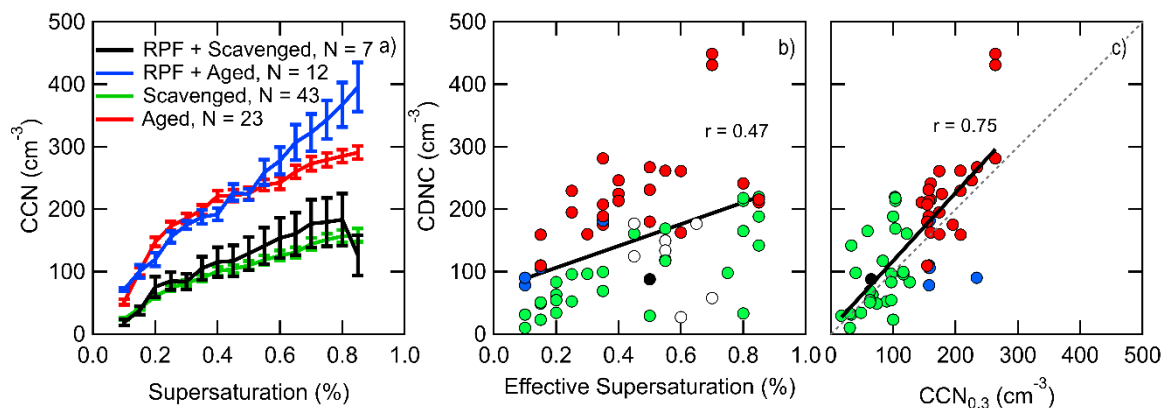
Figure 2. (a) Mean MBL CCN spectra for each regime. The number of samples (N) at each supersaturation of the CCN spectra varied from the number of samples in the legend because occasionally CCN spectra scans were not fully completed by the end of the MBL leg. Error bars represent the standard error ( \sigma/\sqrt{N} ). Correlations of measured CDNC with (b) calculated effective supersaturation and (c) measured MBL CCN 0.3 . Empty points did not have a corresponding CCN 0.3 or CN measurement. Solid lines in (b) and (c) represent linear fits and the dashed line in (c) represents the 1:1 line.
