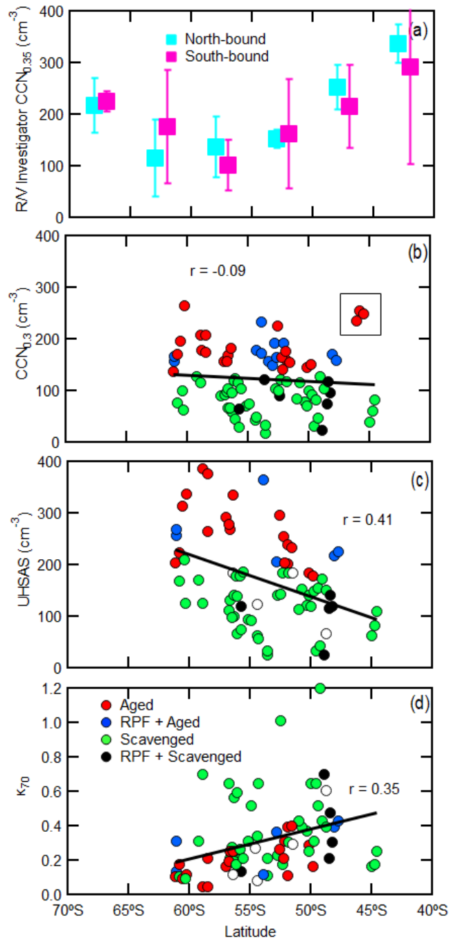
Figure 5. (a) 5^\circ latitude bin averaged CCN_{0.35} from the R/V Investigator . Correlation of latitude to (b) HIAPER GV CCN_{0.3} (c) total particle concentration with D_p > 0.07 \mu m (UHSAS) and (d) \kappa derived at 0.07 \mu m . White points in (c) and (d) did not have a corresponding CCN_{0.3} or CN measurement. Pearson's coefficient for (b) is r = -0.27 when excluding the three outliers at \sim 46^\circ S highlighted in the black square.
