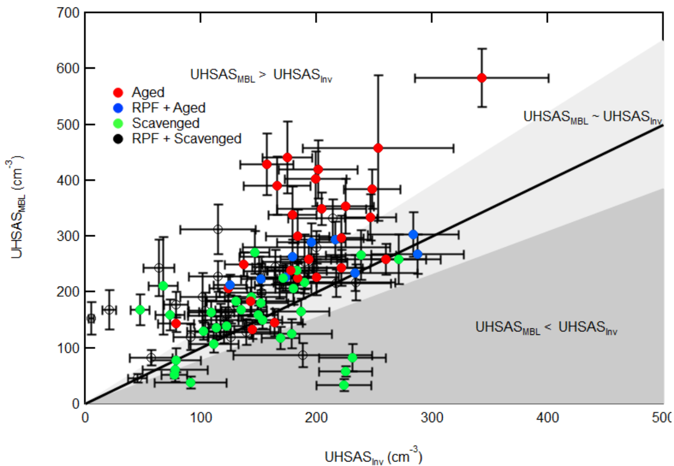
850 Figure 8. Comparison of UHSAS concentrations ( D_p > 0.07 \mu\text{m} ) measured in the surface coupled MBL and decoupled layer or FT. Error bars represent standard error. Empty markers do not have a corresponding \text{CCN}_{0.3} measurement.
