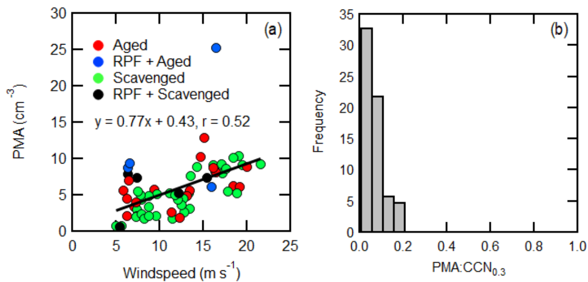
Figure 6. (a) Correlation of estimated PMA concentration and wind speed, and (b) the fraction of PMA accounting for CCN 0.3 for MBL legs. Exclusion of the outlier in (a) increases the Pearson's Coefficient to 0.59 .
