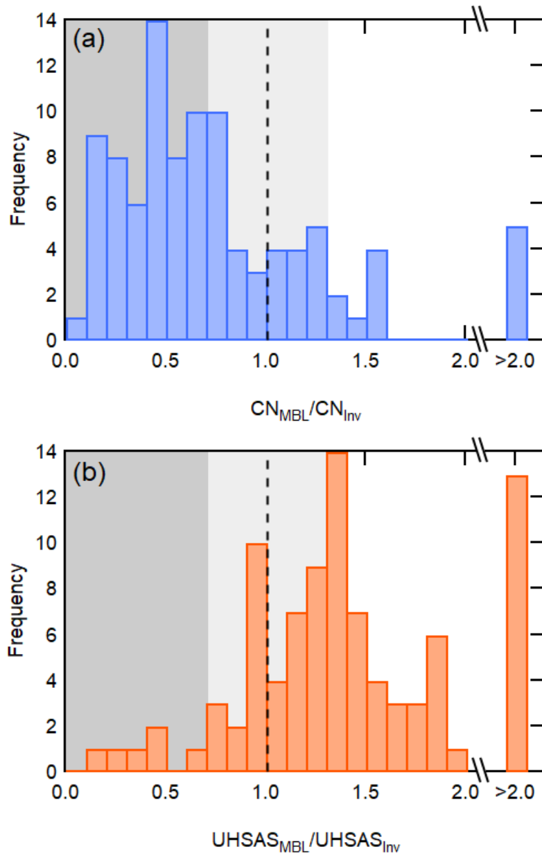
Figure 9. Histogram of (a) CN_{MBL}/CN_{Inv} from Figure 7 and (b) UHSAS_{MBL}/UHSAS_{Inv} from Figure 8.
