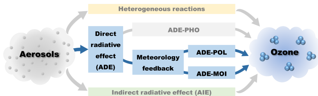
500 Figure 1: The mechanism of aerosols affecting ozone. The main topic of this paper has been marked as blue lines and blocks.
