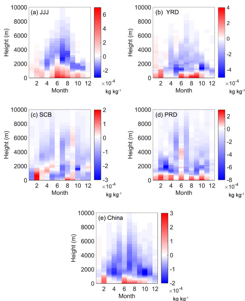
520 Figure 6: Monthly changes of specific humidity in (a) Jing-Jin-Ji, (b) Yangtze river delta, (c) Sichuan Basin, (d) Pearl river delta, and (e) China due to aerosol direct radiative effect. Differences are calculated as the monthly mean of \text{EXP}_{\text{radon}} minus \text{EXP}_{\text{radoff}} .
