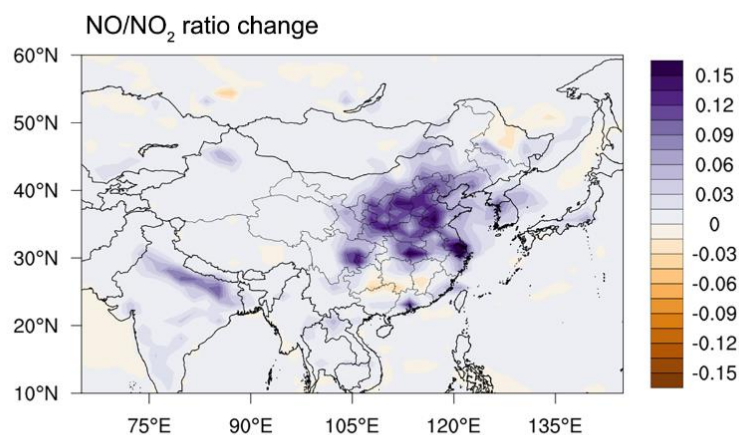
Figure 8: Annual average change of NO/NO 2 due to aerosol direct radiative effect. Differences are calculated as the annual mean of 530 EXP radon minus EXP radoff .
