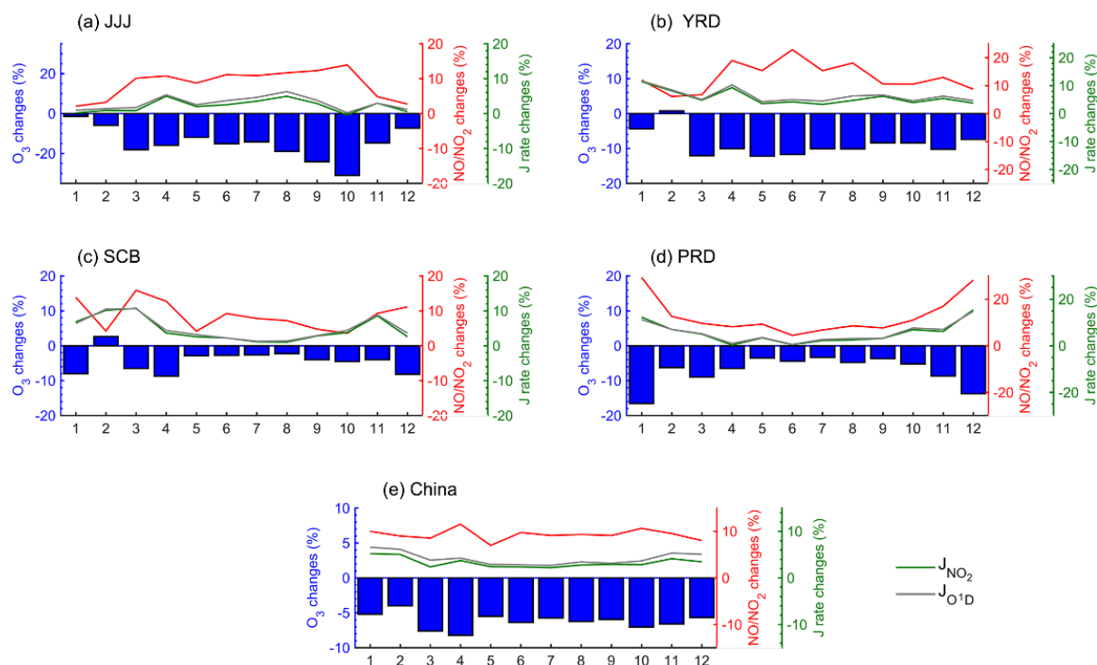
Figure 9: Monthly variation of O_3 concentration changes, NO/NO_2 ratio changes, J_{NO_2} and J_{O^1D} changes in (a) Jing-Jin-Ji, (b) Yangtze river delta, (c) Sichuan Basin, (d) Pearl river delta, and (e) China due to aerosol direct radiative effect. Differences are calculated as (EXP_{radon}-EXP_{radoff})/EXP_{radoff} , averaged over one year.
