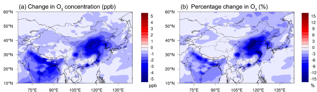
540 Figure 10: Annual average change of ozone due to aerosol direct radiative effect (a) absolute changes (ppb) are calculated as EXP_{radon} minus EXP_{radoff} , (b) percentage changes (%) are calculated as (EXP_{radon} - EXP_{radoff}) / EXP_{radoff} .
