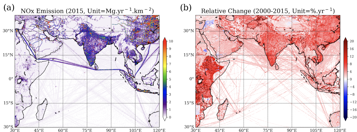
Figure 34. Same as Figure 23, but for NO x .
