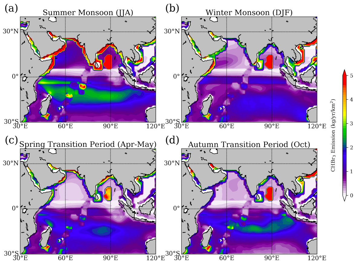
Figure 104. Bromoform ( \text{CHBr}_3 ) emission for (a) summer monsoon (June – August), (b) winter monsoon (December – February), (c) spring transition (April – May) and (d) autumn transition (October) periods based on static surface concentrations and ERA-Interim meteorology for 2014 (Fiehn et al., 2018).
