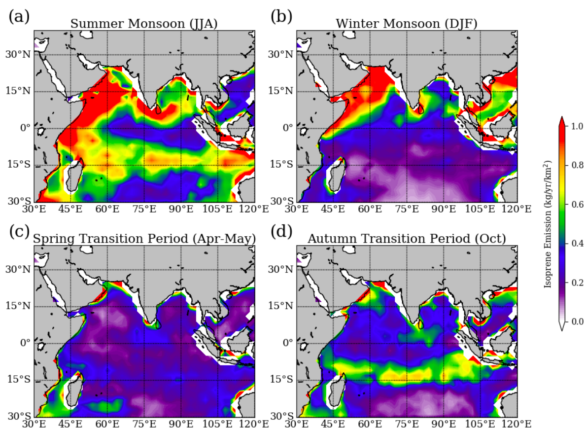
Figure 940. Same as Figure 89 but for isoprene from Booge et al. (2016).
