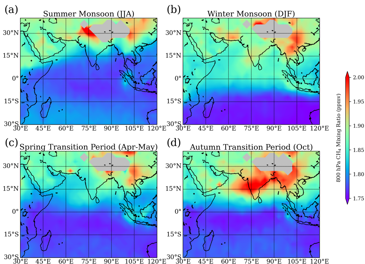
Figure 145. Methane (CH 4 ) mixing ratios at 800 hPa from GOSAT for (a) summer monsoon 2009 – 2014 (June – August), (b) winter monsoon 2009/2010 – 2014/2015 (December – February), (c) spring transition 2009 – 2014 (April – May) and (d) autumn transition 2009 – 2004 (October) periods.
