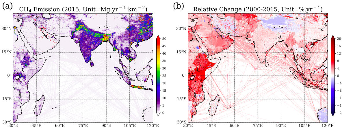
Figure 56. Annual mean CH 4 emissions for 2015 (a) and relative change with respect to 2000 (b) from EDGAR V5.0_GHG.
