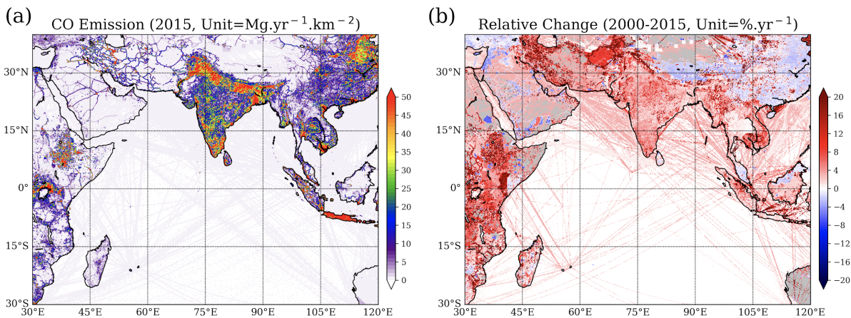
Figure 23. Annual mean \text{CO} emissions for 2015 (a) and relative change with respect to 2000 (b) from EDGAR V5.0_AP.
