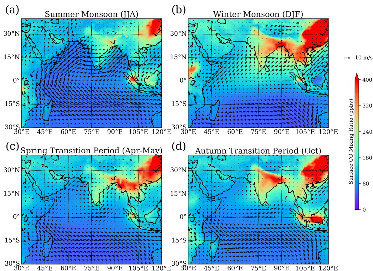
Figure 112. Surface carbon monoxide (CO) mixing ratios from MOPITT (coloured shading) and surface wind from ERA-Interim (black arrows) for (a) summer monsoon 2014 – 2018 (June – August), (b) winter monsoon 2014/2015 – 2018/2019 (December – February), (c) spring transition 2014 – 2018 (April – May) and (d) autumn transition 2014 – 2018 (October) periods.
