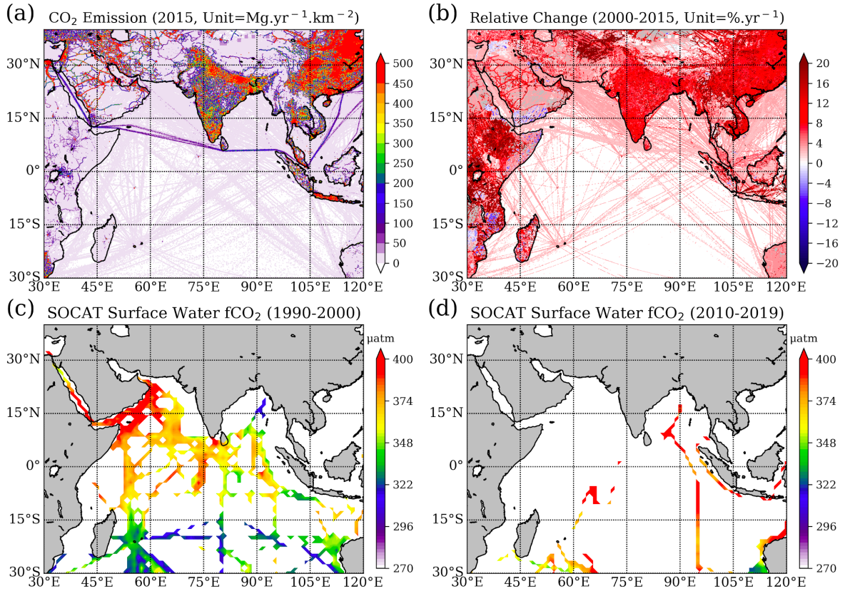
Figure 78. Annual mean CO 2 emissions for 2015 (a) and relative change with respect to 2000 (b) from EDGAR V5.0_GHG. Surface water fCO 2 observations (color shading, unit: \mu\text{atm} ) over the Indian Ocean for 1990–2000 (c) and 2010–2019 (d) from SOCATv2019 (Bakker et al., 2016).
