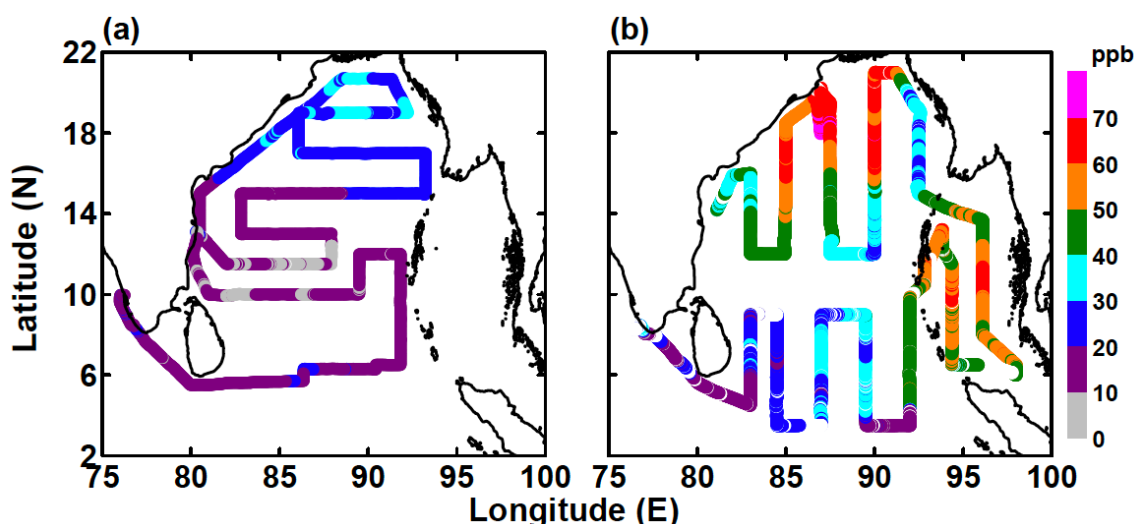
Figure 134. Surface ozone mixing ratios in the Bay of Bengal observed during a) boreal spring (March – April 2006, ICARB) and b) winter monsoon (December – January 2009, ICARB). From David et al., 2011, copyright 2011, reproduced with permission.
