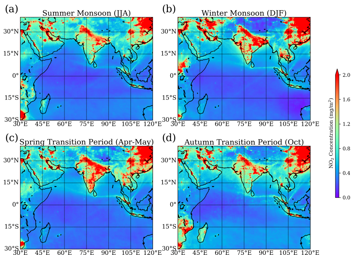
Figure 123. Tropospheric nitrogen dioxide (NO 2 ) column from TROPOMI for (a) summer monsoon 2019 (June – August), (b) winter monsoon 2018/2019 (December – February), (c) spring transition 2019 (April – May) and (d) autumn transition 2019 (October) periods.
