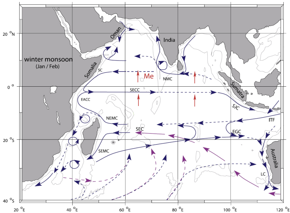
Figure S1. Schematic representation of identified oceanic currents during the summer monsoon (a) and winter monsoon (b). Current branches indicated are the South Equatorial Current (SEC), South Equatorial Countercurrent (SECC), Northeast and Southeast Madagascar Current (NEMC and SEMC), East African Coastal Current (EACC), Somali Current (SC), Southern Gyre (SG) and Great Whirl (GW) and associated upwelling wedges (green shades), Southwest and Northeast Monsoon Currents (SMC and NMC), South Java Current (SJC), East Gyrar Current (EGC), and Leeuwin Current (LC). The subsurface return flow of the supergyre is shown in magenta. Depth contours shown are for 1000 m and 3000 m (grey). Updated representations are from SMC01; red vectors (Me) show directions of meridional Ekman transports. ITF indicates Indonesian Throughflow (from Schott et al., 2009, copyright 2009 by the American Geophysical Union, reproduced with permission).
