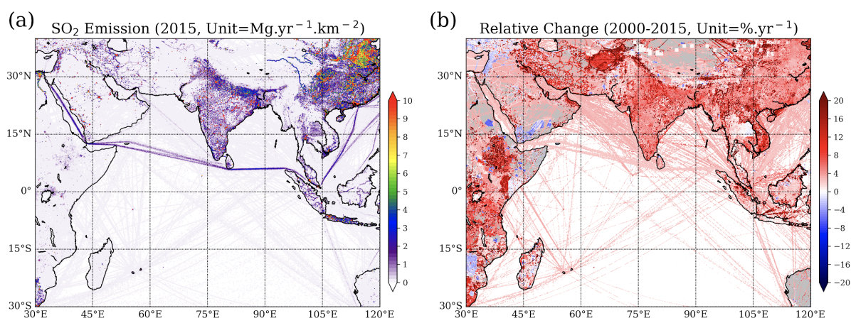
Figure 45. Same as Figure 23, but for SO 2 .
