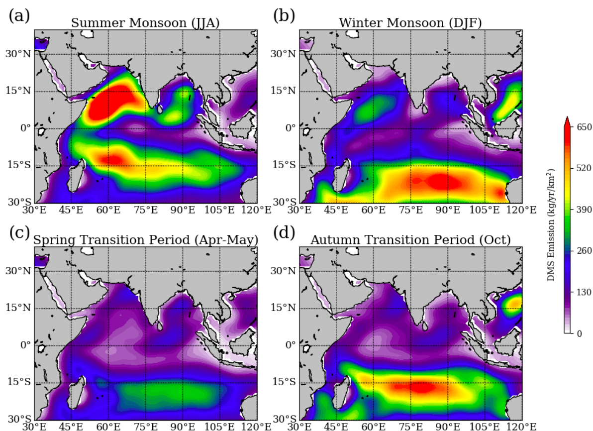
Figure 89. DMS emission for (a) summer monsoon (June – August), (b) winter monsoon (December – February), (c) spring transition (April – May) and (d) autumn transition (October) periods from Lana et al. (2011).
