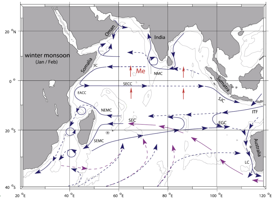
Figure 2. Schematic representation of identified oceanic currents during the summer monsoon (a) and winter monsoon (b). Current branches indicated are the South Equatorial Current (SEC), South Equatorial Countercurrent (SECC), Northeast and Southeast Madagascar Current (NEMC and SEMC), East African Coastal Current (EACC), Somali Current (SC), Southern Gyre (SG) and Great Whirl (GW) and associated upwelling wedges (green shades), Southwest and Northeast Monsoon Currents (SMC and NMC), South Java Current (SJC), East Gyral Current (EGC), and Leeuwin Current (LC). The subsurface return flow of the supergyre is shown in magenta. Depth contours shown are for 1000 m and 3000 m (grey). Updated representations are from SMC01; red vectors (Me) show directions of meridional Ekman transports. ITF indicates Indonesian Throughflow (from Schott et al., 2009, copyright 2009 by the American Geophysical Union, reproduced with permission).
