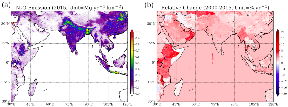
Figure 67. Same as Figure 56 but for N 2 O
