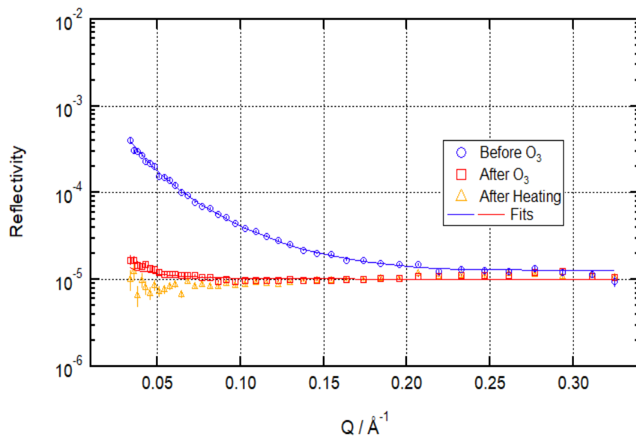
Figure S7: Reflectivity before ozonolysis (blue circles), after ozonolysis (red squares) and after heating (orange triangles) for ozonolysis of 17 \mu\text{L } 1.3 \text{ g L}^{-1} d_{34}\text{-OA} ( \text{CHCl}_3 spread. sol.) on pure water subphase by 323 \pm 29 \text{ ppb O}_3 added at t = 0 \text{ s} at 3 \pm 1 \text{ }^\circ\text{C} .
