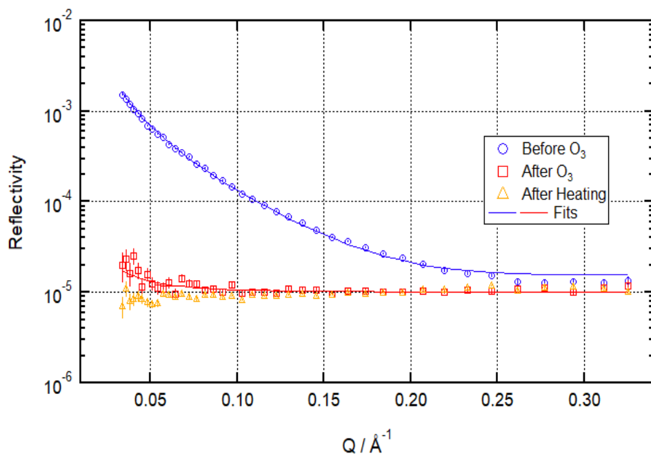
Figure S5: Reflectivity before ozonolysis (blue circles), after ozonolysis (red squares) and after heating (orange triangles) for ozonolysis of 25 \mu\text{L} 1.0 \text{g L}^{-1} d_{34}\text{-OA} ( \text{CHCl}_3 spread. sol.) on 36 \text{g L}^{-1} \text{NaCl(aq)} subphase by 323 \pm 29 ppb \text{O}_3 introduced at t = 0 s at -2 \pm 1 ^\circ\text{C} .
