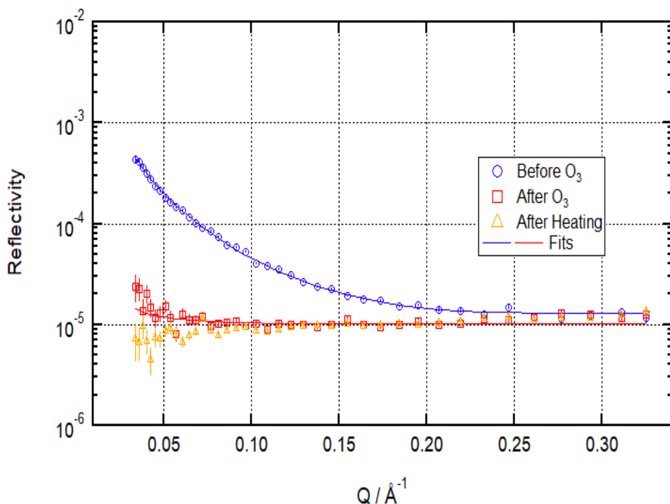
70 Figure S8: Reflectivity before O_3 (blue circles), after O_3 (red squares) and after heating (orange triangles) for ozonolysis of 17 \mu\text{L } 1.0 \text{ g L}^{-1} d_{34}\text{-OA} ( \text{CHCl}_3 spread. sol.) on 36 \text{ g L}^{-1} \text{NaCl(aq)} subphase by 323 \pm 29 \text{ ppb } O_3 added at t = 0 \text{ s} at 3 \pm 1 \text{ }^\circ\text{C} .
