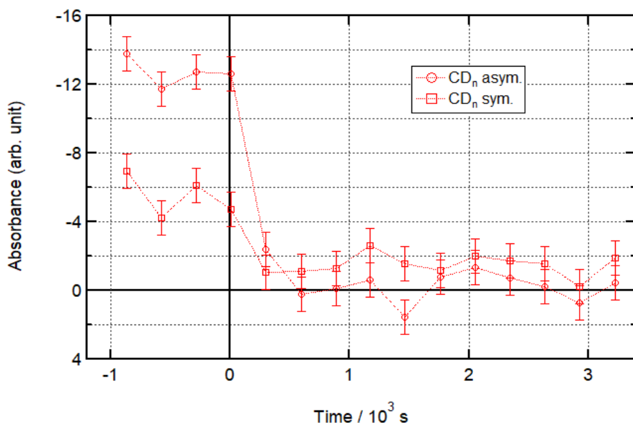
Figure S13: Time evolution plot for ozonolysis of 29 \mu\text{L} 1.0 \text{g L}^{-1} d_{34}\text{-OA} ( \text{CHCl}_3 spread. sol.) on pure subphase by 323 \pm 29 ppb \text{O}_3 introduced at t = 0 s at 21 \pm 1 ^\circ\text{C} showing integrated IR absorbance for \text{CD}_n asymmetric (circles) and symmetric (squares) bands.
