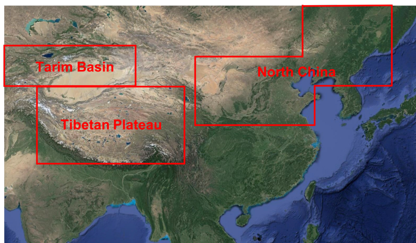
Figure 1. The selected three regions used in this study. The map was created by © Google Earth (version: © Google Earth Map 2020).
