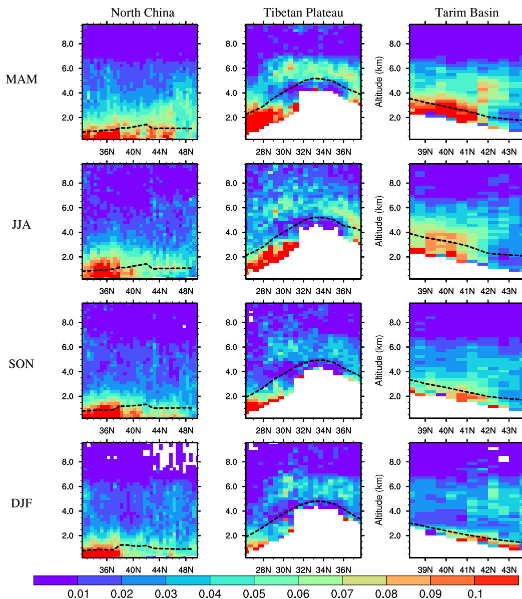
Figure 4. Vertical structure of 1064 nm aerosol extinction coefficients ( \text{km}^{-1} ) observed from CATS by season over the three regions in relation to zonal mean regional surface altitude. The dotted line represents the zonal mean regional planetary boundary layer (PBL).
