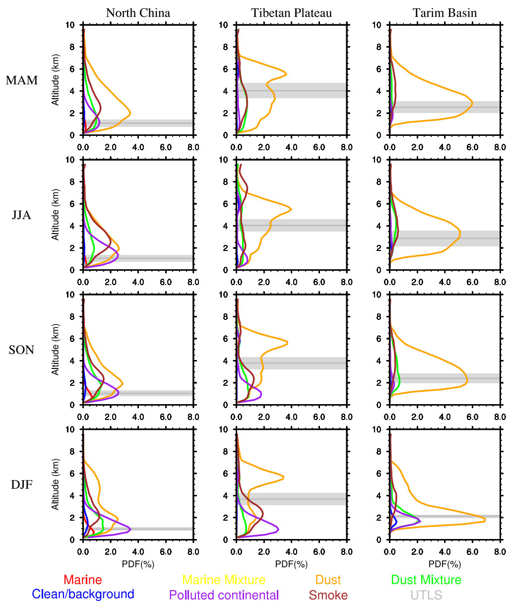
Figure 3. Probability distributions (frequency of occurrence) of the CATS-derived vertical aerosol subtypes by season over the three regions. The grey lines and fill areas correspond to the regional mean planetary boundary layer (km) and one standard deviation of the seasonal average, respectively.
