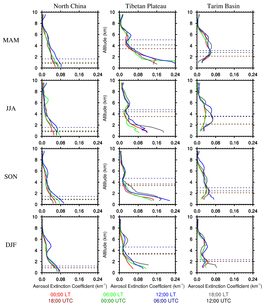
Figure 7. 6 h (00:00, 06:00, 12:00, 18:00 LT) vertical profiles of 1064 nm aerosol extinction coefficients ( \text{km}^{-1} ) observed from CATS by season over the three regions. The dashed lines represent the regional mean planetary boundary layer (PBL) by every 6 h (00:00, 06:00, 12:00, 18:00 UTC).
