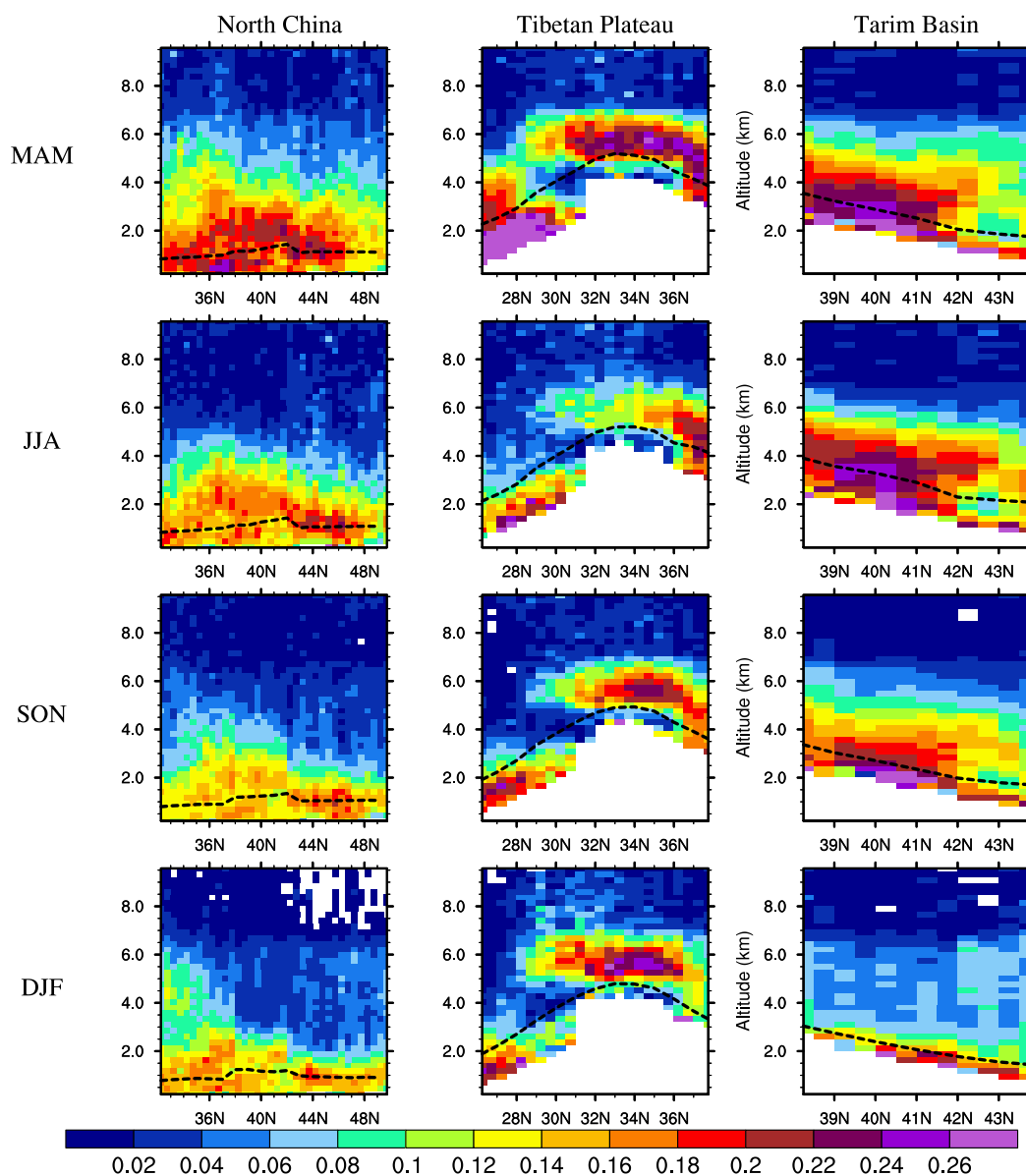
525 Figure 5. Vertical structure of total depolarization ratios observed from CATS by season over the three regions in relation to zonal mean regional surface altitude. The dotted line represents the zonal mean regional planetary boundary layer (PBL).
