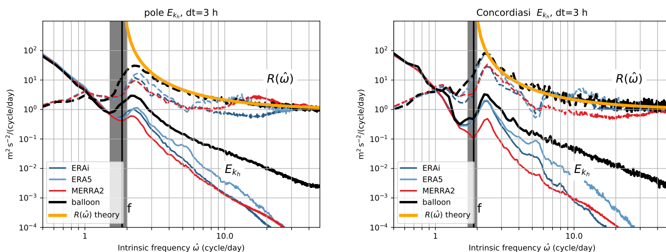
Figure 7. Intrinsic frequency spectra of horizontal kinetic energy per unit mass E_{k_h} during the Vorcore (austral winter 2005, left) and Concordiasi (austral winter 2010, right) campaigns. The black curve corresponds to balloon observations during the campaigns while the spectra estimated from isopycnic trajectories in different (re)analyses are in colors. The vertical black line indicates the mean Coriolis parameter f while the shaded grey area represents its variability along the balloon trajectories.
