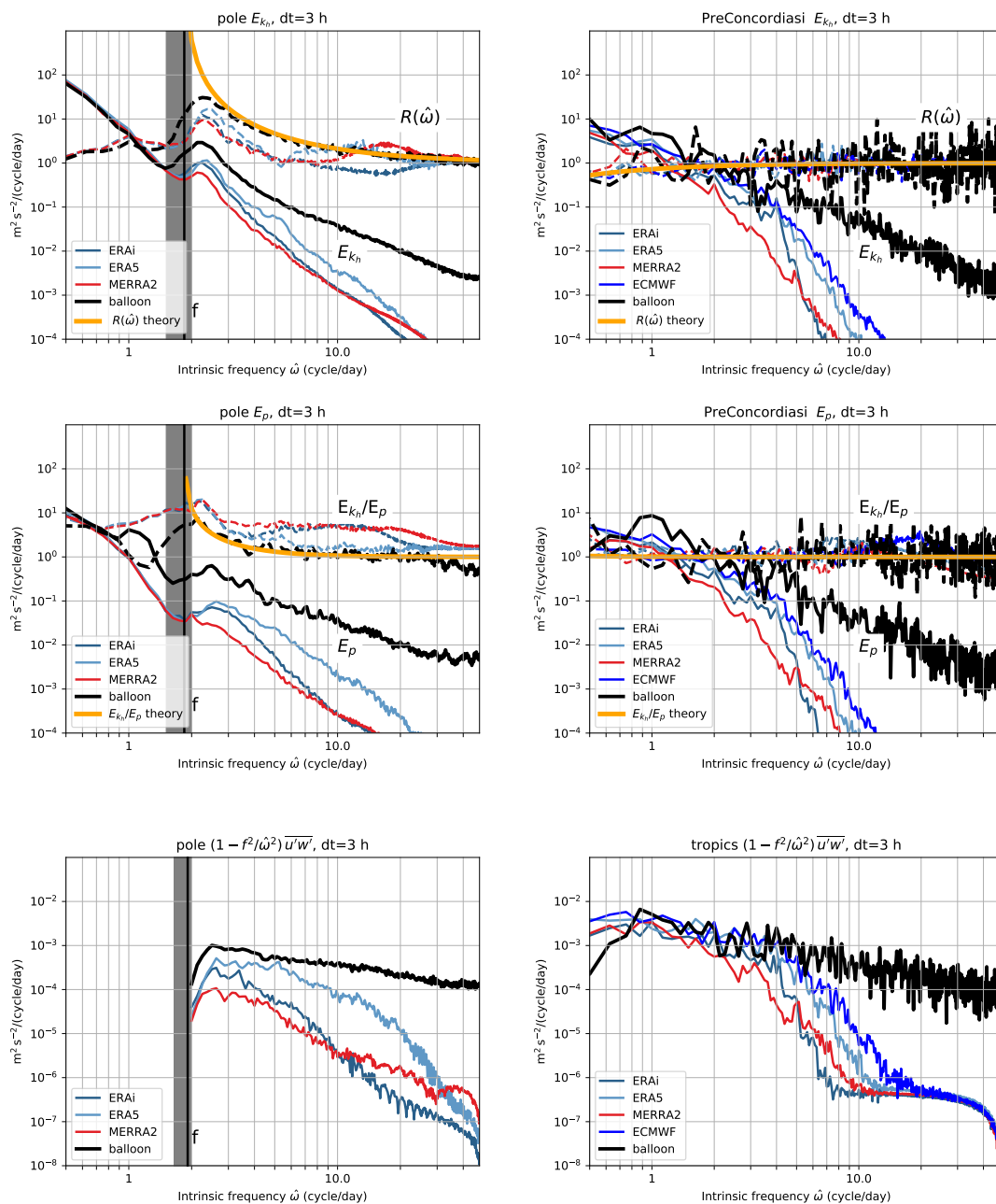
Figure 3. Intrinsic frequency spectra of (top) horizontal kinetic energy per unit mass E_{kh} (solid) and rotary ratio R(\hat{\omega}) (dashed), (middle) potential energy per unit mass E_p and ratio of kinetic over potential energy E_{kh}/E_p , and (bottom) zonal pseudo-momentum flux per unit mass (1 - f^2/\hat{\omega}^2) \overline{u'w'} during the polar Vorcore campaign (left column) and the equatorial PreConcordiasi (right column) campaign. The black curve on each plot corresponds to balloon observations while the spectra estimated from isopycnic trajectories in different (re)analyses are in colors. The trajectories used to compute the spectra are 8-days trajectories started at the balloon position.
