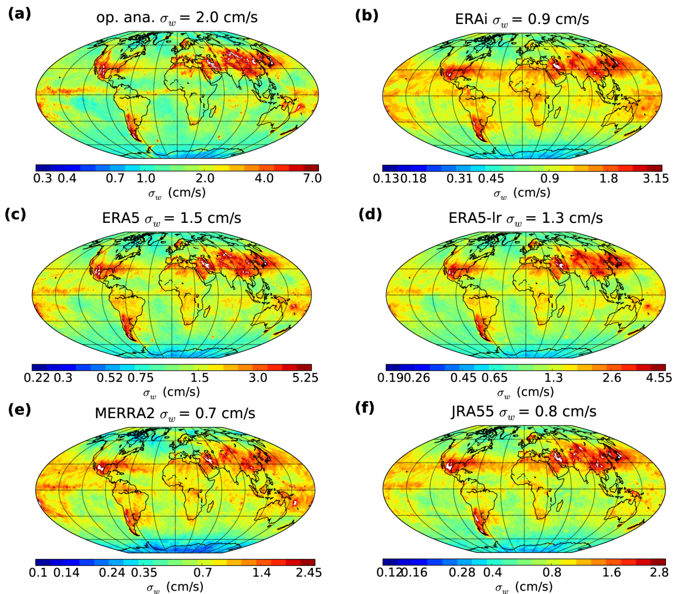
Figure 5. Global maps of vertical velocity standard deviation \sigma_w at 100 hPa in different reanalyses systems during March 2010. Note that the color scales have been adjusted so that the ratio between local and global \sigma_w corresponds to the same color in all panels. ERA5-lr is a retrieval from ERA5 reanalysis truncated at the same resolution as the ERA-Interim (T255).
