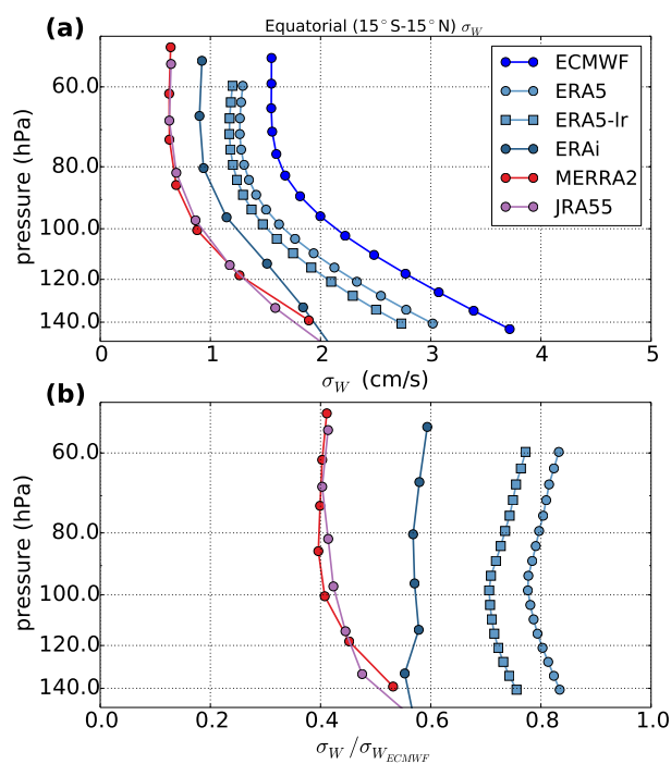
Figure 6. (Top) Equatorial ( 15^{\circ}\text{S} - 15^{\circ}\text{N} ) average profile of vertical velocity variance in different reanalyses systems for March 2010. Bottom: the same, but normalized by the profile from the 2010 ECMWF operational analysis. ERA5-Ir is a retrieval from ERA5 reanalysis truncated at the same resolution as the ERA-Interim (T255). The position of the dots corresponds to the model vertical levels, and emphasize the better resolution of ERA5 in the Tropical Tropopause Layer compared to earlier products.
