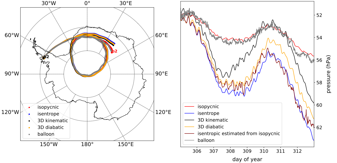
Figure 2. (Left) Observed and calculated horizontal trajectories of Vorcore Balloon 2 started from its position on 2005/11/02 at 00:00 UTC. The calculated trajectories are 3D-kinematic (with omega velocity, black), 3D-diabatic (with diabatic heating rates, orange), 2D-isentropic (blue) and 2D-isopycnic (red) trajectories; all were computed using ERA5 wind and temperature field at 3-hourly output resolution. The observed trajectory of the balloon is shown in grey. (Right) Pressure time series corresponding to the horizontal trajectories on the left panel. Please note that the y-scale only covers a narrow range of altitudes (roughly 1 km maximum deviation peak-to-peak, i.e. about 3 model levels for ERA5).
