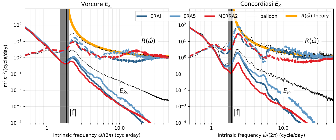
Figure 7. Intrinsic frequency spectra of horizontal kinetic energy per unit mass E_{kh} during the Vorcore (austral winter 2005, left) and Concordiasi (austral winter 2010, right) campaigns. The black curve corresponds to balloon observations during the campaigns while the spectra estimated from isopycnic trajectories in different (re)analyses are in colors. The vertical black line indicates the mean Coriolis parameter |f| while the shaded grey area represents-depicts its variability along the balloon trajectories.
