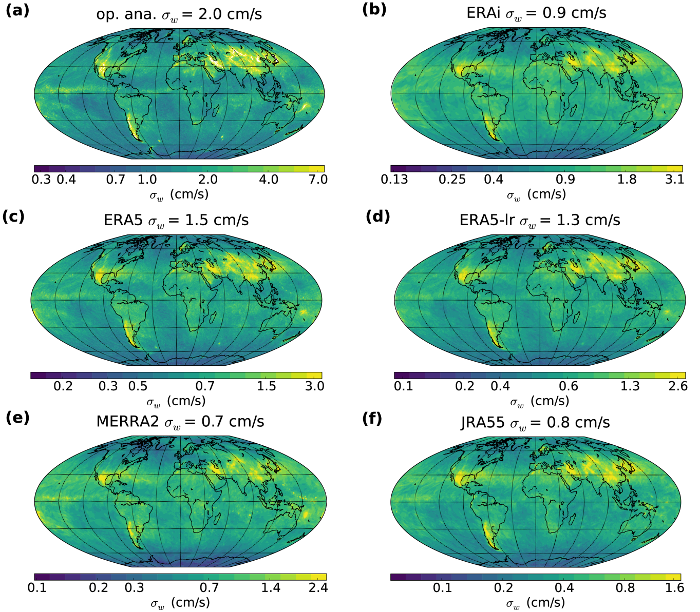
Figure 5. Global maps of vertical velocity standard deviation \sigma_w at 100 hPa in different reanalyses systems during March 2010. ERA5-lr is a retrieval from ERA5 reanalysis truncated at the same resolution as the ERA-Interim (T255). Note that the color scales are logarithmic and that they have been adjusted so that the ratio between local and global \sigma_w corresponds to the same color in all panels. ERA5-lr is a retrieval from ERA5 reanalysis truncated at This normalization emphasizes the same-resolution-as-spatial pattern, regardless of the ERA-Interim (T255) average value.
