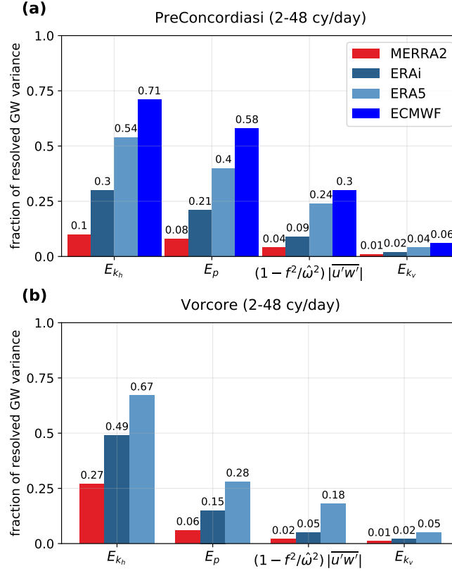
Figure 8. Bar chart of the fraction of resolved variance in the reanalyses reanalysis balloon trajectories in the 2-48 cy/day frequency range, i.e. variance in the reanalysis trajectories normalized by the variance present in balloon observations. Results are shown for the (a) tropical 2010 PreConcordiasi campaign and the (b) 2005 polar latitudes' Vorcore. The fields considered are, from left to right: horizontal kinetic energy E_{kh} , potential energy E_p , zonal pseudo-momentum flux (1 - f^2 / \hat{\omega}^2) |u'w'| and vertical kinetic energy E_{kv} .
