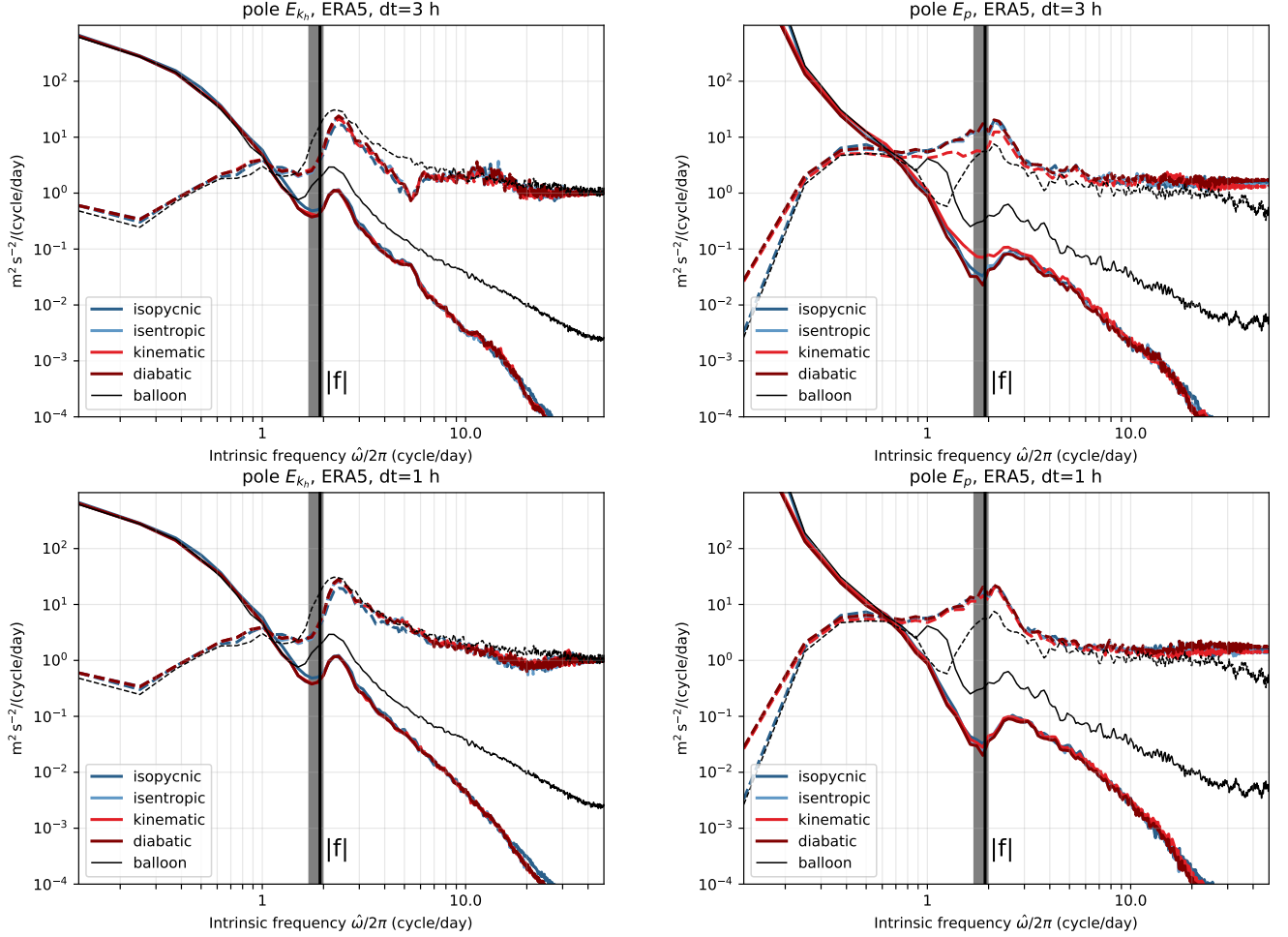
Figure B1. Intrinsic-frequency spectrum of (left) kinetic energy E_k and (right) potential energy E_p per unit mass along ERA5 trajectories started at Vorcore balloon locations, for different trajectory types: isopycnic (constant \rho ; note that E_p spectrum is in that case adjusted following Eq. 3, as is done for the balloons), isentropic (constant \theta ) and kinematic and different reanalysis output frequencies (top: 3 hours; bottom: 1 hour).
