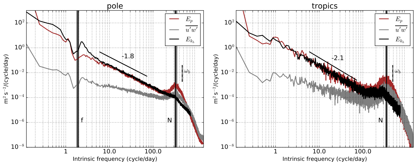
Figure 1. Average spectra of horizontal kinetic energy E_{kh} , potential energy E_p and \overline{u'w'} inferred from SPB observations during the (left) polar and (right) equatorial balloon campaigns in 2010.
