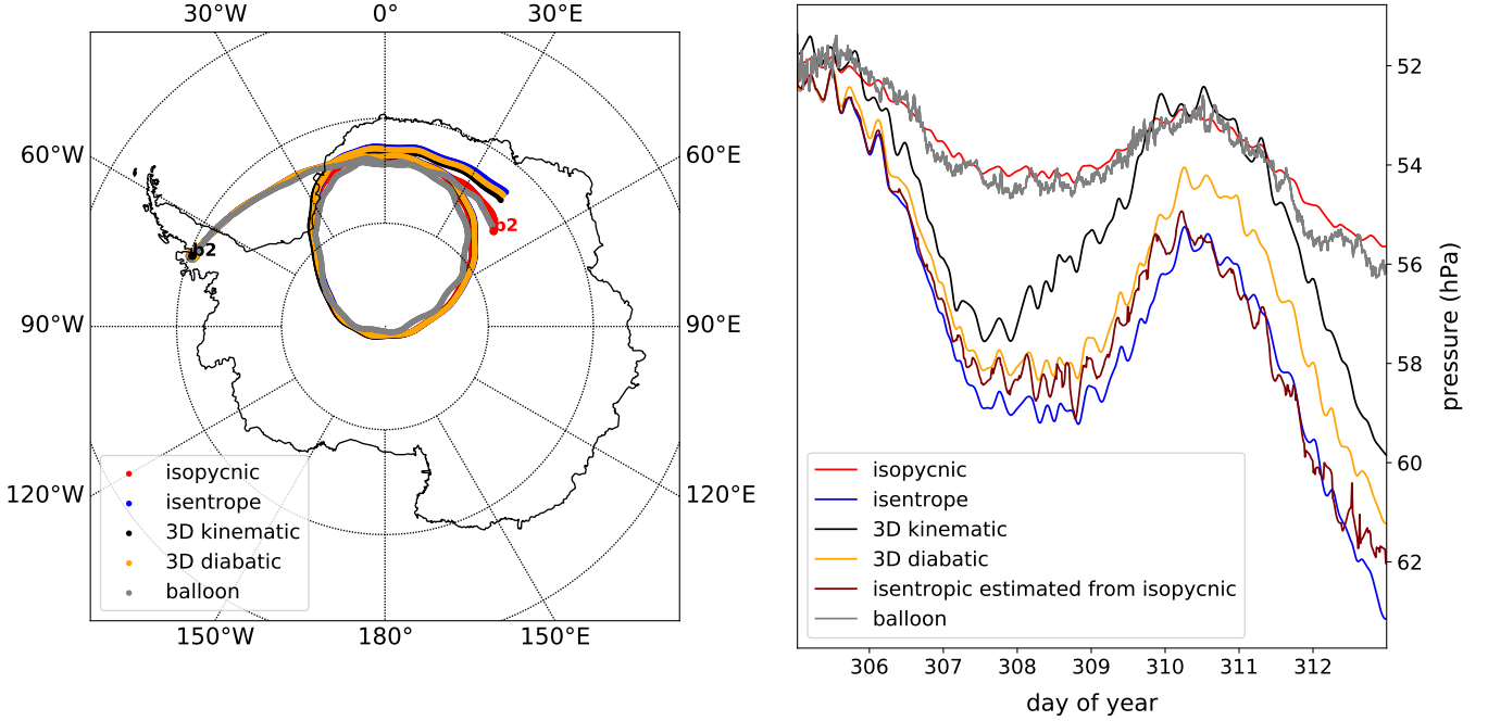
Figure 2. (Left) Observed and calculated horizontal trajectories of Vorcore Balloon 2 started from its position on 2005/11/02 at 00:00 UTC. The calculated trajectories are 3D-kinematic (with omega velocity, black), 3D-diabatic (with diabatic heating rates, orange), 2D-isentropic (blue) and 2D-isopycnic (red) trajectories; all were computed using ERA5 wind and temperature field at 3-hourly output resolution. The observed trajectory of the balloon is shown in grey. (Right) Pressure time series corresponding to the horizontal trajectories on the left panel. Please note that the y-scale only covers a narrow range of altitudes (roughly 1 km maximum deviation peak-to-peak, i.e. about 3 model levels for ERA5).
