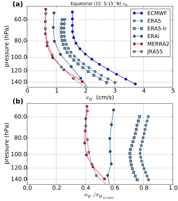
Figure 6. (Top) Equatorial (15°S-15°N) average profile of vertical velocity variance in different reanalyses systems for March 2010. Bottom: the same, but normalized by the profile from the 2010 ECMWF operational analysis. ERA5-Ir is a retrieval from ERA5 reanalysis truncated at the same resolution as the ERA-Interim (T255). The position of the dots corresponds to the model vertical levels, and emphasize the better resolution of ERA5 in the Tropical Tropopause Layer compared to earlier products.
