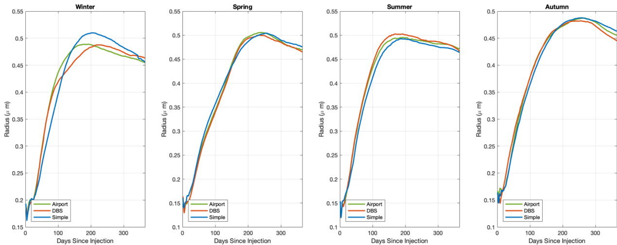
440 Figure 12: Mass-averaged effective radius of injected \text{SO}_4 aerosols on the 540 K isentrope spanning one year of CESM2(WACCM6) simulations after injection.
